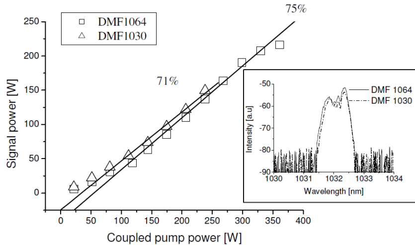
Fig. 3. Slope efficiency measurement of the DMF1030 and the DMF1064 and recorded output spectra at the maximum output powers.
