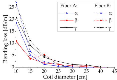
Fig. 4. Bending loss in transmission band \alpha , \beta , and \gamma as a function of coil diameter. The largest coil diameter is used as a reference of zero bending loss.
