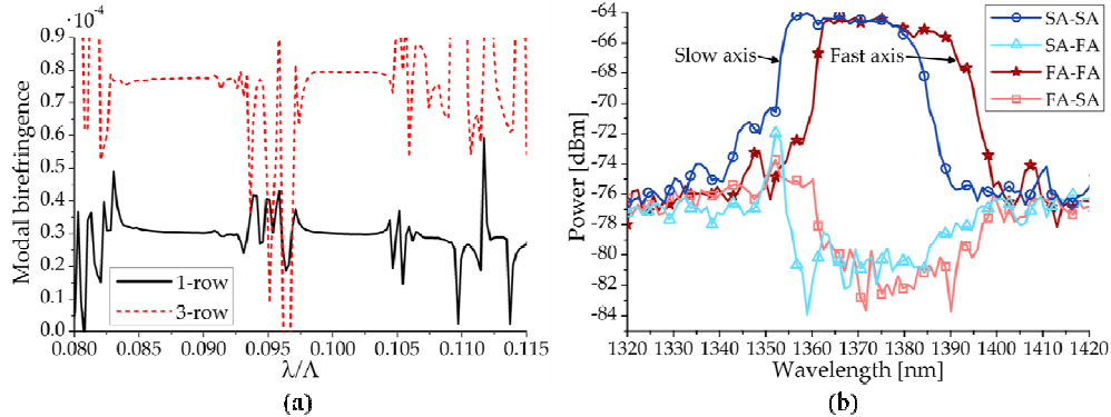
Fig. 9. (a) Calculated modal birefringence in the 1- and 3-row design. The modal birefringence is increased with a factor of \sim 2.7 in the 3-row design. (b) Polarization properties of transmission band \gamma .
