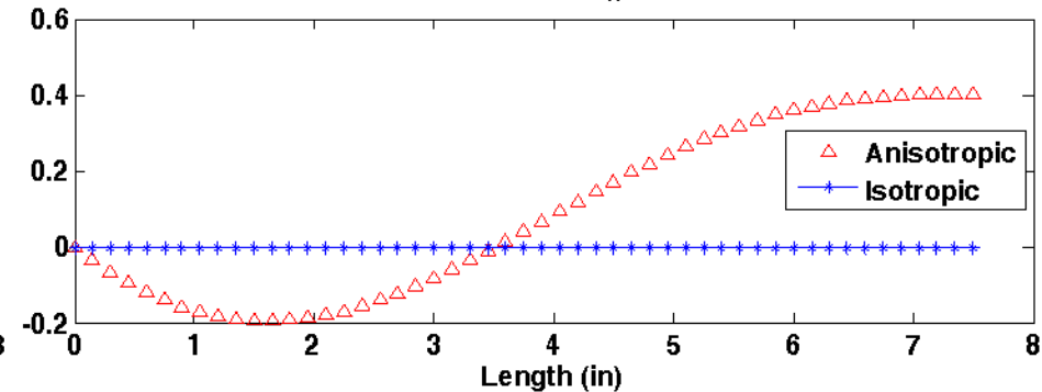
Torsion ( \theta_x )
