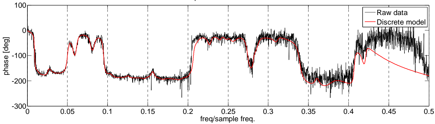
Phase of displacement/force transfer function
