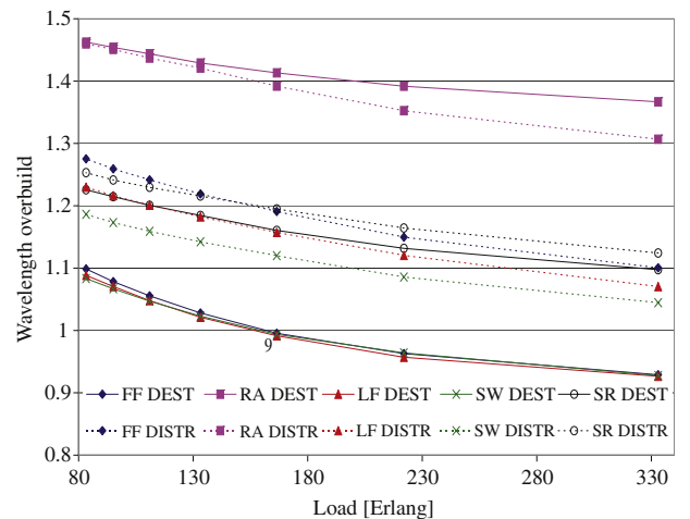
Fig. 8. (Color online) Wavelength overbuild versus load.
