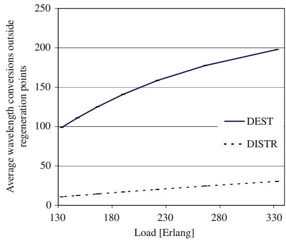
(d) Average wavelength conversions outside of regeneration points.
