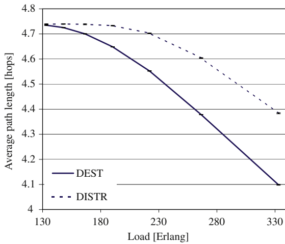
(c) Average path length.
