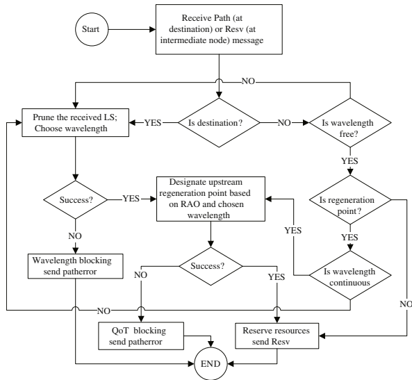
Fig. 2. Flow-chart for the DISTR scheme.
