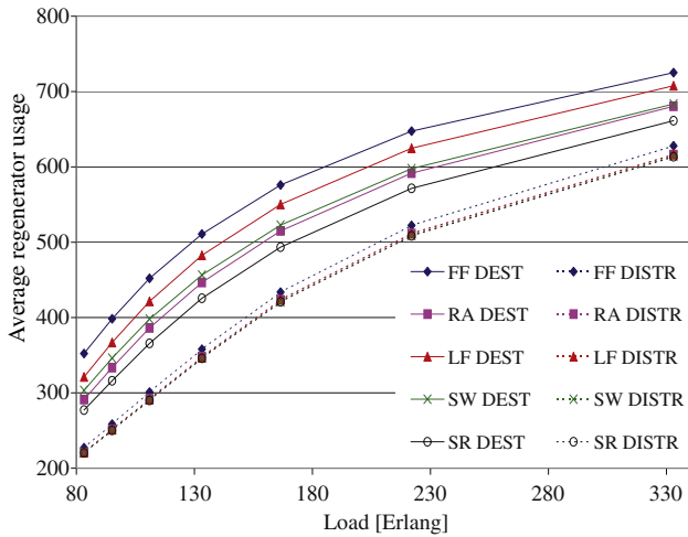
Fig. 6. (Color online) Average regenerator usage versus load.
