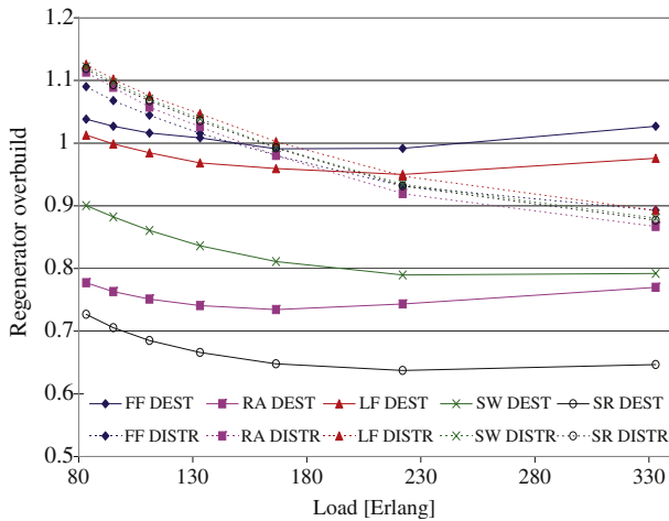
Fig. 9. (Color online) Regenerator overbuild versus load.
