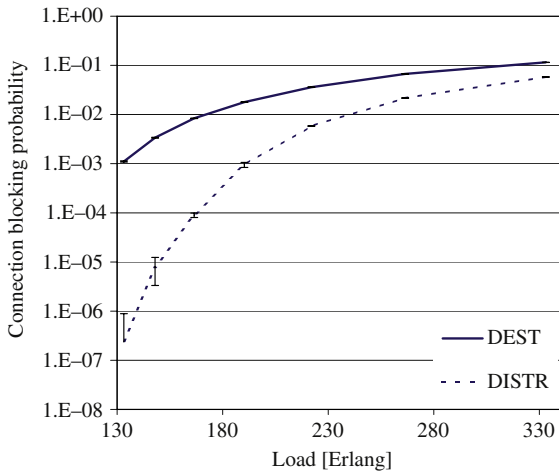
(a) LSP blocking probability.
