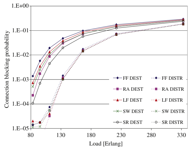
Fig. 5. (Color online) Total LSP blocking probability versus load.
