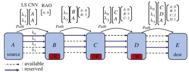
Fig. 1. (Color online) Example of CNV usage.
