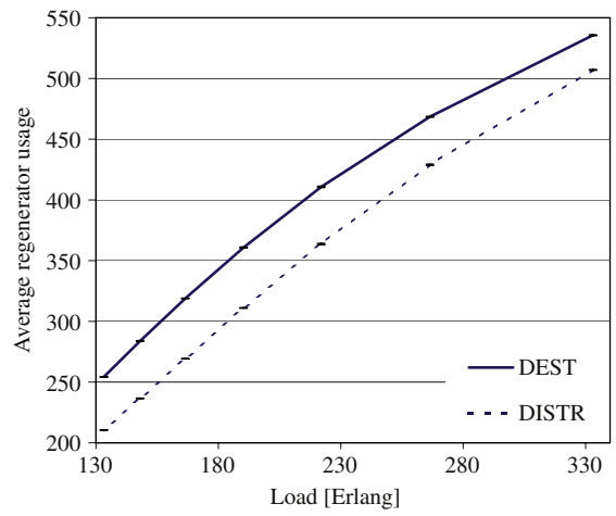
(b) Regenerator usage.
