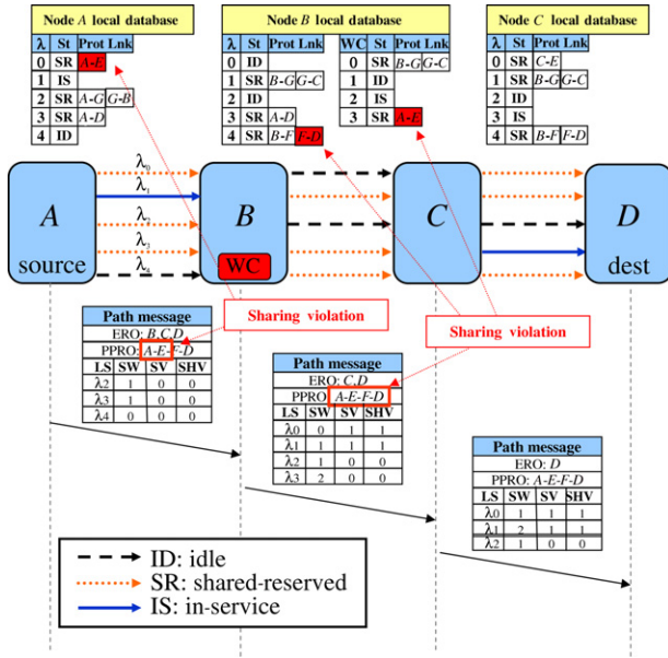
Fig. 3. (Color online) RSVP-TE operations for the protection LSP.
