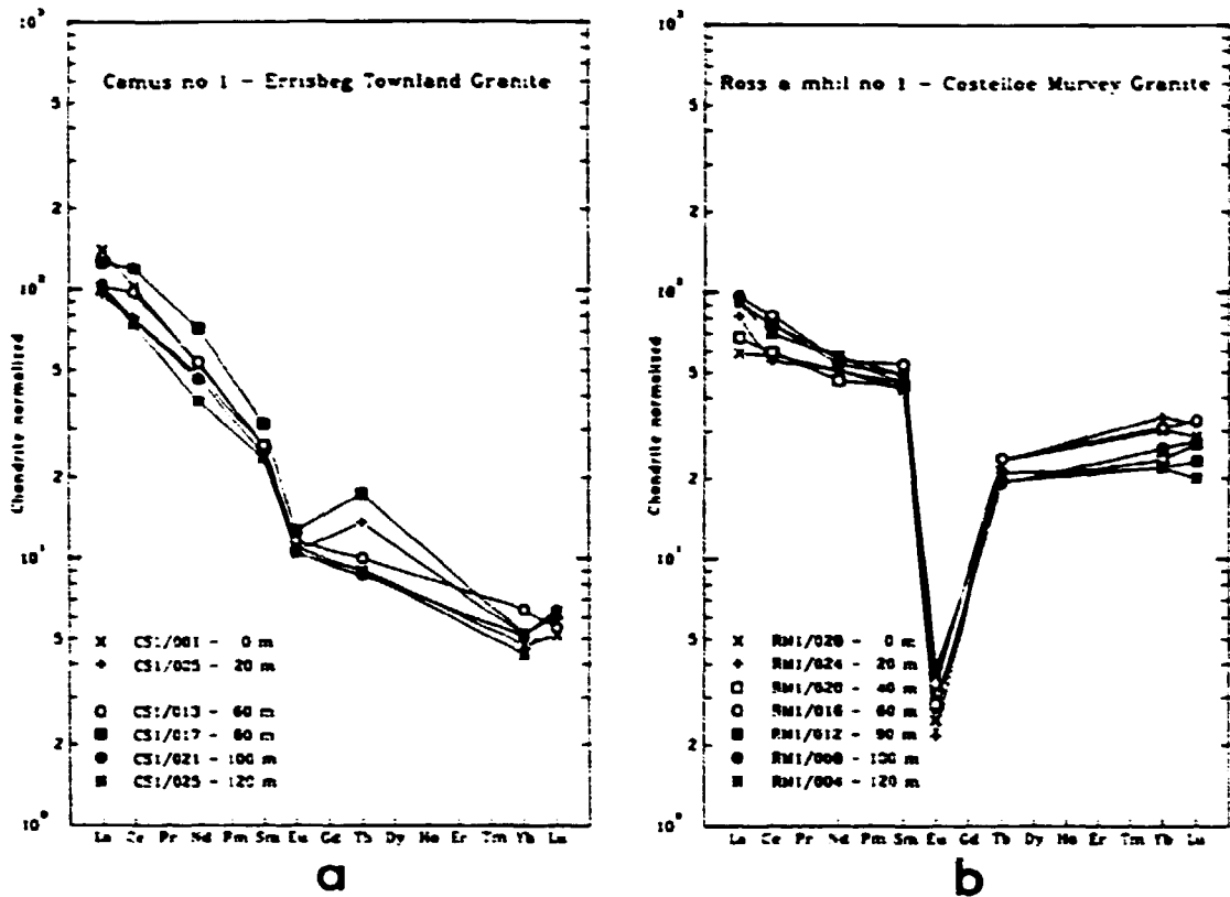
Fig. 5.2.1. Chondrite-normalised REE profiles for drill core samples of Irish granites. a = bore hole Camus no. 1, b = borehole Ros a Mhil, both from the Galway area.
