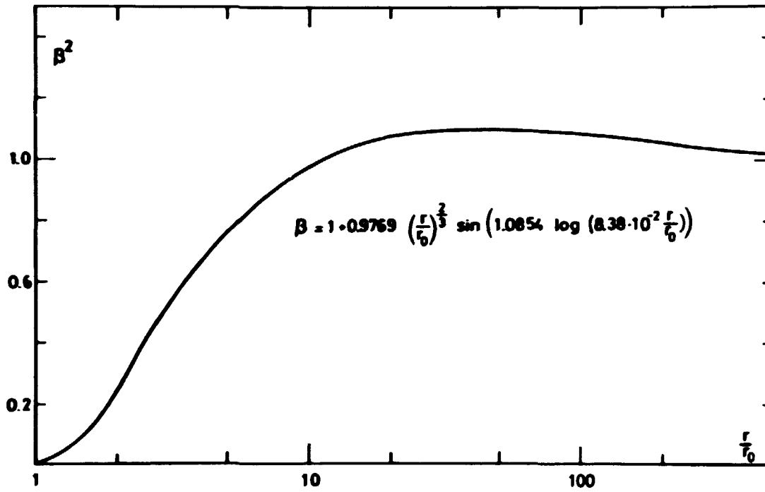
Fig. 18. Geometry factor B^2 as a function of cathode radius to emitting plasma radius r/r_0 .
