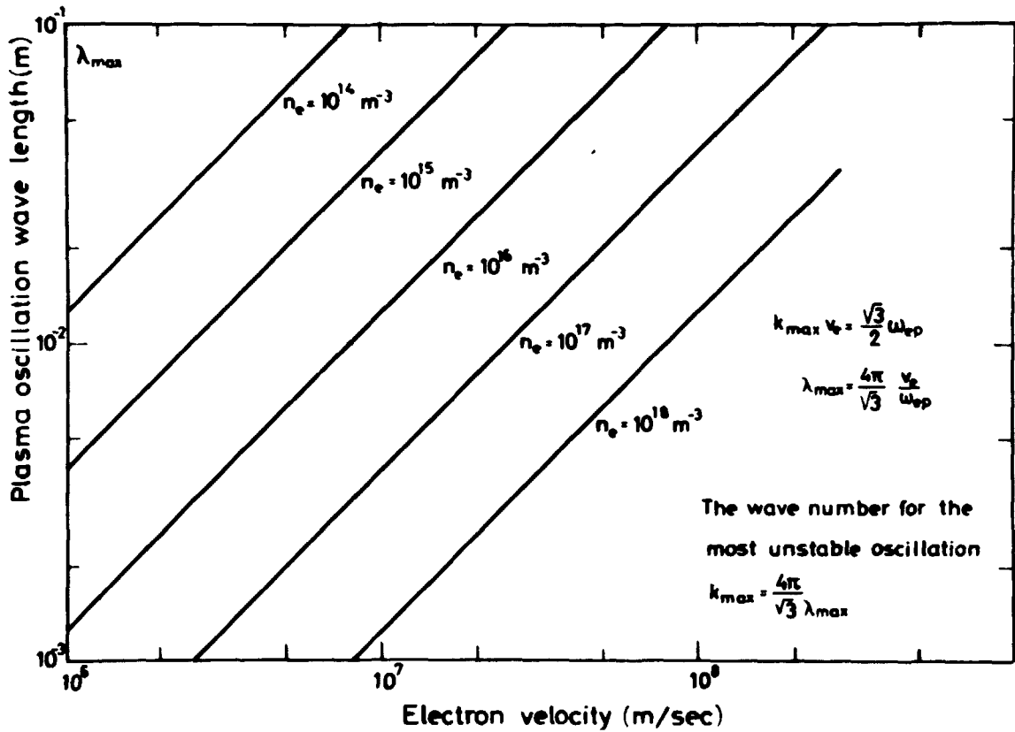
Fig. 22. Plasma oscillation wavelength for the most unstable oscillation as a function of the root mean square thermal velocity of the plasma electrons.
