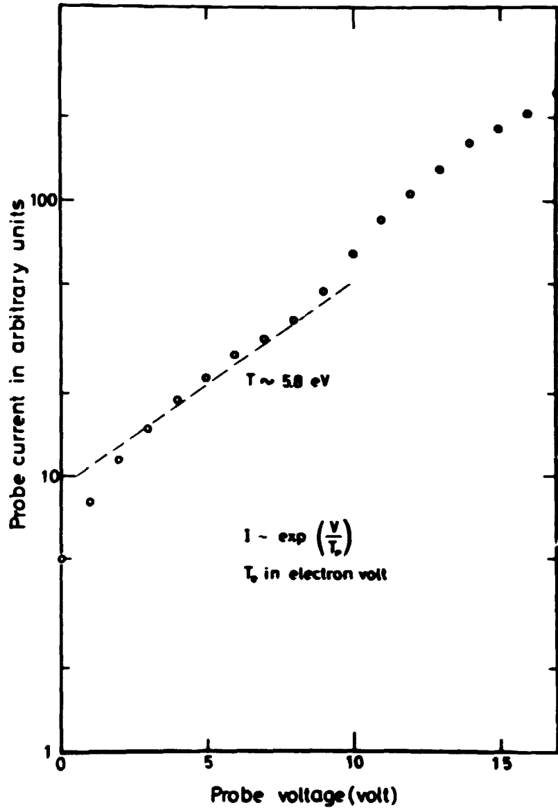
Fig. 19. Electron temperature determined from current-voltage characteristic of a Langmuir probe of area A = 3 \cdot 10^{-7} \text{ m}^2 .
