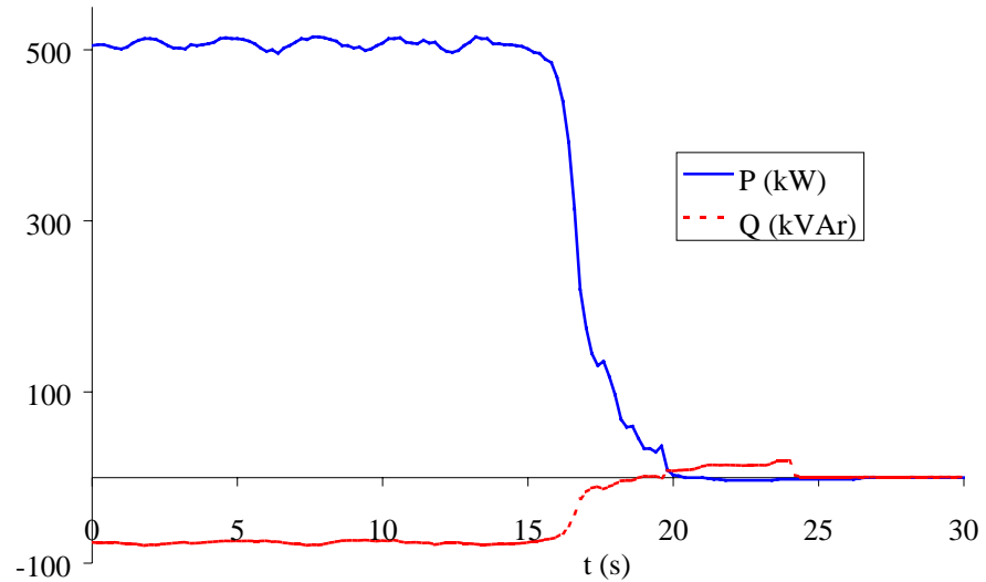
Figure 66. Active and reactive power during stop of an Enercon E-40 in high wind conditions. The upper (positive) curve is the active power and the lower (negative) curve is the reactive power.
