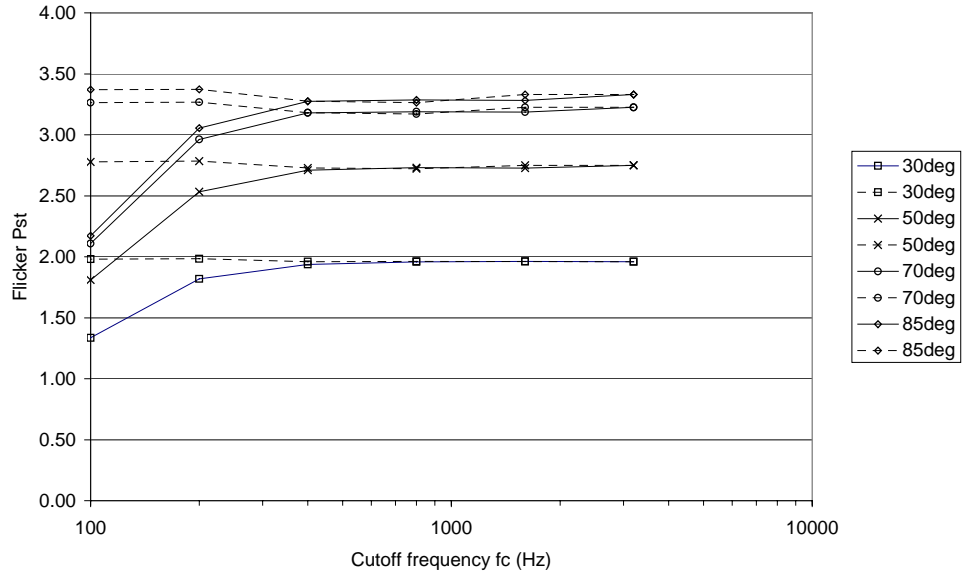
Figure 38. Flicker Pst values for the 6.4kHz DEWI measurement of cut-in operation filtered with the cut-off frequency f_c . The dashed lines keep the original sampling frequency 6.4kHz, and the solid lines the data is reduced to the sampling frequency 2 \cdot f_c .
