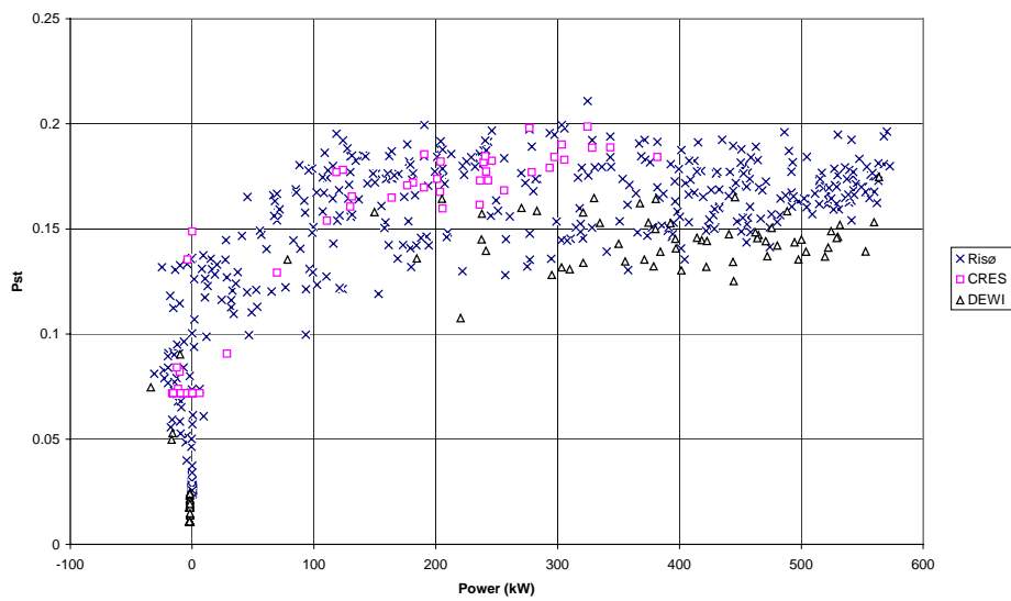
Figure 17. 5 minutes Pst values with grid angle 50 deg and short circuit ratio 20 vs. mean value of power.
