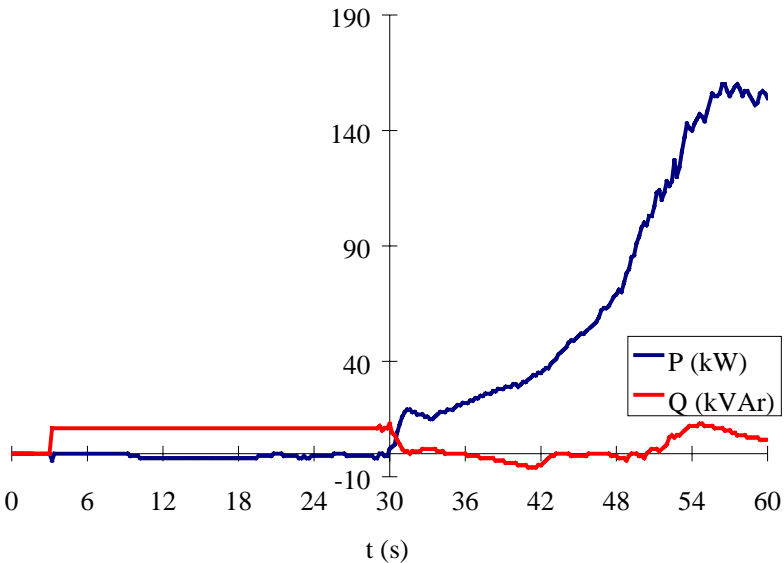
Figure 65. Active and reactive power during start of the Enercon E-40 located in Skåne. The upper (positive) curve is the active power and the lower (negative) curve is the reactive power.
