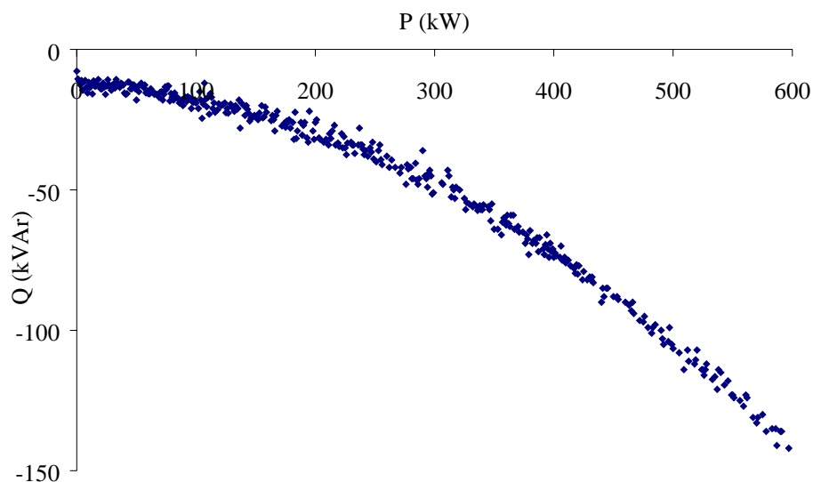
Figure 54. Measured reactive power as a function of active power from fixed-speed Wind World 600 kW wind turbine.
