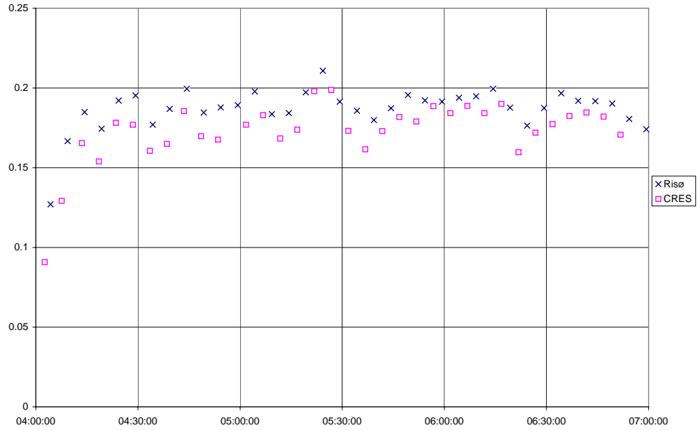
Figure 22. Time series of 5 minutes P_{st} values with grid angle 50 deg and short circuit ratio 20. The measurements were taken 16 October 1997.
