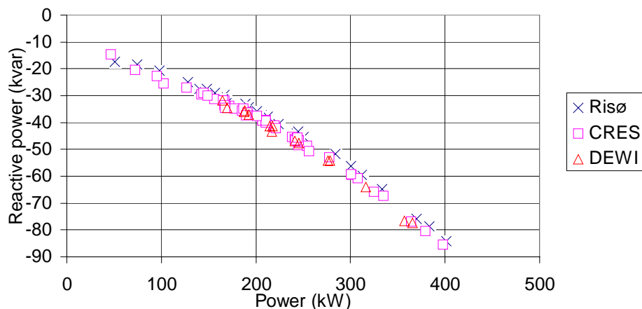
Figure 7. 1 min. mean values of reactive power vs. active power measured 16. October 1997 between 14:00 and 15:00
