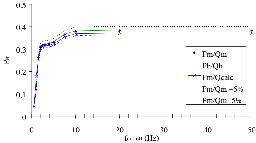
Figure 55. Short term flicker emission P_{st} from a fixed-speed stall-regulated Wind World 600 kW wind turbine calculated at different cut-off frequencies of the measured and calculated active and reactive power.
