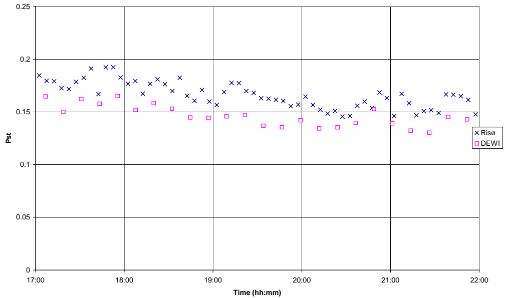
Figure 23. Time series of 5 minutes P_{st} values with grid angle 50 deg and short circuit ratio 20. The measurements were taken 16 October 1997.
