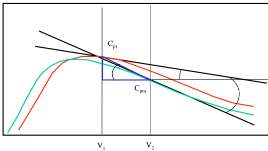
Fig. 6.1. Power and C_p curves for variable pitch with fixed rotor speed
