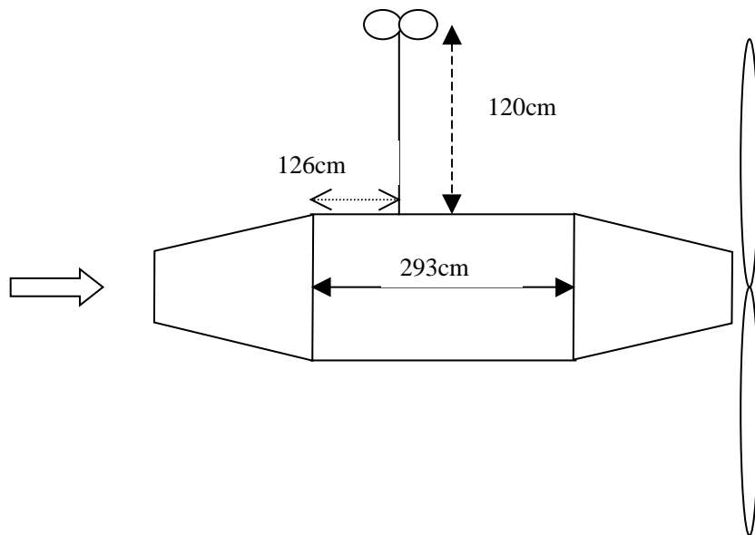
Fig 2.20. Placement of the anemometer on the nacelle
