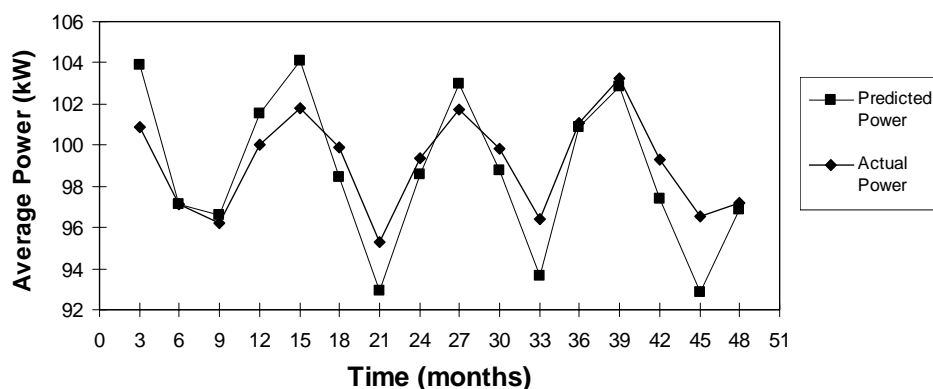
Fig. 7.1. Reduction in uncertainty possible with multi-variate analysis compared with the fixed level associated with conventional performance assessment
