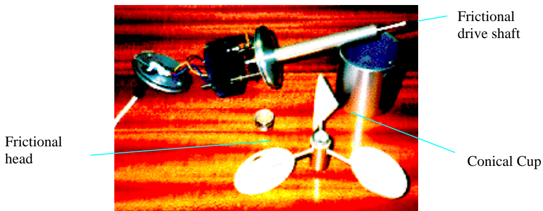
Fig. 4.1. Vector A100 cup anemometer
