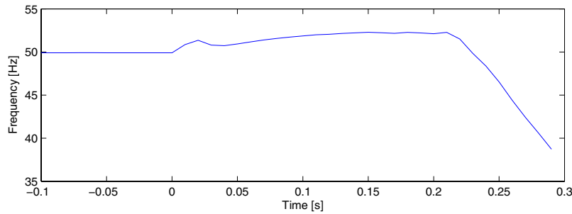
Figure 65: Frequency of the voltage U_{10\text{wt}2} measured at the 10 kV connection point of wind turbine #2.
