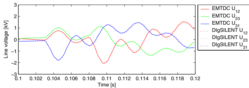
Figure 18: Simulated generator voltages with EMTDC and DIgSILENT in first line period after the shout circuit is cleared.
