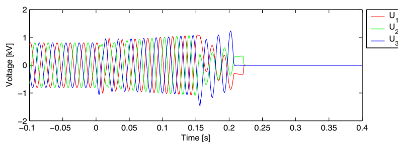
Figure 75: Simulated line to neutral voltages U_{LV} at the 960 V bus of wind turbine #1.
