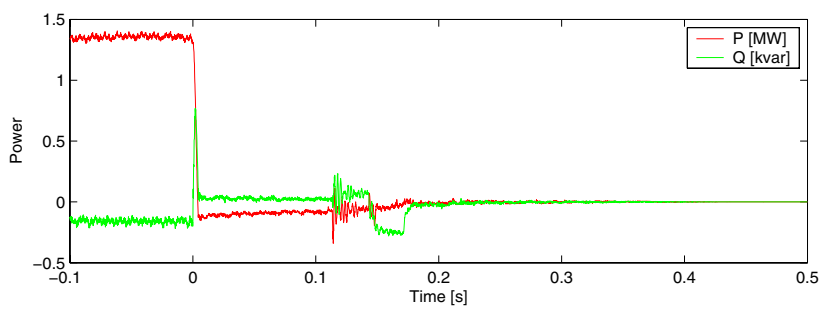
Figure 61: Active power P_{10wt2} and reactive power Q_{10wt2} measured at the 10 kV connection point of wind turbine #2.
