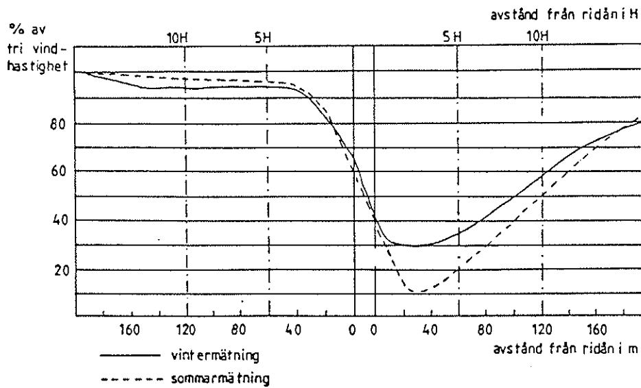
Figur 8.2. Vindprofiler, Vålaholm (efter Nord, 1986) (ref. 4)
