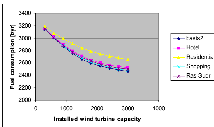
Figure 8 Fuel consumption of systems with 3% annual load increase
