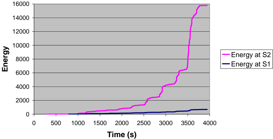
Figure 32 Cumulative stress wave energy trace showing the relative activities at S2 (loading yoke) and S1 (close to desired failure chord). Note also the rapid increase in stress wave activity at S2 indicating that failure is approaching.
