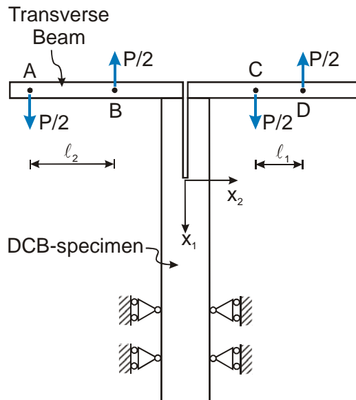
Figure 7. Schematics of the proposed loading method; the mode mixity is controlled entirely by altering the length of one of the transverse beam arms, e.g. l_1 . [Mixed_Mode_loading_1c.cdr]
