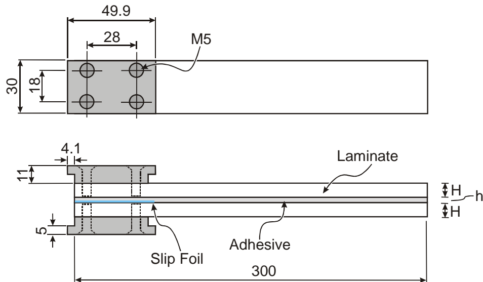
Figure 9. Sketch of the specimen geometry. Steel parts are attached to the laminates by screws and adhesive. Nominal dimensions: H = 8 mm, h = 3 mm and B = 30 mm. [Mixed_mode_specimens_dimensions_1b.cdr]
