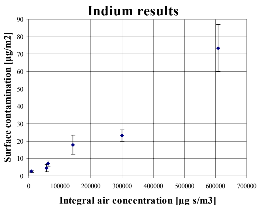
Figure 2.6 Surface contamination plotted versus the integrated air concentration in 6 different tests. The error bars shows the standard deviation on the mean for each test.
