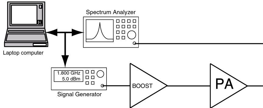
Figure 7.8 Measuring ACPR for digital predistortion system.
