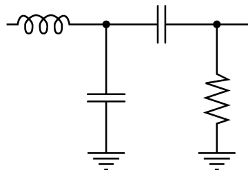
Figure 3.11 Load-pull impedance realized as a matching network.
