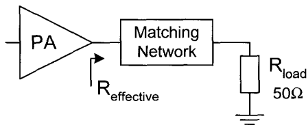
Fig. 1. Power amplifier and load
