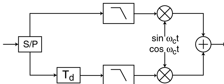
Figure 7.6 Block diagram of digital OQPSK modulation.
