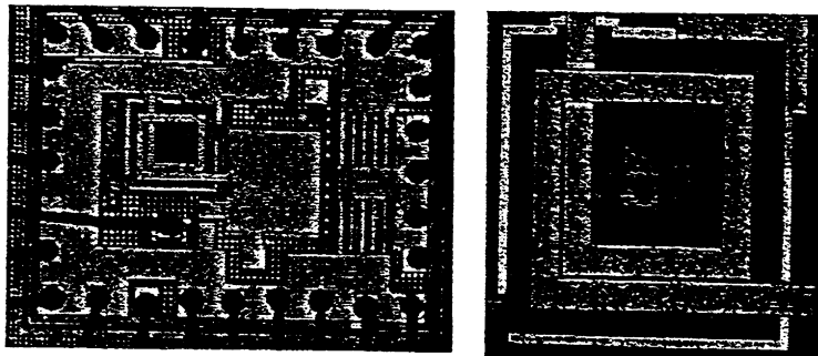
Figure 7. Photo of entire chip and of the inductor
