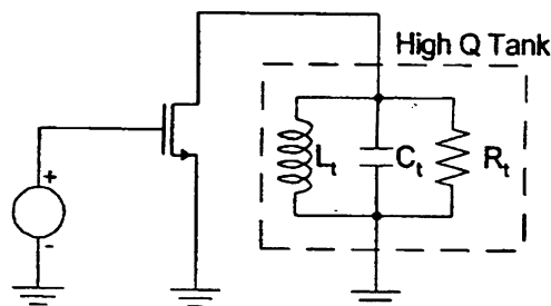
Figure 2. Determination of effective transistor load using a high Q tank.
