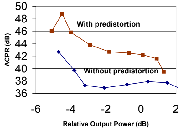
Figure 4: ACPR with or without predistortion vs. output power
