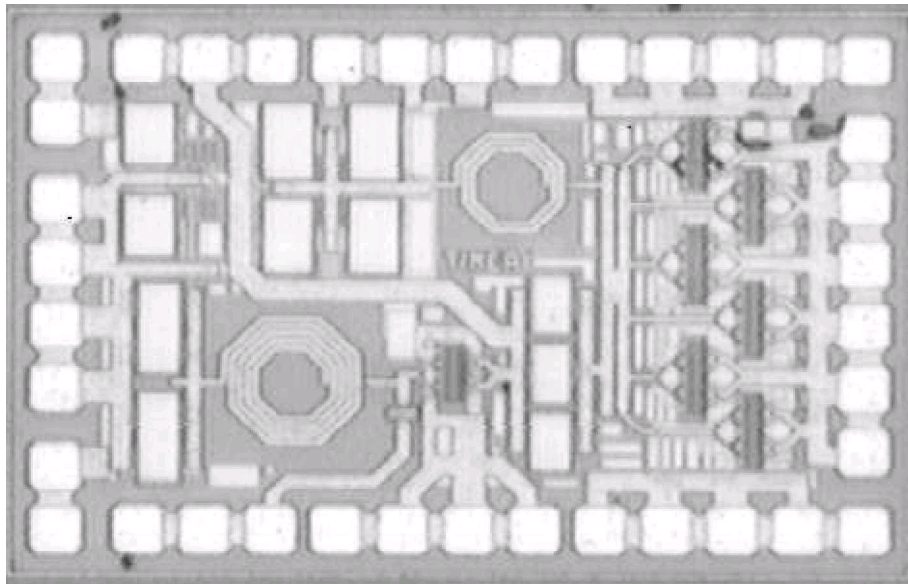
Figure 8.15 Die photograph.
