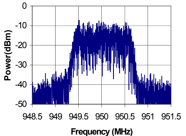
Figure 6: Spectrum with predistortion
