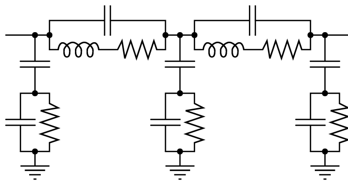
Figure 5.5 On-chip inductor model.
