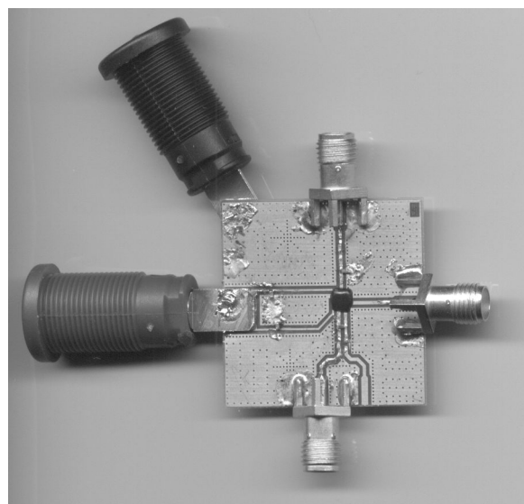
Fig 4. PCB photograph.
