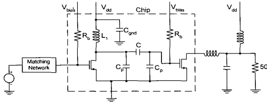
Fig. 4. PA circuit
