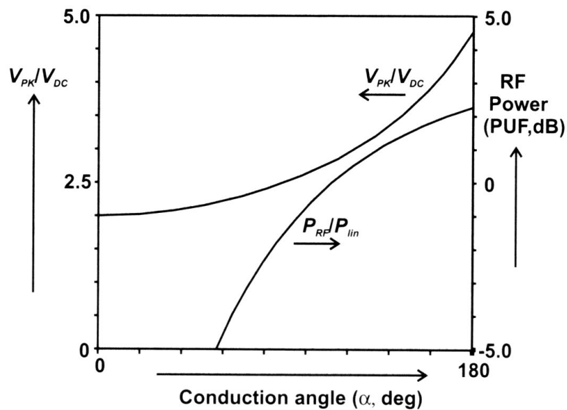
Figure 2.13 Output power and peak voltage vs. conduction angle [1].
