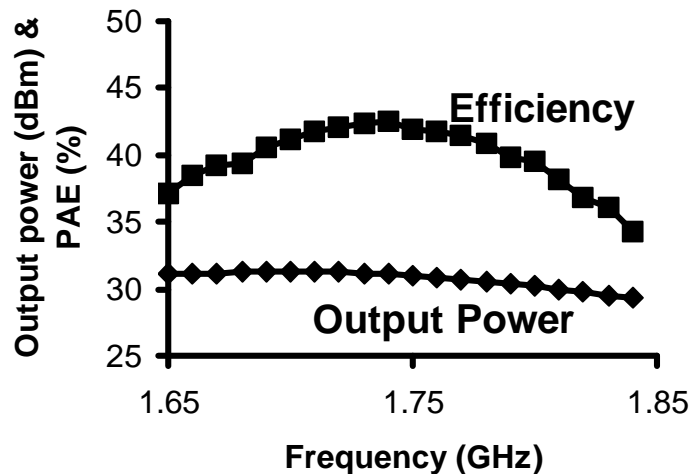
Figure 8.10 Output power and efficiency vs. frequency, biased for maximum output power
