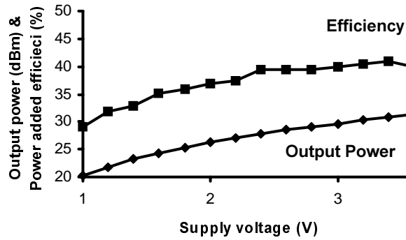
Figure 5 Measured output power and efficiency vs. supply voltage at 1730 MHz.
