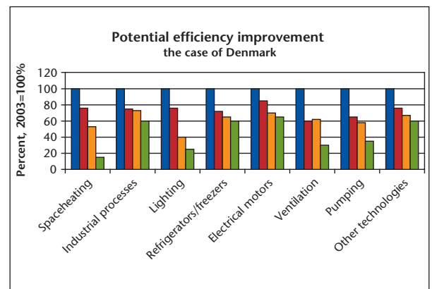
Figure 15: The potential for improving end-use energy efficiency in Denmark. Column 1 (100%) shows consumption today; Column 2 shows socio-economic investments that are profitable up to 2015. Column 3 shows private investments that are profitable, assuming the present pattern of energy tax, up to 2015. Column 4 is a conservative estimate of technically-possible efficiency improvements (not theoretical limits). [20]
