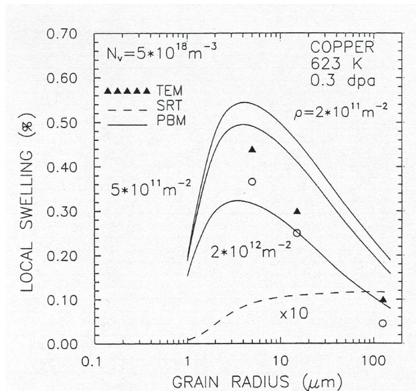
Figure 28. The calculated (full lines) and experimentally measured ( \blacktriangle ) grain size dependence of the local void swelling in the grain interiors of copper irradiated at 350°C to 0.3 dpa. The open circles (O) are the swelling values calculated for specific grain sizes using the experimental values of void and dislocation densities.
