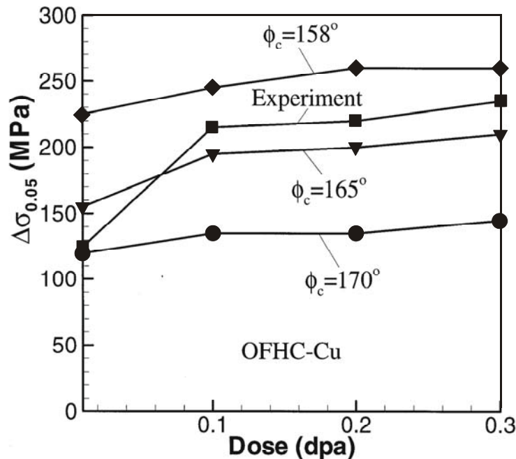
Figure 27. Comparison between the dose dependence of the calculated increase in flow stress (due to irradiation) values and the experimental measurements of Singh, Edwards and Toft (unpublished work).
