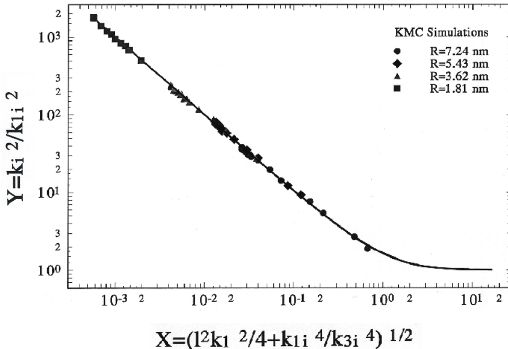
Figure 26. The Master Curve relating 3D and 1D reaction kinetics. Data points are the results of KMC simulations shown in Figure 25 and the full line is the result of analytical calculations.
