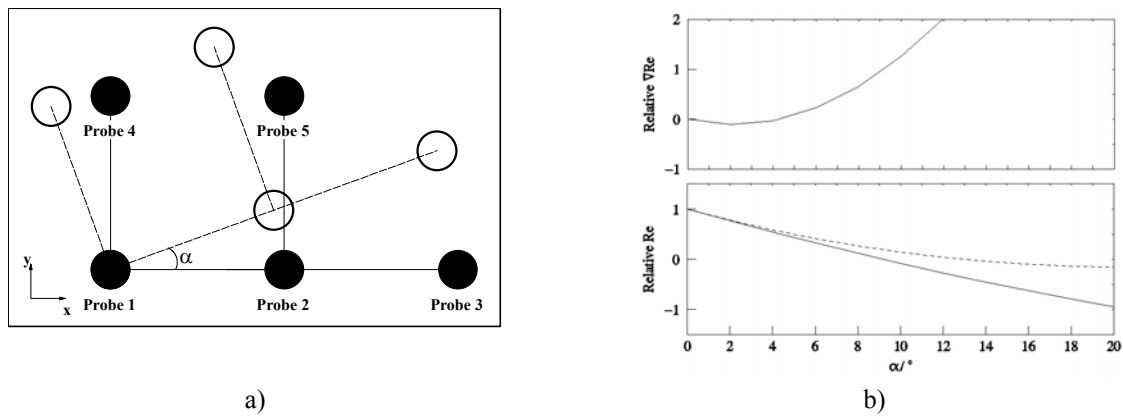
Figure 13. a) The probe array used in the numerical investigations of the effects of misalignment. b) The upper graph shows the difference of the "measured" divergence of the Reynolds stress and the value for perfect alignment relative to the latter as a function of the misalignment angle \alpha . The lower graph shows the change of the Reynolds stresses measured by probes 1, 2, 4 (full line) and probes 2, 3, 5 (dashed line) relative to the Reynolds stresses for perfect alignment.
