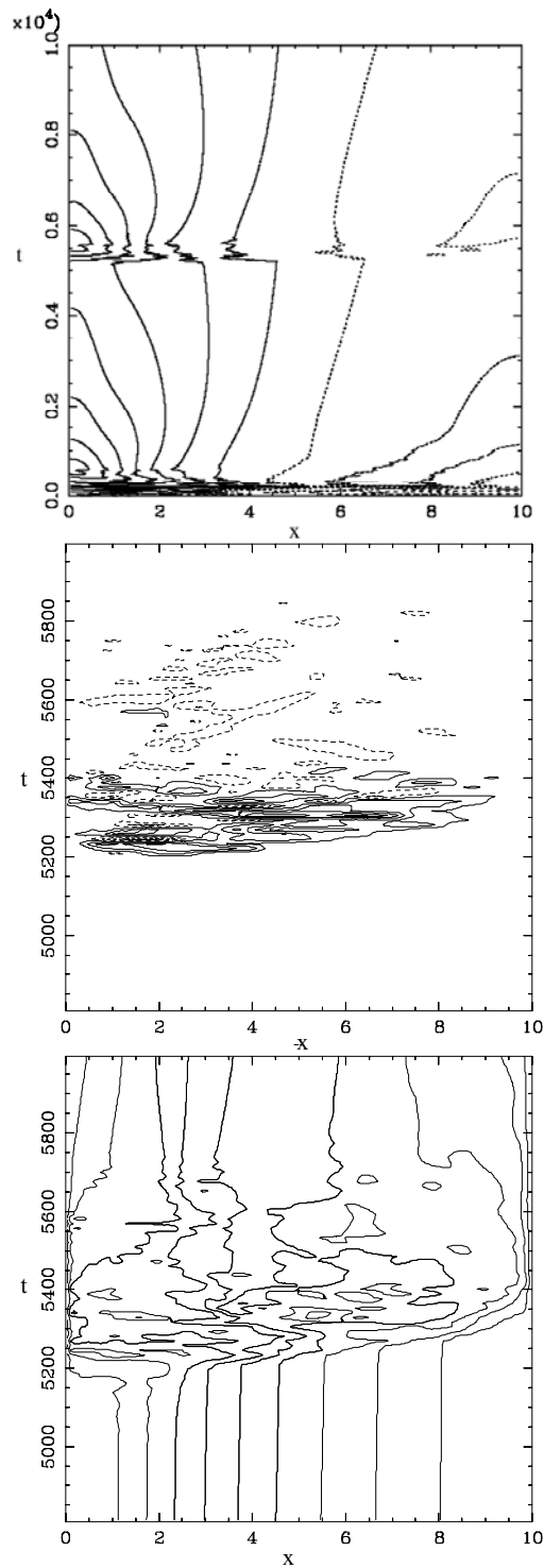
Figure 10. Upper panel: Contours of the zonal velocity, V , over time. Middle and lower panels: Enlarged with respect to time for the flux burst \Gamma_T(t) plotted versus (x,t) and the temperature profile over time.
