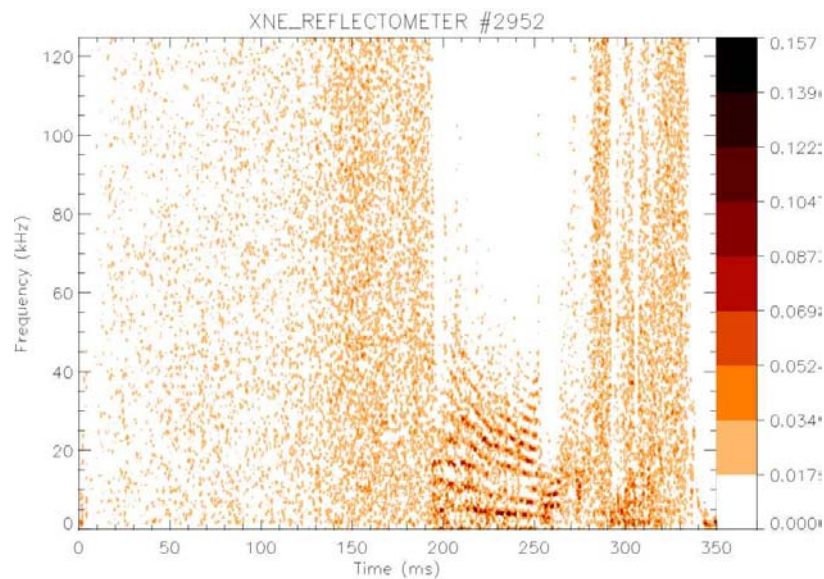
Figure 5. Spectrogram of MAST shot no. 2952 where the H-mode starts at t = 195 ms and a low frequency mode structure builds up. Data from the MAST fluctuation reflectometer.
