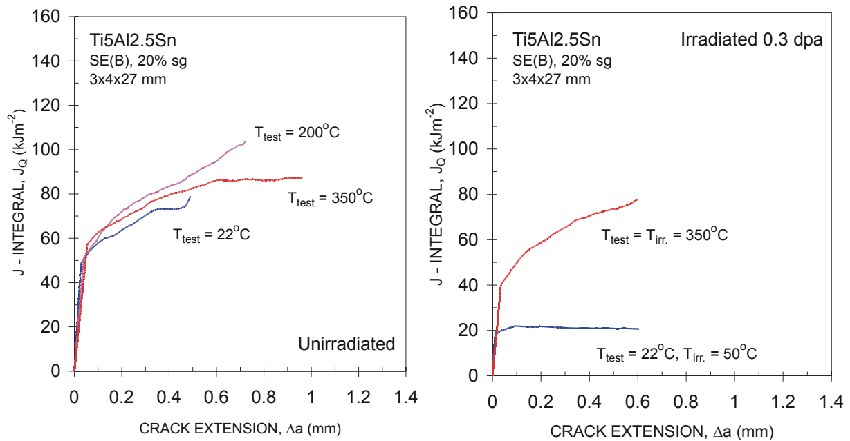
Figure 20. Fracture resistance curves for \alpha -titanium alloy at different test temperatures in the unirradiated and neutron irradiated conditions.
