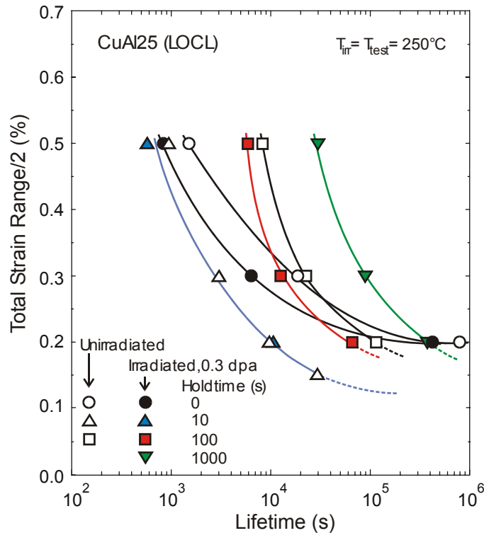
Figure 14. Fracture lifetime as a function of strain range in creep-fatigue interaction tests with different holdtime carried out at 250°C on the dispersion strengthened CuAl-25 alloy.
