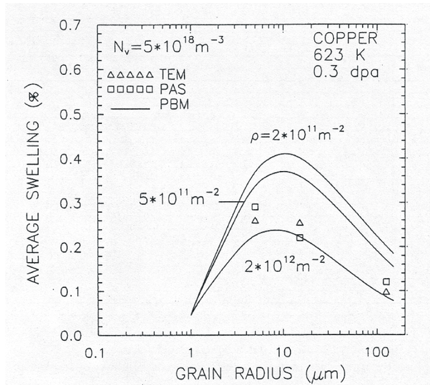
Figure 29. The grain size dependence of the average void swelling calculated (full lines) using PBM and measured experimentally using TEM ( \Delta ) and PAS ( \square ).
