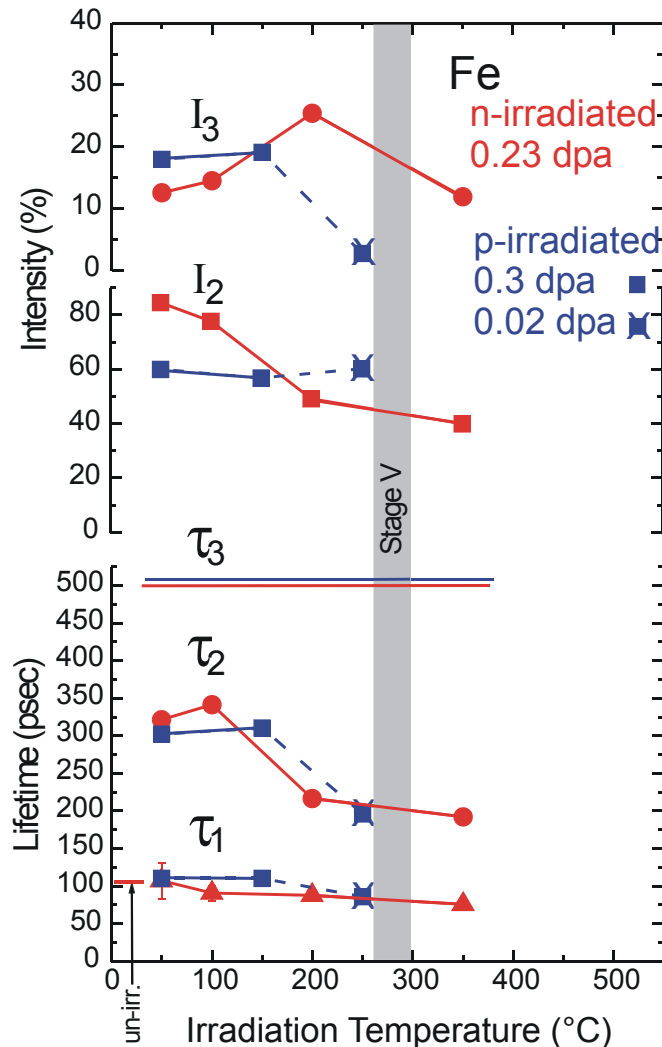
Figure 24. The variation of positron lifetimes and their intensities with irradiation temperature for iron irradiated with neutrons (red) and 600 MeV protons (blue). The lifetimes \tau_2 and \tau_3 are characteristic for different types of defects. At low temperatures both voids ( \tau_3 = 500 ps as shown by straight lines) and micro-voids ( \tau_2 \sim 300 - 350 ps) are formed, while at higher temperatures no micro-voids are seen. The intensities I_2 and I_3 of the lifetime components give information about the defect densities.
