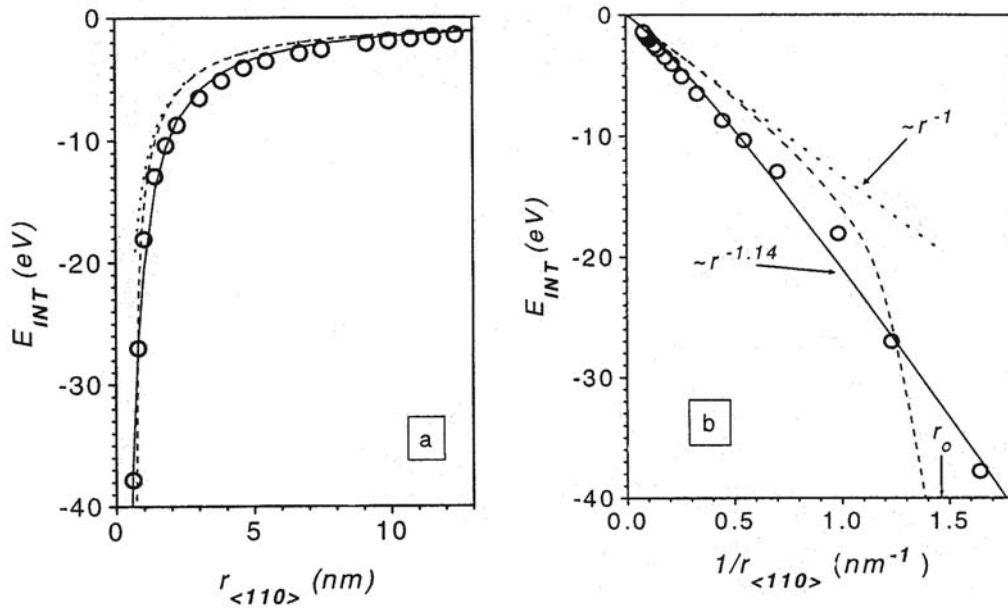
Figure 23. Interaction energy between 1/2 \langle 111 \rangle edge dislocation and a perfect loop of 37 SIA in bcc iron as a function of (a) separation distance along \langle 110 \rangle direction and (b) reciprocal of the separation distance. Full line (—) power function fitted to the MD simulation data, dashed line (- - -) full isotropic elasticity calculation and dotted line (.....) infinitesimal loop approximation (reciprocal distance law) calculation.
