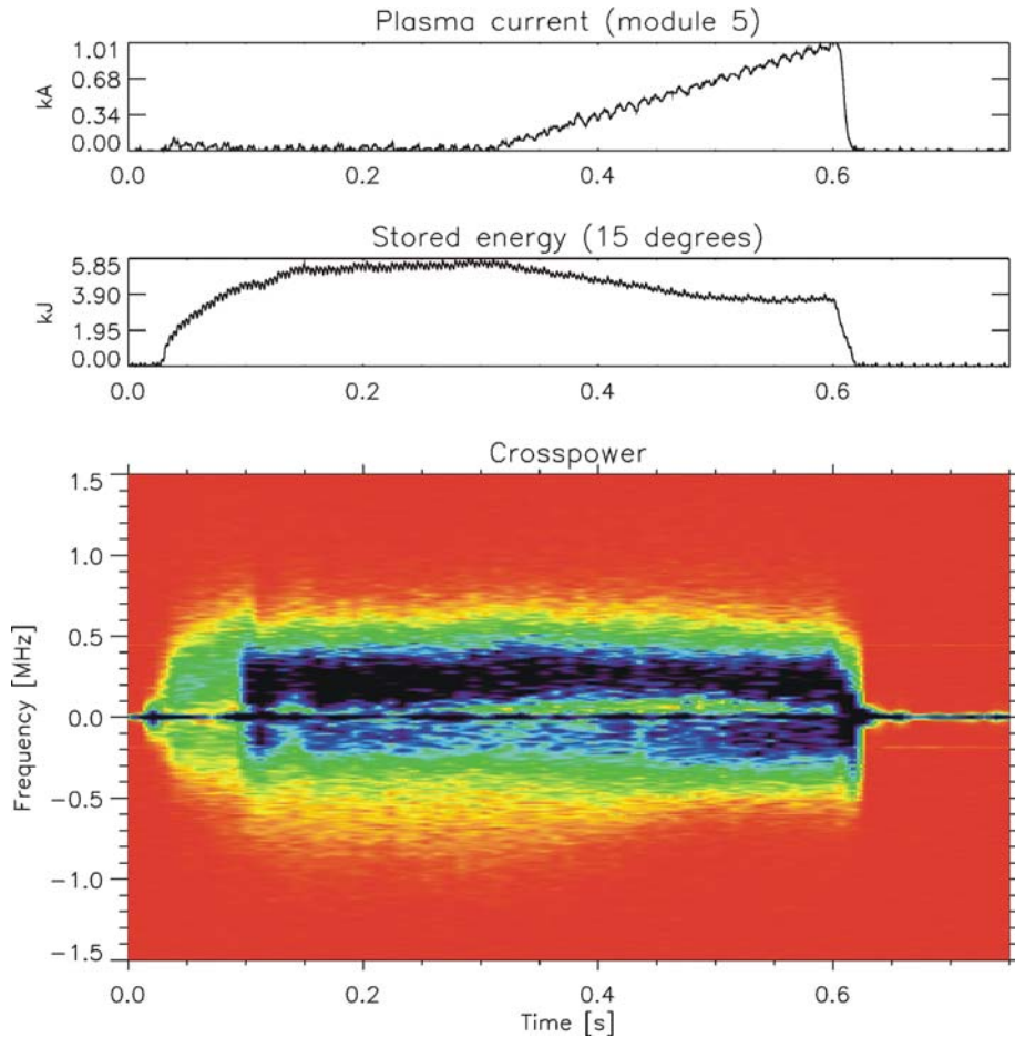
Figure 2. From top to bottom: Net plasma current, stored energy and crosspower amplitude (linear scale) versus frequency and time. The wave number of the density fluctuations measured was 20 \text{ cm}^{-1} . The relative angle between the volumes \theta_R = 4 degrees (centre of plasma, shot 50031).
