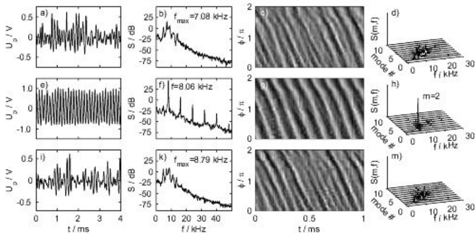
Figure 7. Temporal and spatiotemporal drift wave dynamics: experiment. The three rows correspond to the unperturbed case, active exciter with a co-rotating field and active exciter with counter-rotating field, respectively. The four columns show the density fluctuations, the frequency power spectrum, the spatiotemporal density fluctuations and the frequency mode number power spectrum. Power spectra are obtained by Fourier transformation of the temporal and spatiotemporal data.
