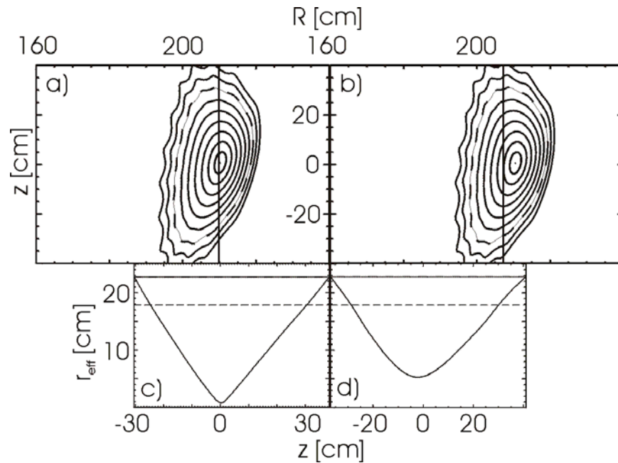
Figure 1. Comparison of measurement position relative to \tau_a = 0.344 flux surfaces in 1999 (inset a, R = 209.8 cm) and 2000 (inset b, R = 207.2 cm). The vertical lines indicate the approximate measurement volume position. Insets c and d show the effective radial coordinate r_{\text{eff}} along the vertical measurement volumes. The dashed lines show the last closed flux surface, and the dotted lines show the plasma boundary.
