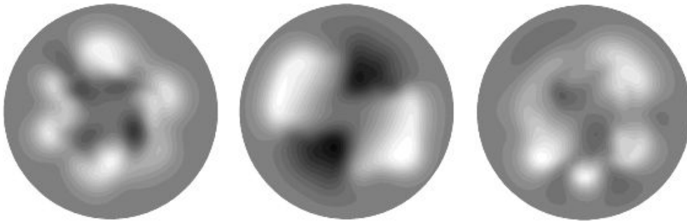
Figure 9. Snapshots of the 2D mode structure as taken from the simulations. Grey scale plots of the density fluctuations; from left to right: Unperturbed case, co- and counter-rotating current profiles.
