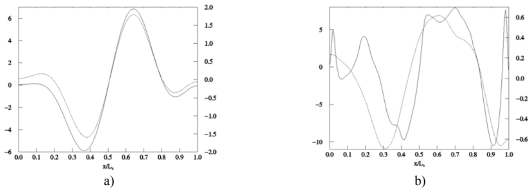
Figure 12. The poloidal flow (dashed line) compared with the flow predicted by the drift wave pseudo-Reynolds stress (full line) at two instants in time a) t = 75 and b) t = 125 .
