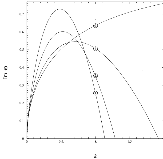
Figure 11. Growth rate of the zeroth (most unstable) mode versus wave number for an inverted stratification. The curve numbers correspond to the value of U_0 .
