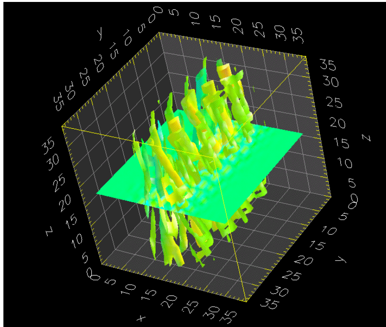
Figure 6. Density fluctuations in a sheared magnetic field. The alignment of the fluctuations with the magnetic field structure and initial localisation at the resonant flux surface can be clearly seen.
