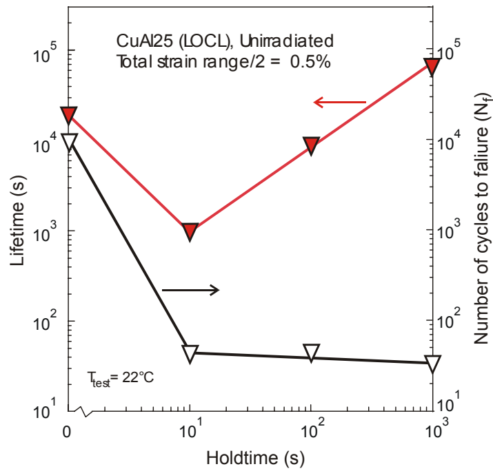
Figure 16. The same as Figure 15, but for tests carried out only on unirradiated specimens and only one strain range value of 0.5% at 22°C.
