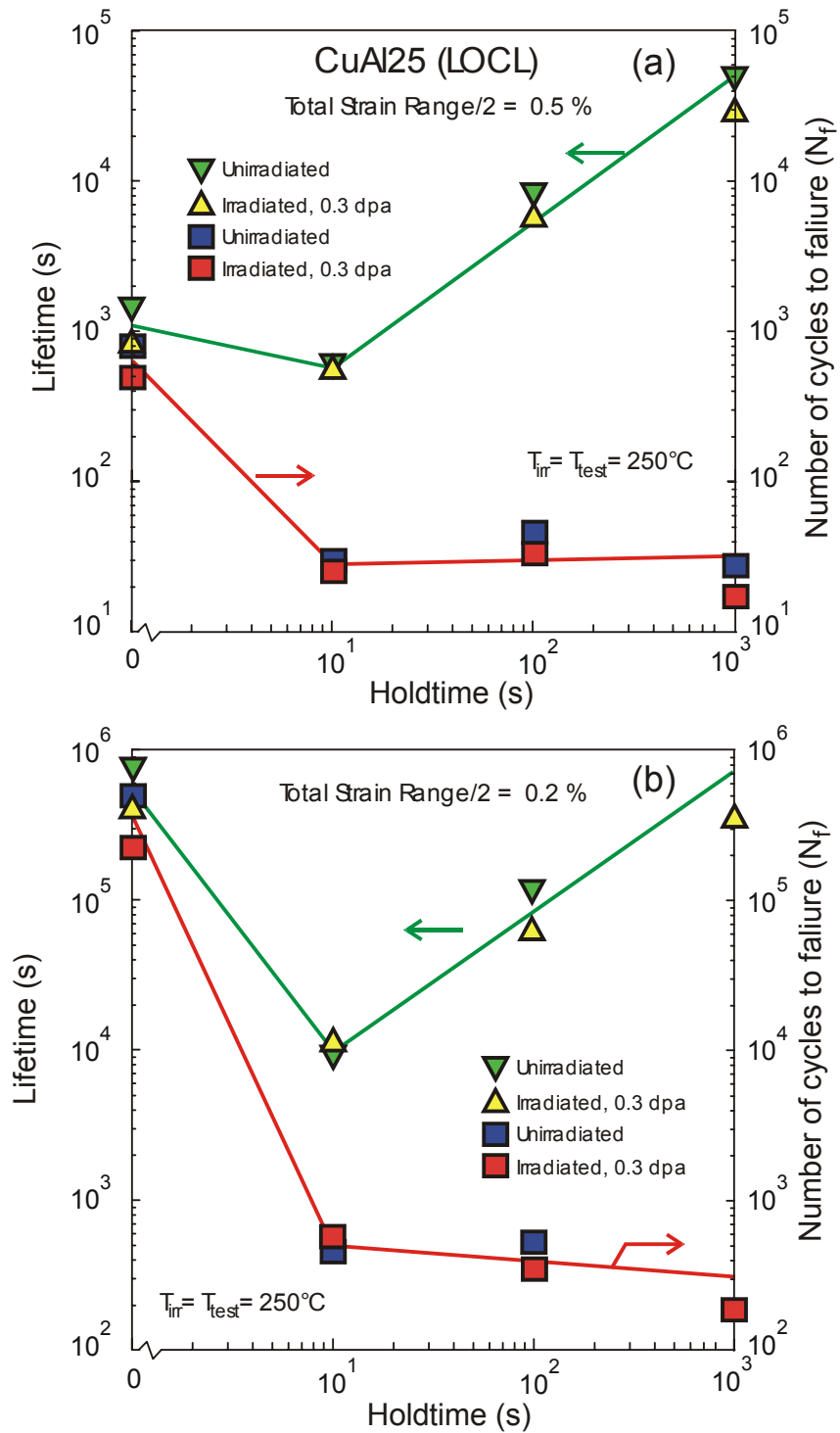
Figure 15. Fracture lifetime and number of cycles to failure as a function of holdtime obtained during creep-fatigue interaction tests at 250°C on CuAl-25 alloy. Results are shown for both unirradiated and irradiated materials tested at two different strain range values.
