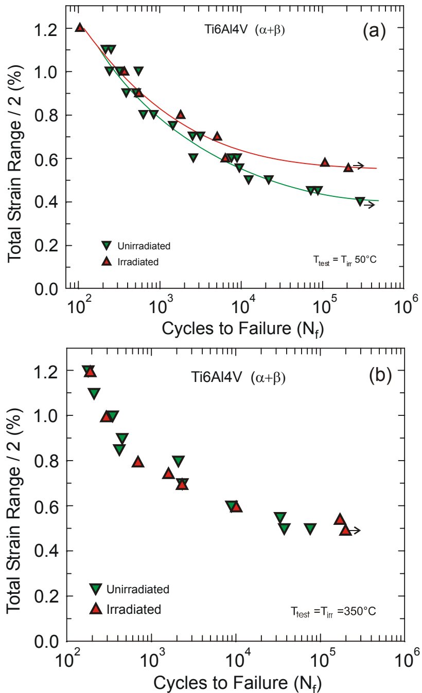
Figure 19. Same as Figure 18 but for the (\alpha+\beta) (Ti6Al4V) titanium alloy.
