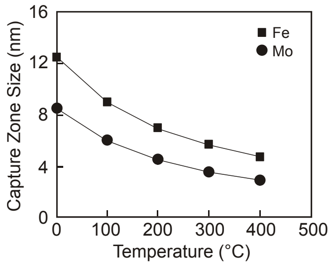
Figure 22. Temperature dependence of the trapping zone size for small defect clusters in bcc iron and molybdenum.
