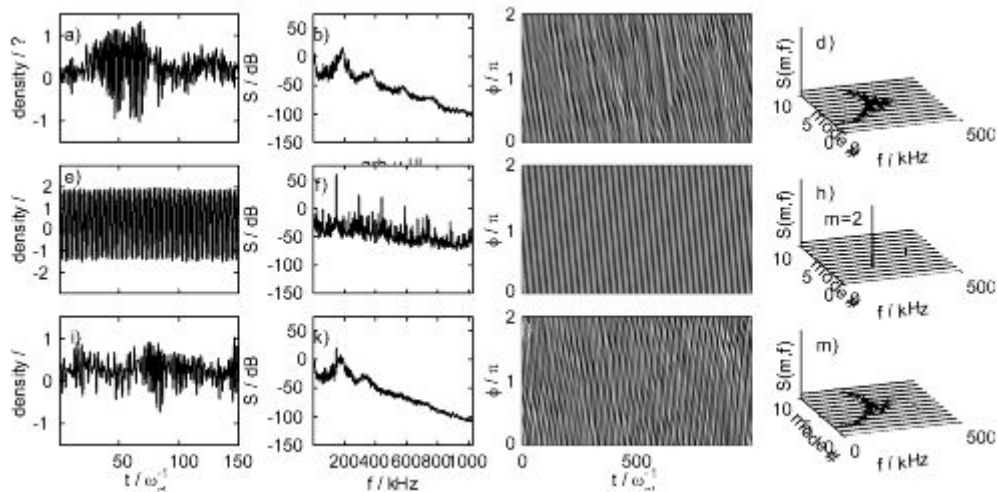
Figure 8. Temporal and spatiotemporal drift wave dynamics: simulation. The figure is arranged as in Figure 7. Excellent agreement is found between experiment and simulation.
