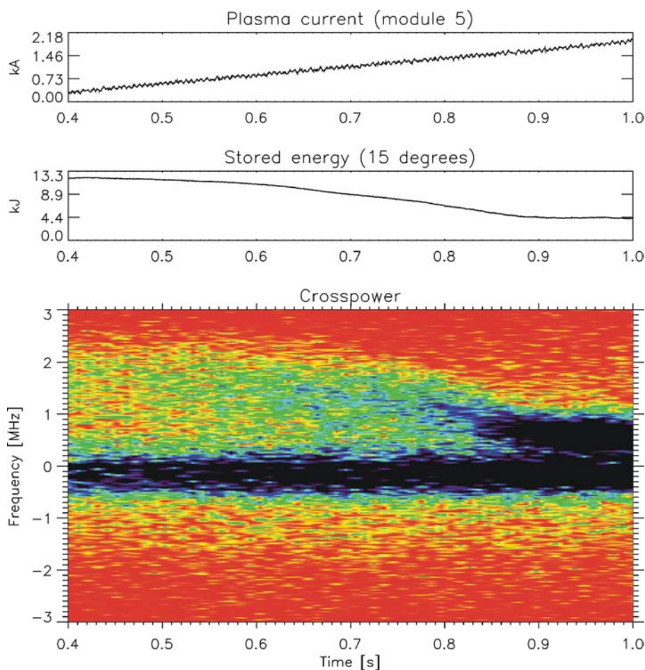
Figure 3. From top to bottom: Net plasma current, stored energy and crosspower amplitude (linear scale) versus frequency and time. The wave number of the density fluctuations measured was 15 \text{ cm}^{-1} . The relative angle between the volumes \theta_R = 10.5 degrees (bottom of plasma, shot 47940).
