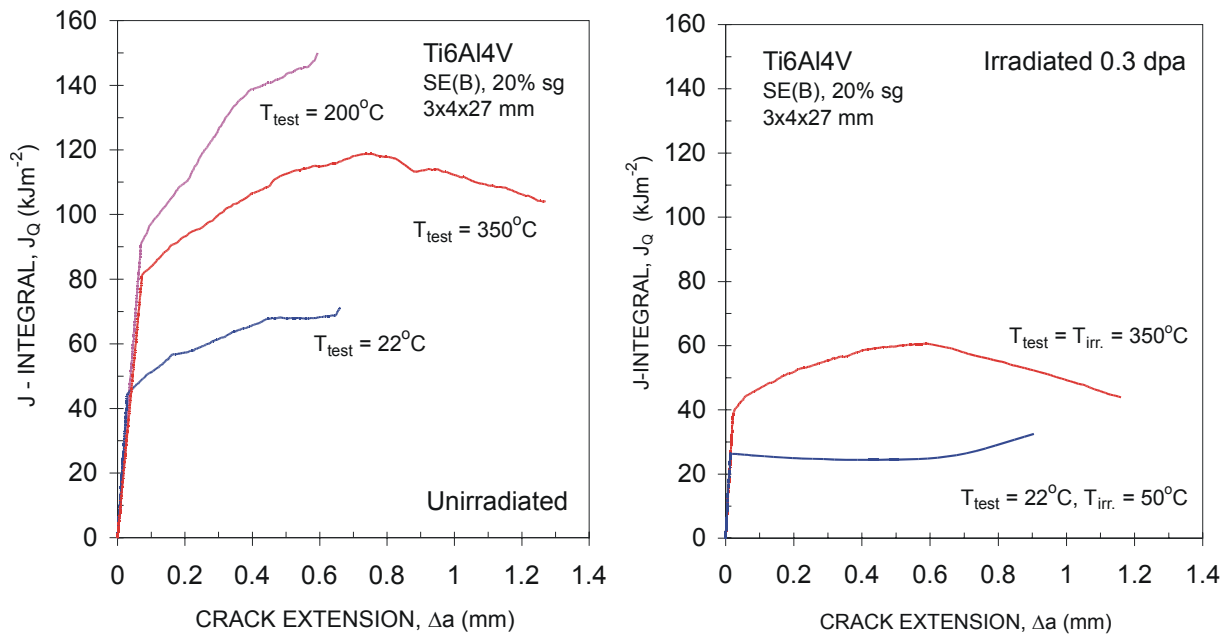
Figure 21. The same as Figure 20 but (\alpha+\beta) -titanium alloy.
