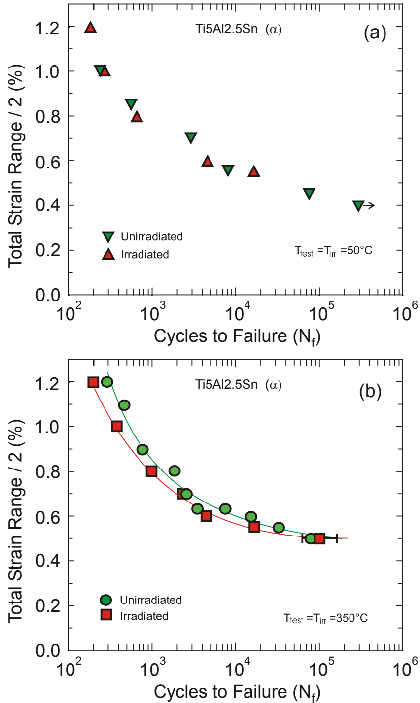
Figure 18. Fatigue lives of the \alpha(\text{Ti5Al2.5 Sn}) titanium alloy determined at 50 and 350°C in the unirradiated and irradiated conditions.
