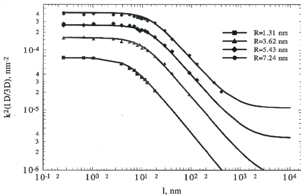
Figure 25. A comparison of the analytical expression (curves) and computer simulation results (points) for the sink strength of a random array of absorbers of number density, N , and radius, R , as a function of L , the ID path length of migrating defects under mixed 1D 3D migration. Data for four different values of R are shown.
