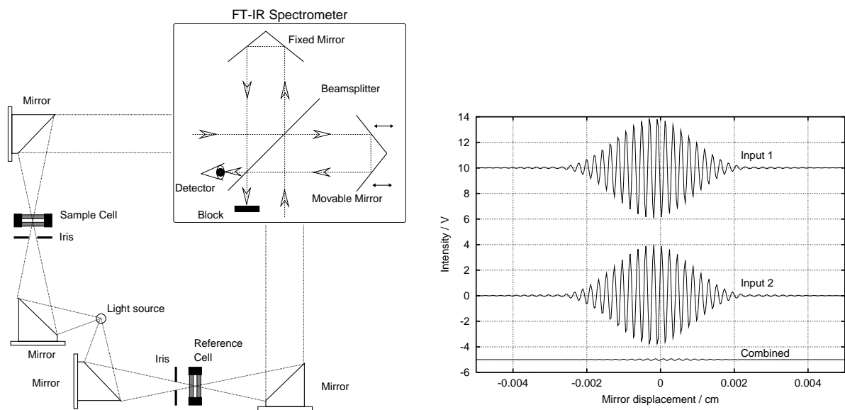
Figure 40. Left: Schematic drawing of optical subtraction instrumentation. Right: Interferogram from inputs 1, 2, and optical subtraction.
