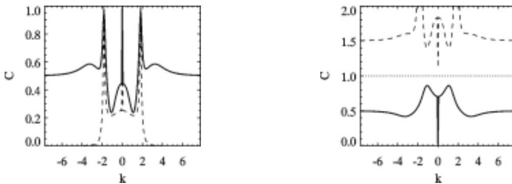
Figure 60. Left: Intensity correlation function in the far field, normalised so that C = 1 is the perfect correlation and C = -1 is the perfect anti-correlation. The full (dashed) line is the fundamental (second-harmonic) correlation between +k and -k calculated analytically just below threshold for pattern formation. Right: A plot in the far field showing the fundamental photon number variance of the sum (dashed line) and difference (full line) between intensities at +k and -k , respectively. The dotted line shows the shot noise level, i.e. the limit between classical and quantum behaviour.
