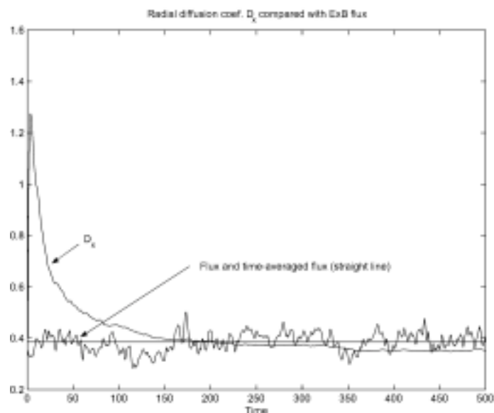
Figure 50. The running diffusion coefficient, D_x , obtained from following the trajectory of 5000 test particles, compared with the turbulent flux.
