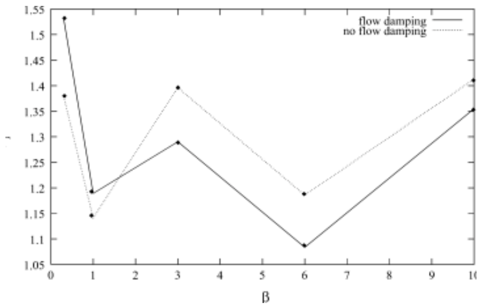
Figure 47. Flux versus normalized plasma beta for runs with and without zonal flow damping. A crossover in the flux scaling can be seen for beta larger than 1.5.
