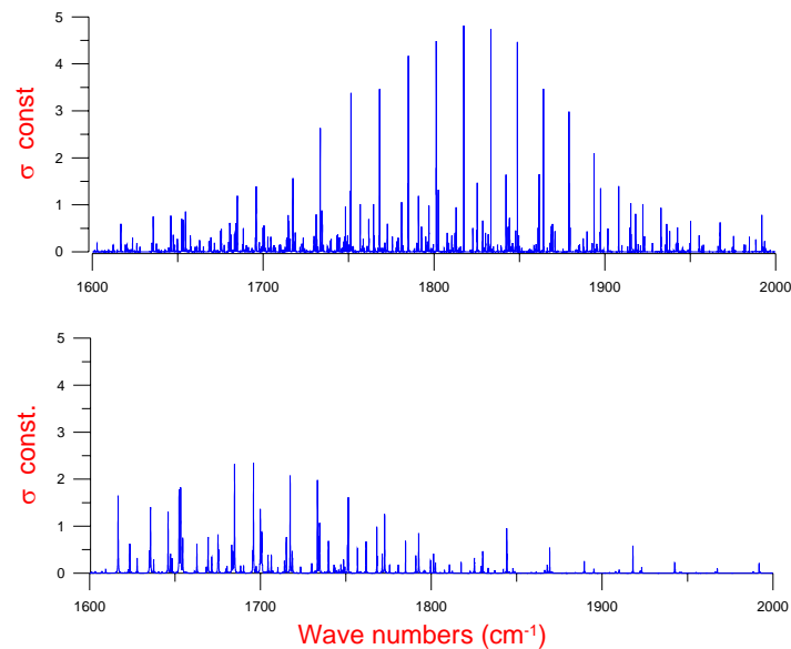
Figure 42. An example of the big difference in shape between the 300 K (lower spectrum) and 650 K (upper spectrum) H 2 O absorption cross sections. The described method based on PCA is capable of modelling this nonlinear relationship between absorption cross sections and temperatures.
