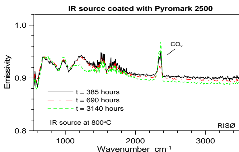
Figure 43. Example of repeated emissivity measurement of small IR source coated with Pyromark 2500. A minor change in emissivity is seen at 1050\text{--}1400\text{ cm}^{-1} after 3140 hours due to reactions with the base material.
