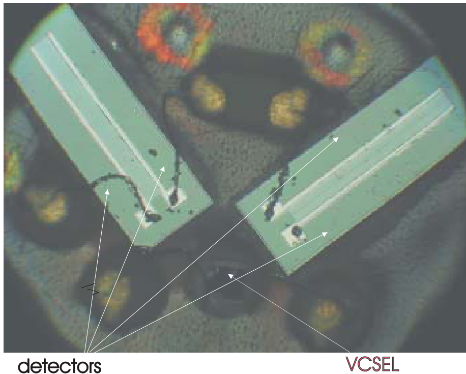
Figure 34. The optical unit placed in the tip of the pen has a diameter of 7 mm and includes four detectors and one VCSEL, sized 300 \mu\text{m} by 300 \mu\text{m} .
