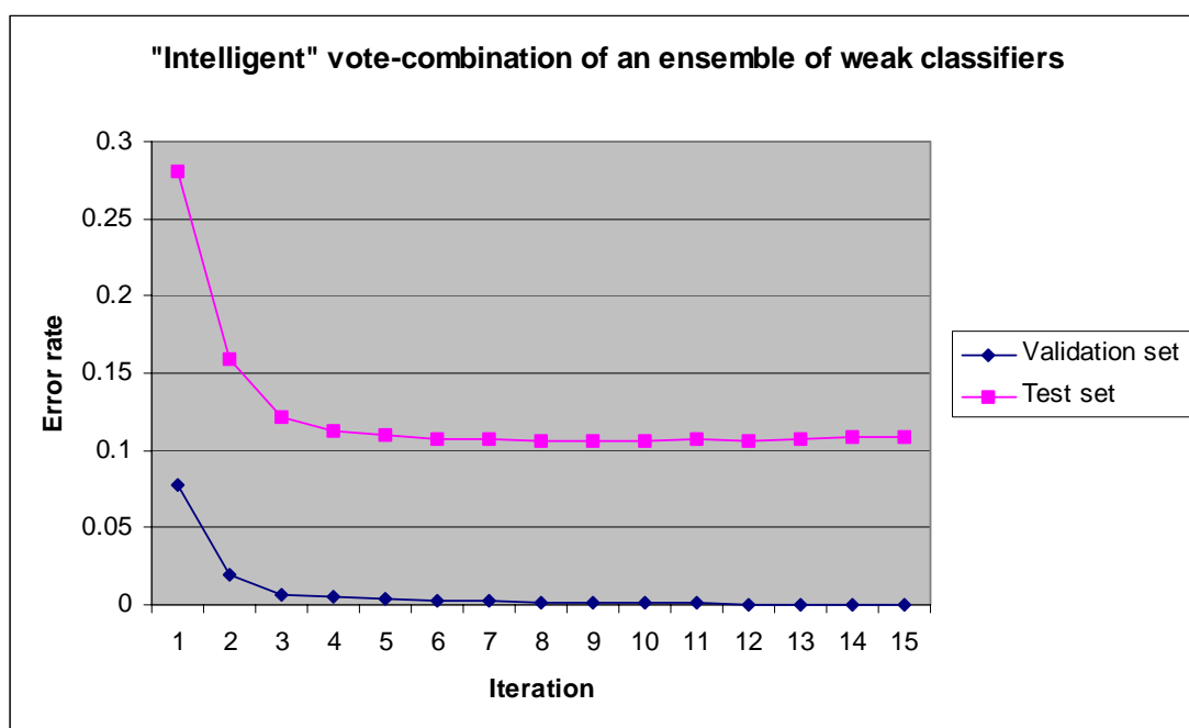
Figure 20. The two graphs illustrate how the performance of an ensemble of 100 weak classifiers (PERT decision trees) can be improved by applying an iterative scheme for adjusting the contribution of the different branches of the decision trees to the overall decision. The validation set and test set error rates are obtained on the so-called DNA data set from the Statlog repository (see http://www.niaad.liacc.up.pt/statlog/datasets/dna/dna.doc.html ).
