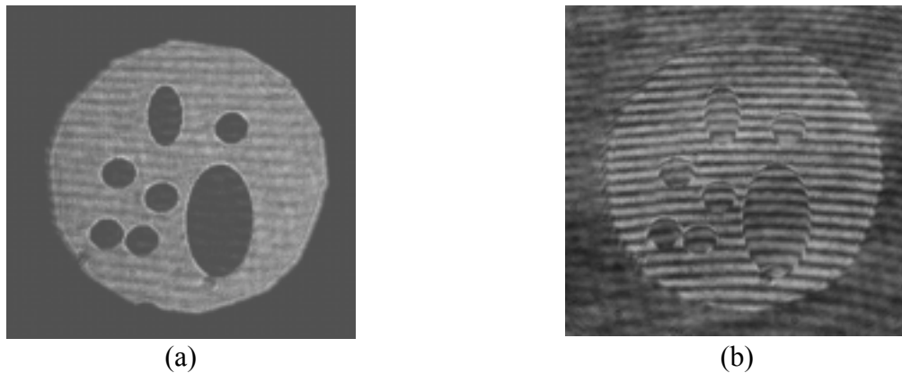
Figure 26. Experimental results for the generation of phase modulation using an SLM operating as the input amplitude modulator. (a) An image of the input amplitude distribution without the filter in place; (b) interference fringe measurement of the output phase modulation.
