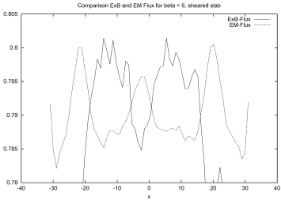
Figure 46. Radial flux surface and time averaged profile of the EXB and the electromagnetic component of the particle flux (note that a constant value of about 0.795 is added to the EM component), showing that the EM component is large where the ExB component is small, namely at the transport barrier.
