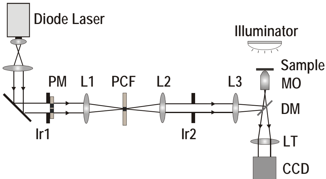
Figure 23. A schematic diagram showing the experimental set-up for an optical tweezer system based on multiple-beam phase contrast.
