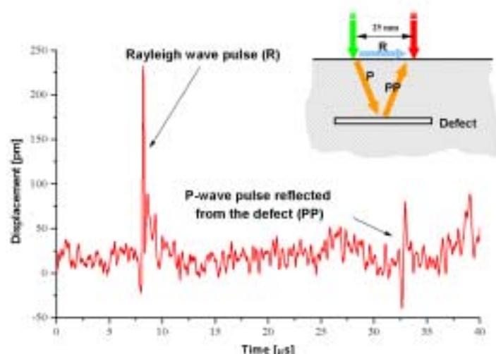
Figure 62. Defect location in a steel bar. The green laser generates an ultrasonic pulse into the material and the red laser is used for interferometric detection of the defect. The result: a received Rayleigh wave and a reflected P-wave. Notice that the reflected P-wave is only visible in the case of a defect.
