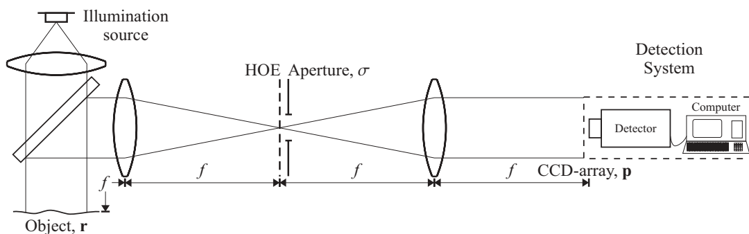
Figure 30. The 4-f set-up for measuring dedicated surface deflections, tilt or vibration.
