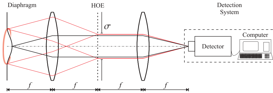
Figure 31. The receiver part of the interferometer for measuring changes in curvature.
