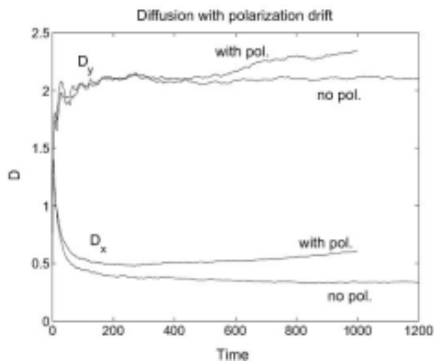
Figure 49. The diffusion coefficients for “alpha particles”, with and without the polarisation drift.
