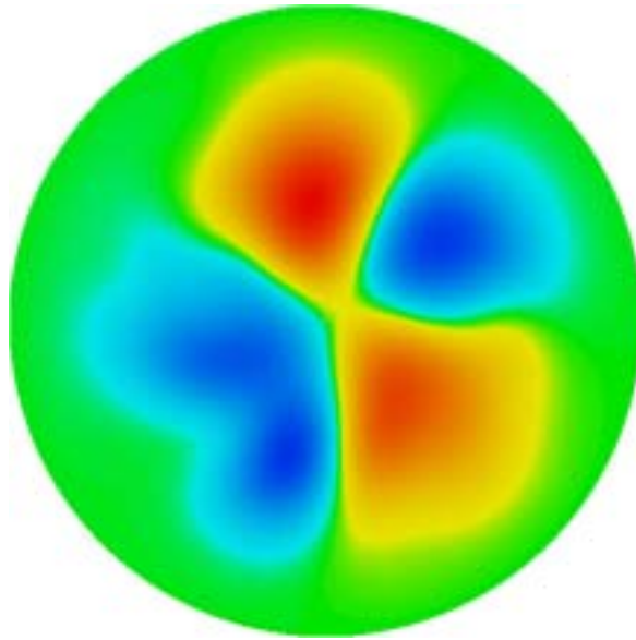
Figure 45. An m = 2 mode with about 3% fluctuation amplitude develops in these 3D simulations of a linear plasma device.
