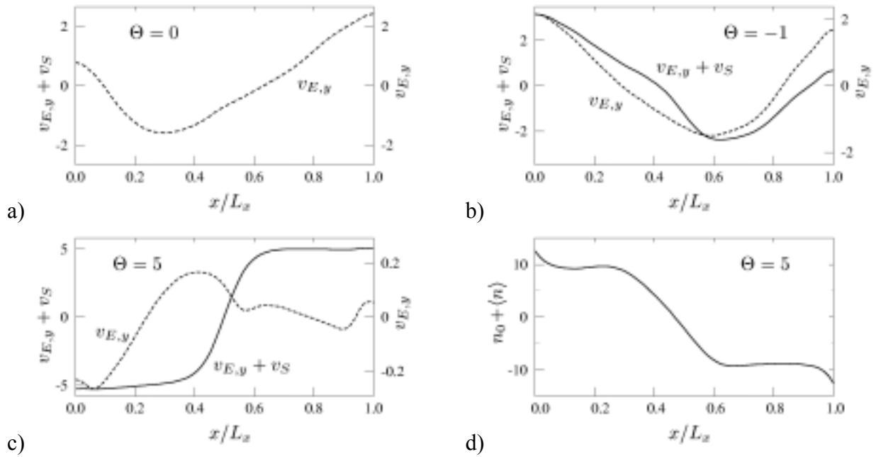
Figure 54. Self-generated shear flow \bar{v}_{E,y} (dashed line) and total shear flow \bar{v}_{E,y} + \bar{v}_S (full line) profiles for a) ( \Theta = 0 ), b) ( \Theta = -1 ) and c) ( \Theta = 5 ); d) the radial density profile for ( \Theta = 5 ). The scale for the full line is to the left.
