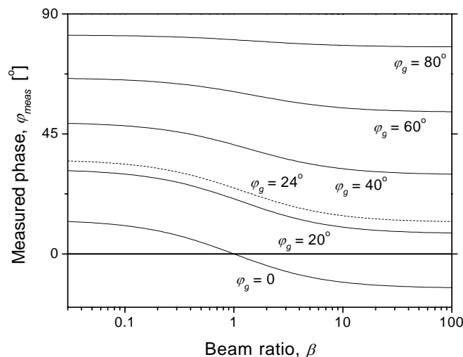
Figure 5. \varphi_{\text{meas}} versus beam ratio \beta for different values of \varphi_g .
