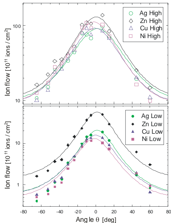
Figure 13. The angular distribution of the ablated ions in units of 10^{11}/\text{cm}^2 for four metals at high ( 2.5 \text{ J/cm}^2 ) and low fluence ( 0.8 \text{ J/cm}^2 ).
