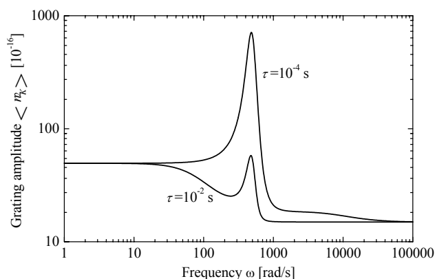
Figure 1. Frequency dependence of the first-order grating amplitude for two different values of \tau . The two curves illustrate the cases \tau\omega_{ac} > 1 and \tau\omega_{ac} \ll 1 , respectively, where \omega_{ac} \approx 500 rad/s is the ac enhancement resonance frequency.
