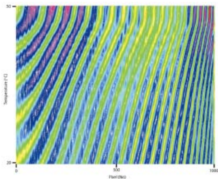
Figure 22. The interference pattern from pure water in the capillary tube at varying temperature. From these measurements, a refractive index sensitivity of 5 \times 10^{-6} may be inferred.
