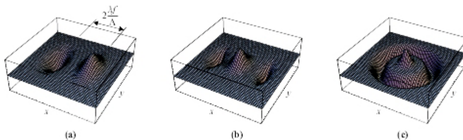
Figure 32. Impulse response for (a) shearing system (tilt sensor), (b) a one-dimensional, and (c) a two-dimensional curvature interferometer.
