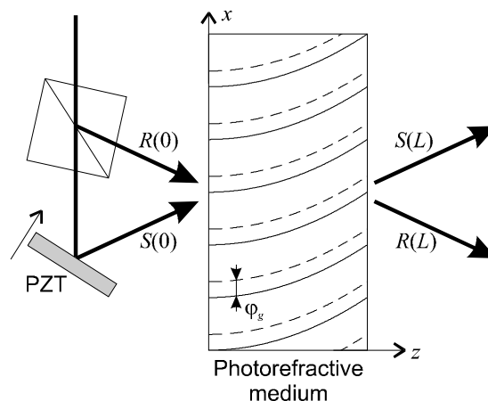
Figure 4. Schematic set-up showing the grating translation technique. The PZT is a piezodriven mirror that can be translated uniformly to induce a linearly increasing phase shift between the reference (R) and signal (S) beams, respectively. \varphi_g is the phase shift between the illuminating light interference pattern and the induced photorefractive grating. This phase shift is called the photorefractive phase shift.
