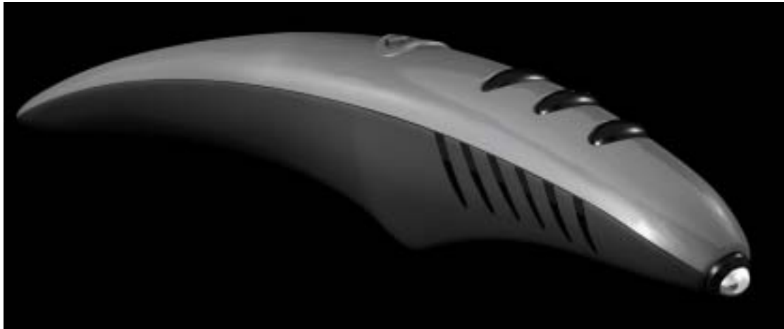
Figure 33. Side view of the Zeptor pen. The pen tip consists of a rotating steel ball, the rotation of which is recorded by an imbedded laser-based system.
