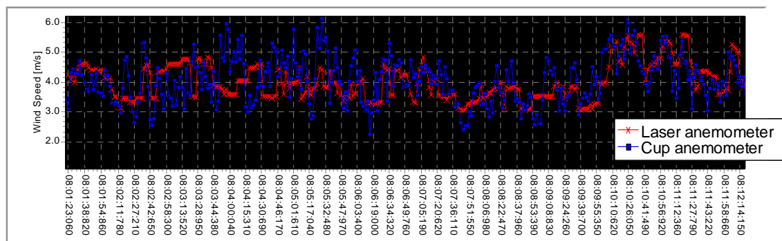
Figure 38. Comparison between the wind velocities measured by the cup anemometer (squares) and by the laser anemometer (cross).
