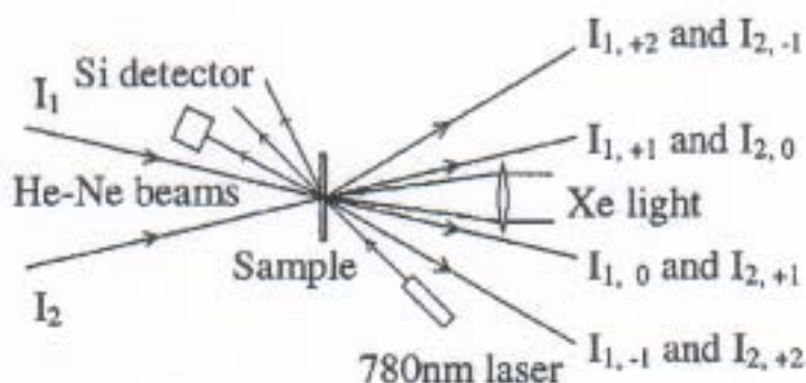
Figure 6. Biphotonic polarisation holographic set-up showing the recorded ( I_1 and I_2 ) and diffracted beams ( I_{i,j} ) of the He-Ne laser.
