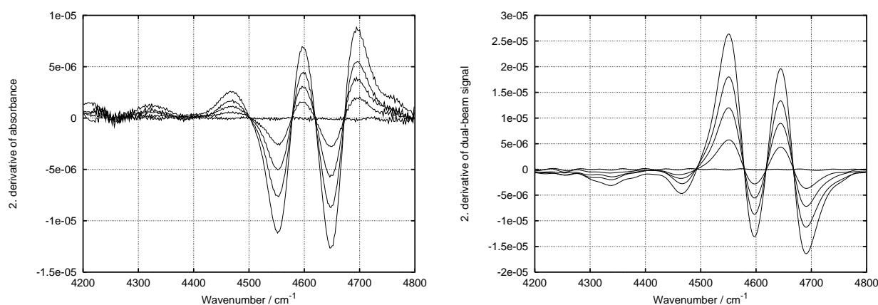
Figure 41. Second derivative of urea signals in concentration range 0-1 g/dl. Left: Traditional absorbance. Right: Optical subtraction.
