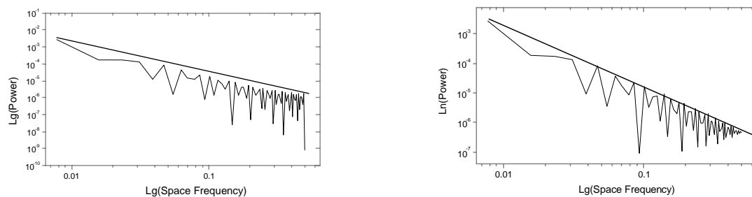
Figure 39. The experimentally found power spectra for random (a) and fractal (b) surfaces.
