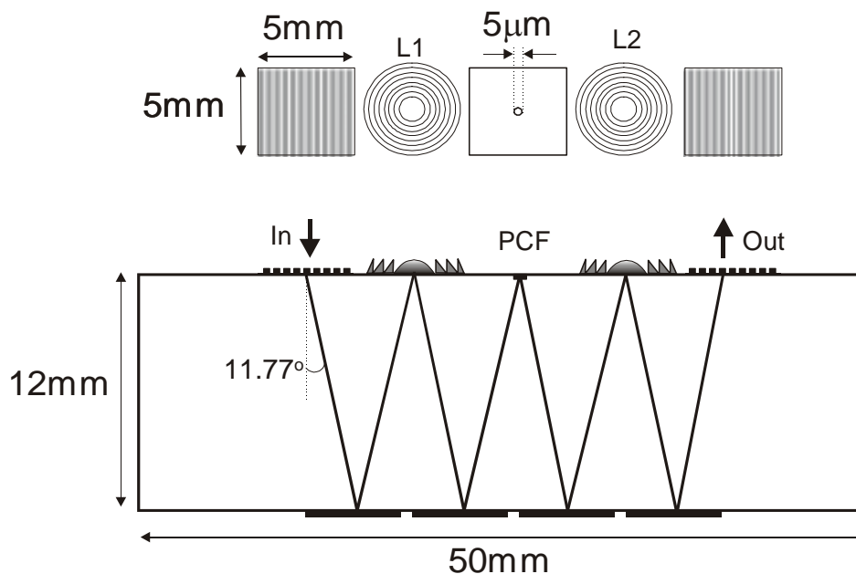
Figure 27. Implementation of the generalised phase contrast method in a planar, integrated micro-optics platform. Diffractive optical elements form the 4-f optical system that is fabricated on top of a 12 mm thick quartz glass substrate. The 5 µm diameter phase contrast filter is etched at the Fourier plane.
