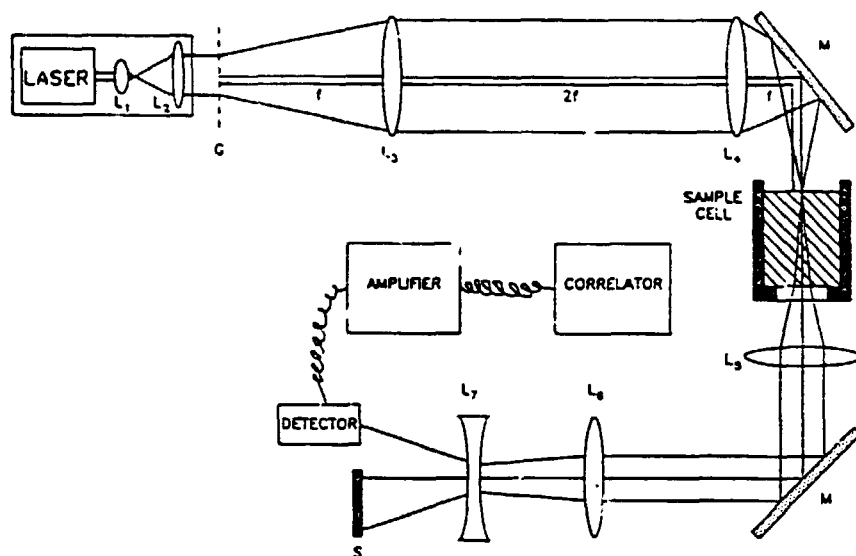
Fig. 1. The experimental setup. L denotes a lens, M a mirror, and S a spatial filter. G denotes a phase grating, whereas f is the focal length of L_3 and L_4 .
