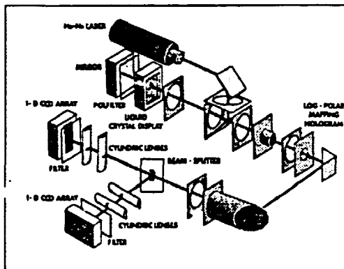
OPTICAL SET - UP
