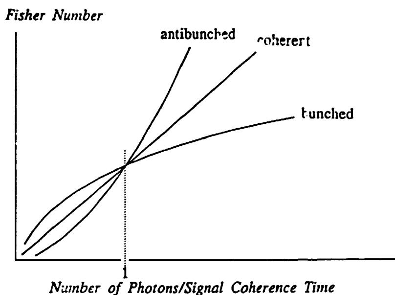
Figure of merit versus mean photon rate for the detection of changes in a weak phase object. (a) is for antibunched light with a coherence time longer than the coherence time of the object, (b) is for coherent light, and (c) is for bunched light.
