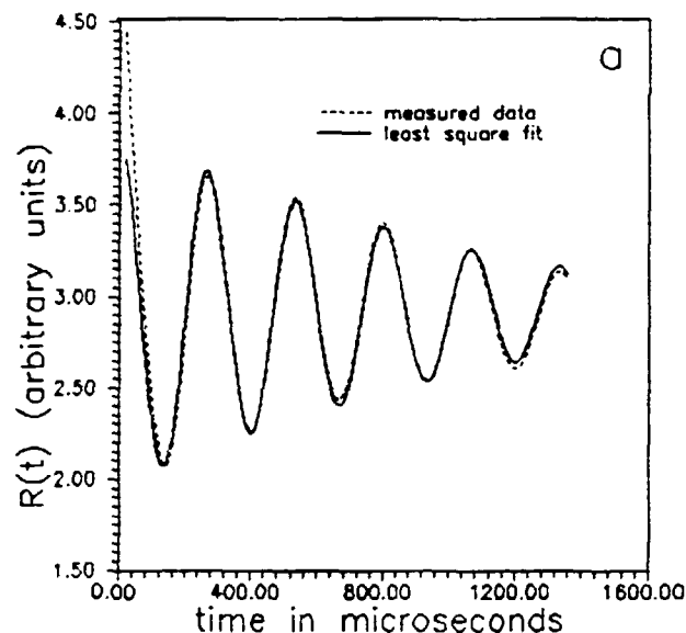
Fig. 2. Measured and fitted autocorrelation for hexane at 25 C. 2\pi/L = 273(\text{cm})^{-1} .
