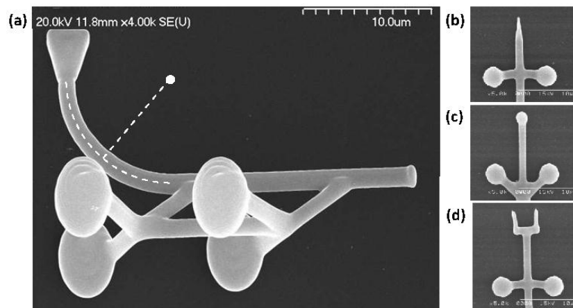
Fig. 2. SEM images of representative two-photon polymerized structures: a) A bent waveguide (bending radius R \sim 8 \mu\text{m} ; width \sim 1.5 \mu\text{m} ) sitting atop a supporting structure having spheroidal handles for optical trapping; the waveguide is connected via reverse-angled rods for minimal light-coupling loss the support structure; b) – d) Some tip structures that can be fabricated
