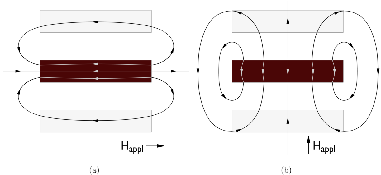
FIG. 2: Illustration of the magnetic field resulting from the magnetization of a single rectangular plate. In (a) the field is along the x -direction and thus parallel to the largest face of the plate. The resulting stray- or interaction field tends to oppose the applied field in the adjacent plates. In (b) the field is along the z -direction. The demagnetizing field inside the body is larger than in (a), however, the stray field tends to enhance the applied field in adjacent plates.
