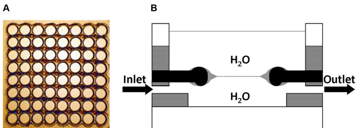
Figure 6.1. (A) An optical image of an array (8x8) of apertures (300 μm in diameter, 400 μm neighbouring apertures centre to centre distance) made in ETFE partition used for biomimetic membrane formation in a device constructed for AFM imaging 93 . (B) A schematic cross-sectional view of the conceptual device for BPMs investigation with AFM. The fluid polymer membrane (gray) is formed across a circular aperture (300 μm diameter) in an ETFE scaffold (black) by injecting the polymer solution through inlet and outlet microchannels made in a spacer ring (dashed grey boxes) of the bottom chamber. The top chamber is open for AFM. The device is clamped via two supportive transparent structures (white boxes) 28 .
