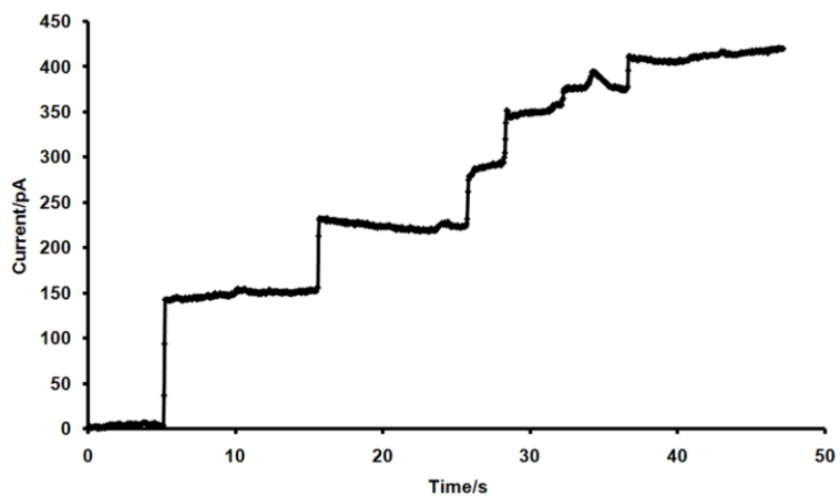
Figure 6 Current trace of the reconstitution of the pore-forming heptameric \alpha -HL membrane protein in established in the microfluidic device 8 \times 8 bilayer arrays.
