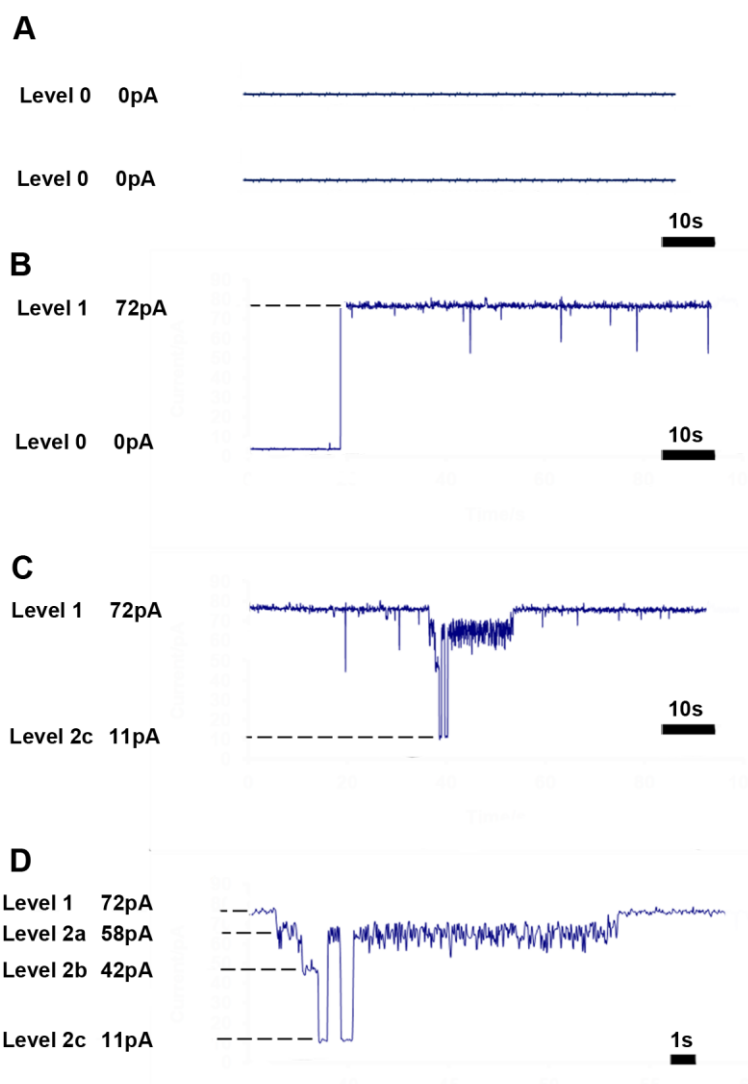
Figure 8.7. Electrical recordings showing: (A) No transmembrane currents (Level 0) observed when \beta -CD (upper current trace) or when a detergent (LDAO) in buffer followed by \beta -CD addition (lower current trace) were applied to the DPhPC/decane membrane made across a 0.7 mm hole in Teflon in 1 M KCl using a horizontal device. (B) FomA trimer incorporation into a lipid bilayer, Level 1. (C-D) FomA current blockage after addition of 10 \mu l of 10 mM \beta -CD, Levels 2a, 2b and 2c. The applied potential across the membrane was +60 mV.
