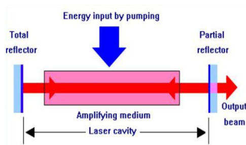
Figure 4.1. A schematic illustration of the basic laser setup. It consists of an amplifying medium with a suitable set of energy levels to support laser action, a source of pumping energy in order to establish a population inversion and an optical cavity or resonator to introduce optical feedback and so maintain the gain of the system overcoming all losses. Figure taken from 98 .
