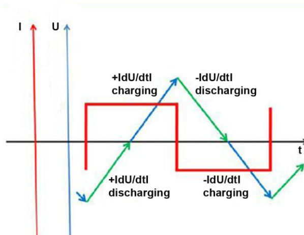
Figure 4.5. A membrane capacitance measurement, showing theoretical relationships between applied triangular input signal, U and the resulting membrane response, I (red). The membranes can be regarded as parallel plate capacitors that continuously cycle between charging and discharging. Whenever dU/dt changes sign the capacitive current changes direction. In between the direction changes the charging and discharging currents are constant since dU/dt is constant. This gives rise to the square shaped membrane response signals. Figure taken from 100 .
