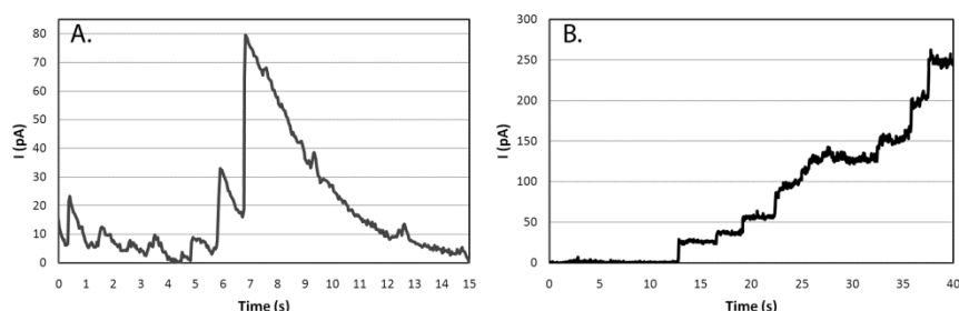
Fig. 2. Vesicle fusion with N/E vesicles and FomA proteoliposomes. A) Current trace of N/E vesicle fusion activity. B) Current trace of FomA proteoliposomes vesicle fusion. Measurements were carried out using voltage clamp technique.
