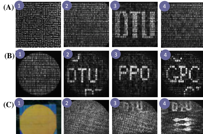
Fig. 4. Phase cryptography using diffractively modulated GPC. (A) Removing edge effects: The undecrypted output, 1 , can show the edges of the hidden letters, but these are removed, 2 , by using pixilated letters, as seen in the decrypted GPC output pattern, 3 . This pattern disappears, 4 , when the GPC filter is removed; (B) Variable keys for an encrypted phase: the same encrypted phase, 1 , may contain different hidden patterns, 2 , 3 , 4 , that are only revealed by using the correct decryption keys. (C) Phase encryption using a hologram master: 1 , White light image of a master hologram with embedded phase within its featureless circular region; 2 , Image of laser diffraction from the circular region; 3 , Undecrypted GPC image of diffraction from the circular region; 4 , Final decrypted GPC image of the encrypted hologram master.
