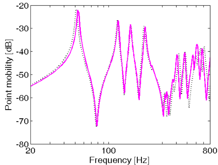
Figure 4-1. Calculated point mobility of a simply supported cross-stiffened rectangular plate. The solid line represents the result for the “exact” FE model; the dotted line is for the smeared FE model. Magnitude shown in dB re 1 m/Ns.
