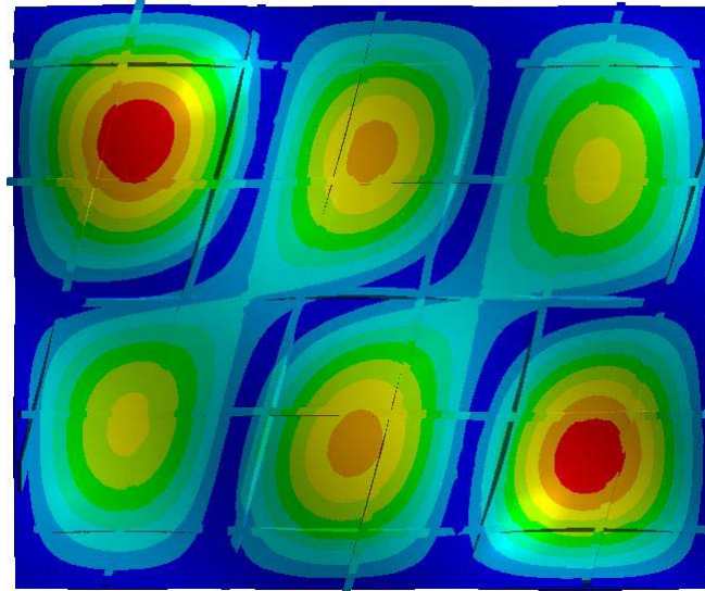
Fig. 13. Modal pattern of mode (3, 2) of the FE estimation of the model with angled y stiffeners.
