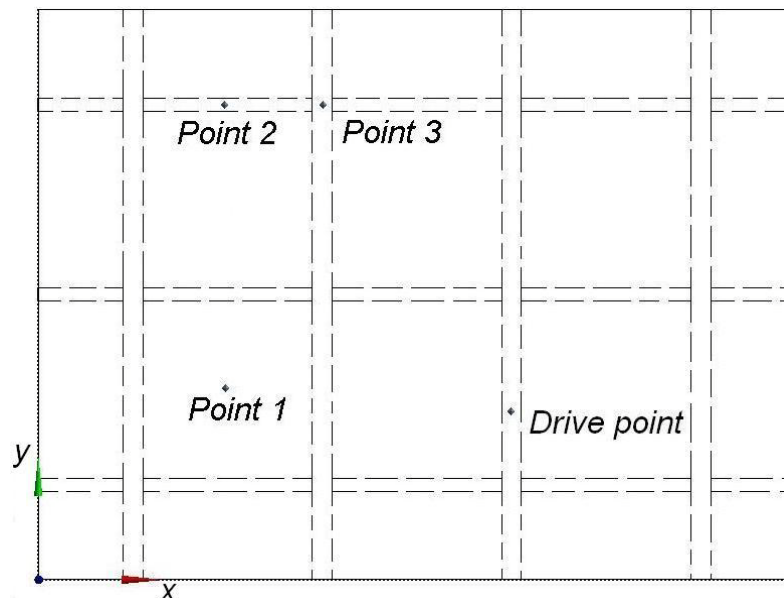
Fig. 7. A sketch of the cross-stiffened plate of model #3. The driving point and the three points for the transfer mobility are shown.
