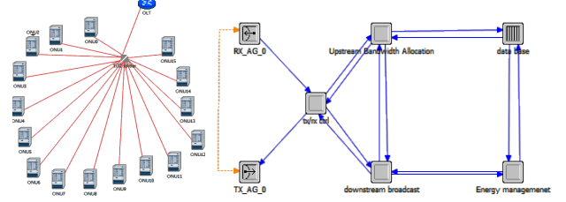
Fig. 4. Simulation setup and control functions in OLT.
