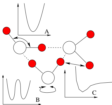
Figure 3.4: A cartoon example of three of the potential energy curves illustrated for the water trimer.
