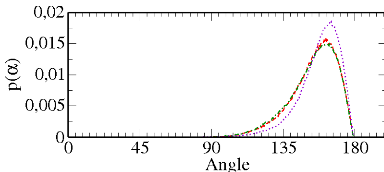
Figure 4.7: The angular distribution functions of the O-H \cdots O angle in liquid water at ambient conditions according to MD simulations. The angle corresponds to \theta in Fig. 2.2
