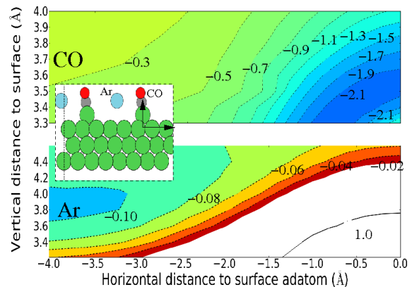
FIG. 1. Spatial difference in interaction energy between strong and weak adsorption surfaces (PES's) for CO (top) and Ar (bottom) adsorbed on Ni(111) surface with Ni adatom (inset), calculated with the vdW-DF method [23]. CO molecule prefers to be close to adatom, while the Ar atom prefers terrace, as indicated by coordinate system in inset. Units are eV and Å.
