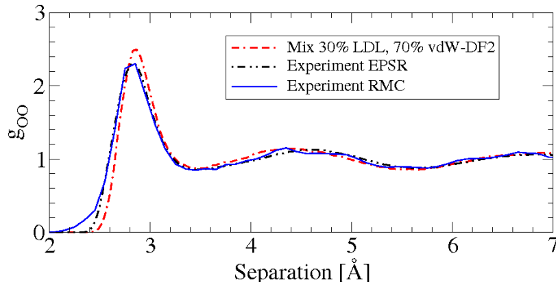
Figure 4.9: Mixing of experimental LDL and vdW-DF2 oxygen-oxygen PCFs compared with PCFs from RMC [106] and EPSR [105]. A mixture of 70/30 agree well with experimental results.
