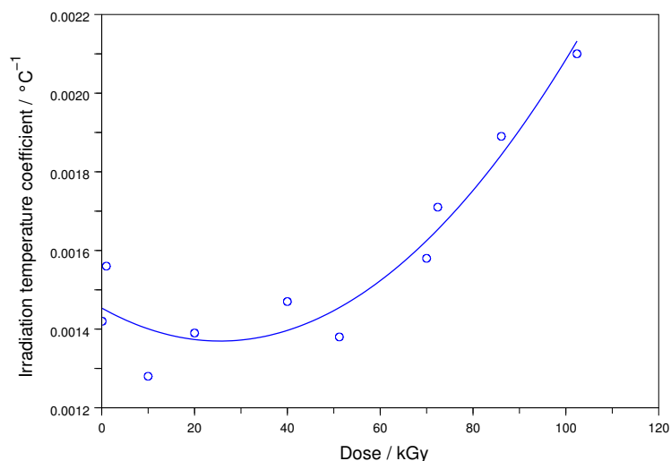
Figure 1: Alanine dosimeter irradiation temperature coefficient as a function of absorbed dose.
