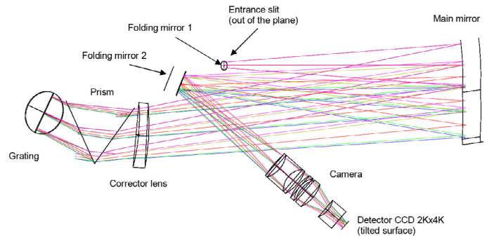
Fig. 5. The UVB spectrograph optical layout. The optical layout of the VIS spectrograph is very similar to this one.
