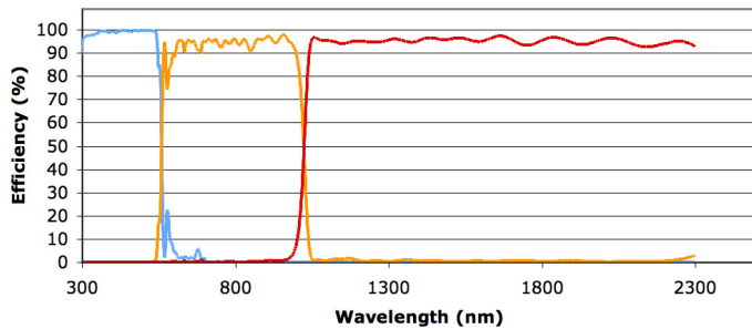
Fig. 4. The combined efficiency of the two dichroic beam splitters. In blue: reflection on the first dichroic; in orange: transmission through the first dichroic and reflection on the second dichroic; in red: transmission through both dichroics.
