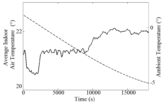
Fig. 13. Average of indoor air temperatures of all households (solid line) and sinusoidal ambient temperature (according to Chapter II.B) (dashed line) during the investigated 5 hours.
