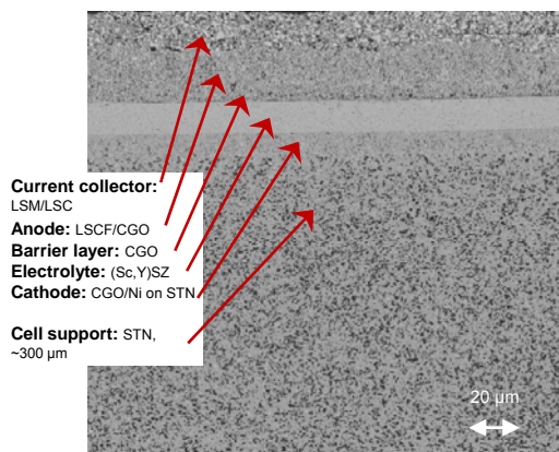
Figure 1: SOE-cell design
