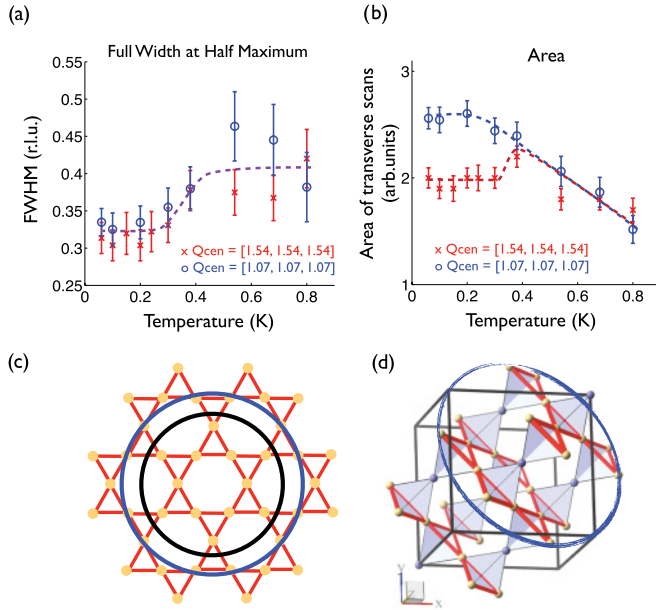
FIG. 3. (Color online) (a) Full width at half maxima (FWHM) and (b) integrated area extracted from the Lorentzian fits to the transverse scans shown in Fig. 2(a). (c) The range of \xi_T within the kagome layer. Above 400 mK (black), the correlations are restricted to a single kagome star unit. Below 265 mK (blue), the transverse correlations grow only to encompass the next-near neighbors in the kagome layer. (d) The pyrochlore lattice decomposed into kagome and interleaved triangular layers. Below 400 mK, the longitudinal correlations extend only between a single KTK unit.
