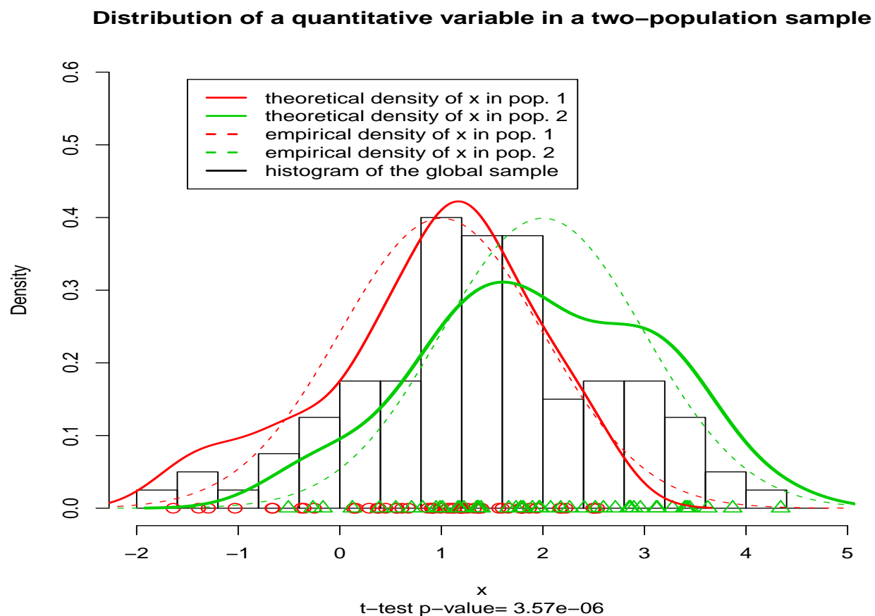
Figure 8: Synthetic example of a variable measured in two populations with mean equal to 1 and 2 respectively and a common unit variance. The global histogram (black) seems unimodal and does not suggest the presence of two populations, the numerical values from the two population overlap substantially. Any algorithm aimed at clustering the individuals would be subject to a large error rate. However, the p-value of a classical t-test is highly significant.
