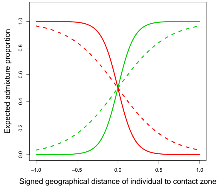
Figure 5: Examples of spatial variation of expected admixture proportions in presence of two clusters. Individuals whose proportions are displayed here are assumed to be continuously located along a linear transect crossing perpendicularly a hybrid zone. Red line: expected admixture proportion q_{i1} , green line: expected admixture proportion q_{i2} . Continuous lines: a = 1 , b = 0.1 , dashed lines: a = 1 , b = 0.3 . Note that the curves are exactly sigmoid (logistic) functions.
