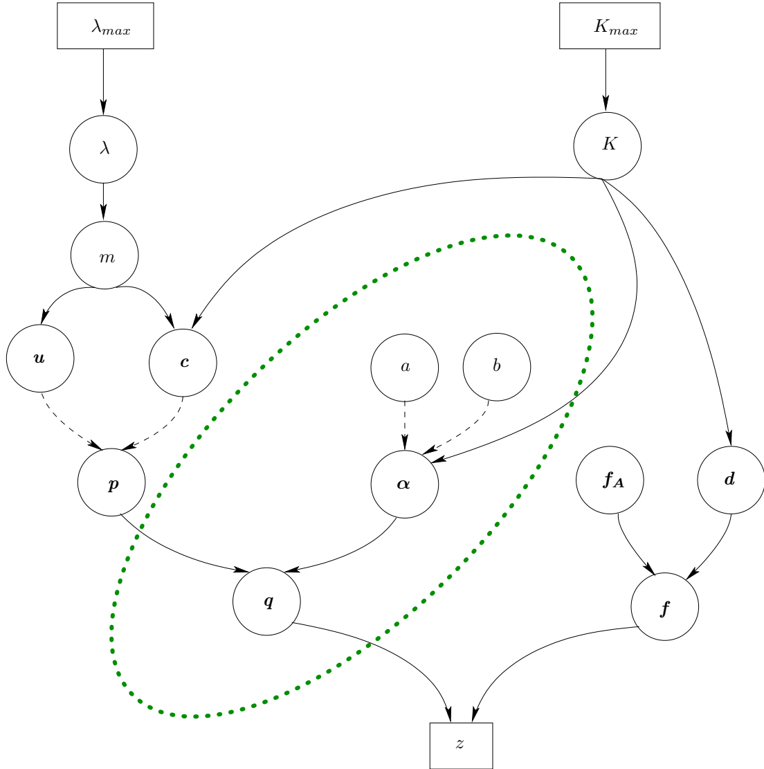
Figure 6: Directed acyclic graph of the model(s) implemented in GENELAND. Continuous lines represent stochastic dependencies, dashed lines represent deterministic dependencies. Squared boxes enclose data or fixed hyper-parameters, rounded boxes enclose inferred parameters. The thick green dotted line enclose parameters of the admixture model.
