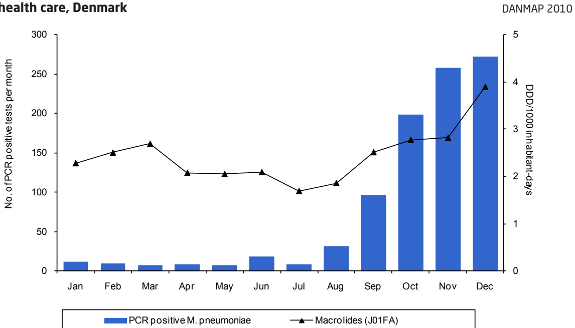
Figure 5.11. Monthly consumption of macrolides and PCR positive Mycoplasma pneumoniae tests in primary health care, Denmark
