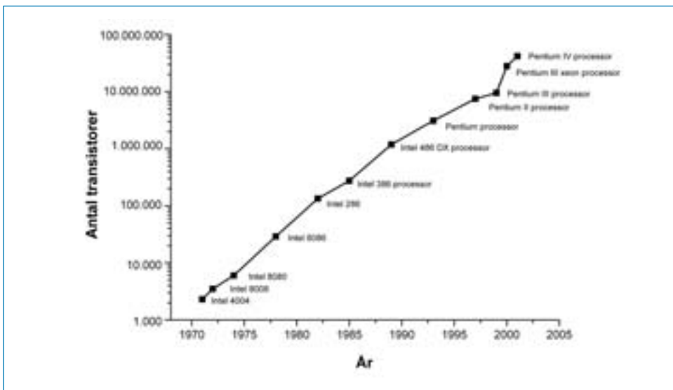
Figur 1. Moores lov
