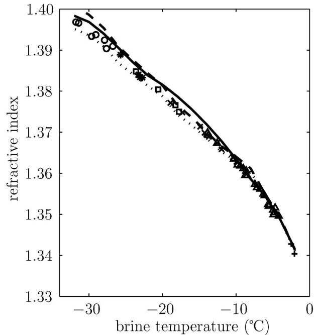
Fig. 1. Refractive index at 589 nm of brine in freezing equilibrium as measured by Maykut and Light [3]. Samples from six solutions are plotted; each solution has its own symbol. The three curves are the values predicted by the Lorentz–Lorenz relation with the density measured by Maykut and Light [3] (solid curve), Thompson and Nelson [7] (dotted curve), and Thompson and Nelson with a temperature correction (dashed curve).
