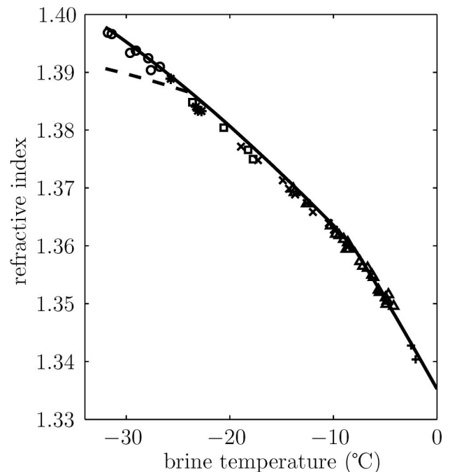
Fig. 3. Predicted refractive indices of brine in freezing equilibrium using the new extrapolation of Quan's and Fry's [1] formula (solid curve) as compared to measurements of Maykut and Light [3]. The dashed curve is the result if we use the three-piece fit in Fig. 2 instead of the two-piece fit.
