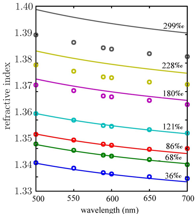
Fig. 5. (Color online) Predicted refractive indices at different wavelengths of nonequilibrium, freezing brine as compared to measurements of Maykut and Light [3]. In this figure, the curves have not been corrected.
