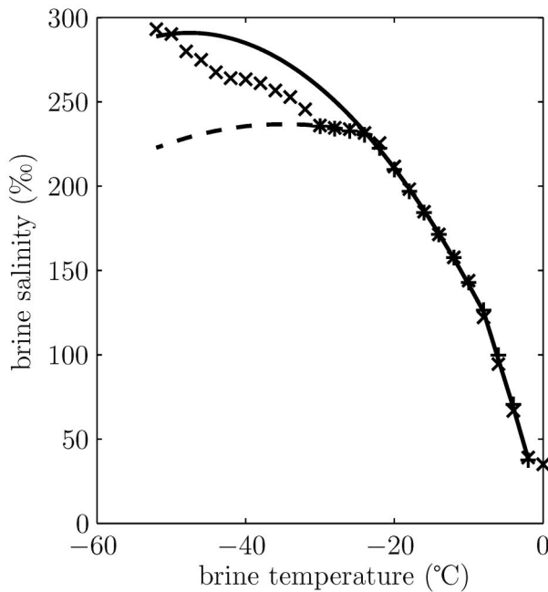
Fig. 2. Salinity of brine in freezing equilibrium as a function of temperature. Data samples measured by (+) Assur [8] and (x) Richardson [4]. The solid curve is a two-piece, parabolic, least-squares fit to the measurements from -2 °C to -8 °C and from -8 °C to -24 °C. The dashed curve is a third piece fitted to the measurements from -24 °C to -32 °C.
