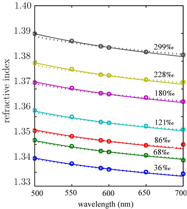
Fig. 4. (Color online) Predicted refractive indices at different wavelengths of nonequilibrium, freezing brine as compared to measurements of Maykut and Light [3]. The solid curve extrapolates the formula by Quan and Fry [1]; the dotted curve uses the Lorentz-Lorenz relation. To explicitly check the ability to predict wavelength dependency of the refractive index, the curves have been corrected to meet the measurements at \lambda = 589 nm.
