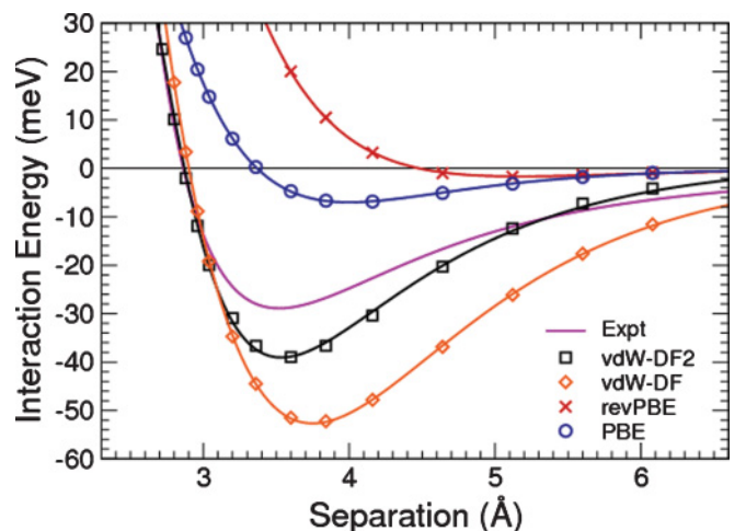
FIG. 1. (Color online) Experimentally determined effective physisorption potential for H 2 on Cu(111), 3 compared with potential-energy curves for H 2 on Cu(111), calculated for the atop site using GGA-revPBE, GGA-PBE, vdW-DF2, and vdW-DF.
