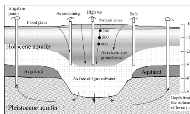
Figure 1. Schematic model of arsenic contaminated groundwater formation in a recharge zone of Sonargaon, Bangladesh. Attached figure on dot gives concentration of Arsenic in the pore water in mg/L. Arrows indicate groundwater flow direction.
