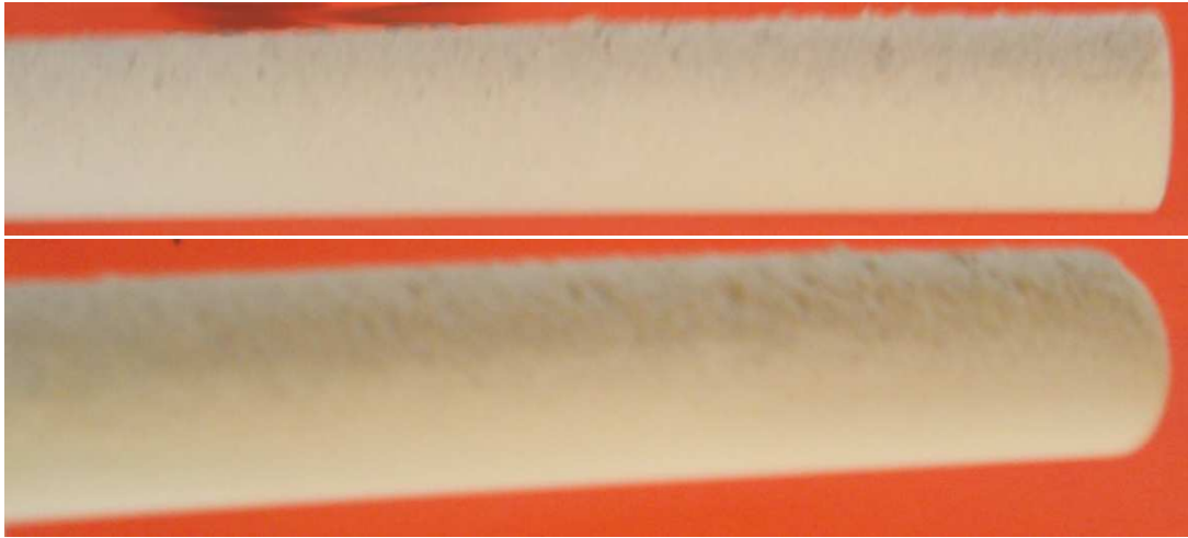
Figure 3.13: View of deposits from the side. The deposit probe has a diameter of 16 mm and the thickness of the upstream deposits is about 1 mm. Top: coal/air combustion; Bottom: coal/oxyfuel combustion. The upstream part of the probe faces upwards in the picture. Colour differences are a consequence of the picture recording.
