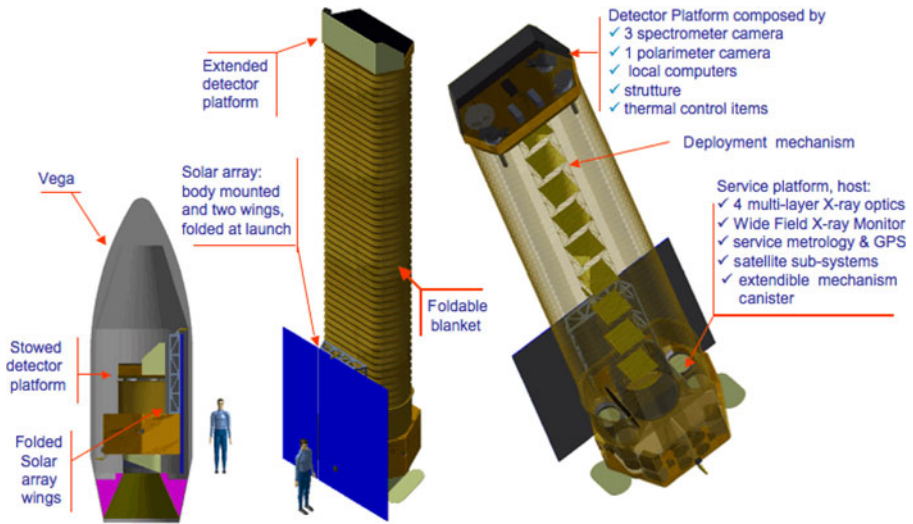
Fig. 16 NXM in the stowed and deployed position
