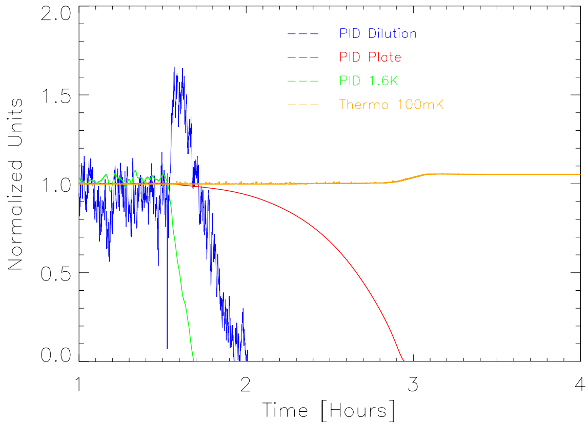
Fig. 19. Thermal behaviour of the 100 mK stage during the 4 K shutdown on 6 August 2009. The vibration level of the 4 K propagated to the dilution is measured from the step in the blue curve (signal of the active regulation of the dilution) after the rapid drop of the 4 K. It is equal to 26 nW.
