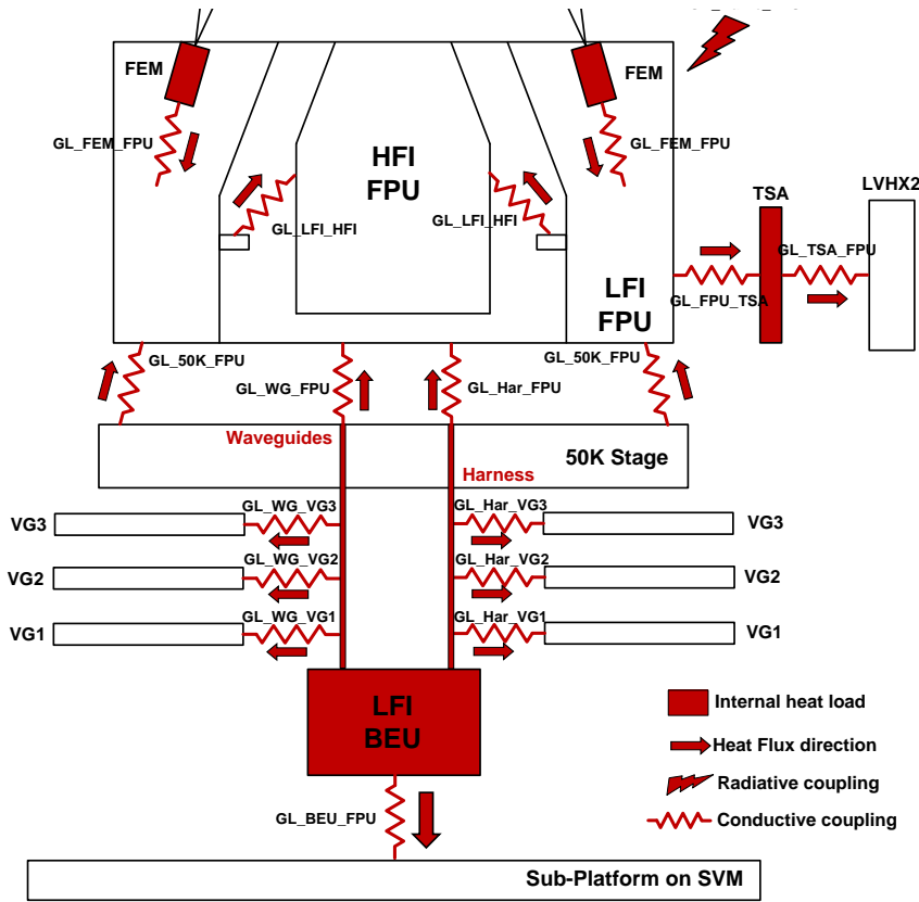
Fig. 14. Principal heatflows for the LFI.
