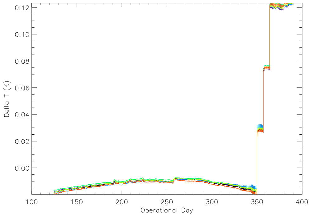
Fig. 34. Temperature from LFI focal plane sensors TSL1 to TSL6 in the period from 125 to 389 days after launch. Until intentional changes in TSA setpoint started around day 350, the temperature shows only a slow drift correlated with distance from the Sun. See also Fig. 37
