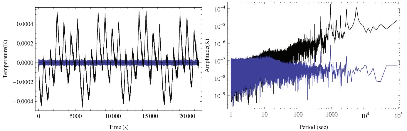
Fig. 24. Daily behaviour of temperatures in the HFI outer shield in October 2009, left, and corresponding Fourier transform amplitude, right. Black: 4KL1 sensor (close to 30 and 44 GHz loads); Blue: PIDN sensor (close to 70 GHz loads).
