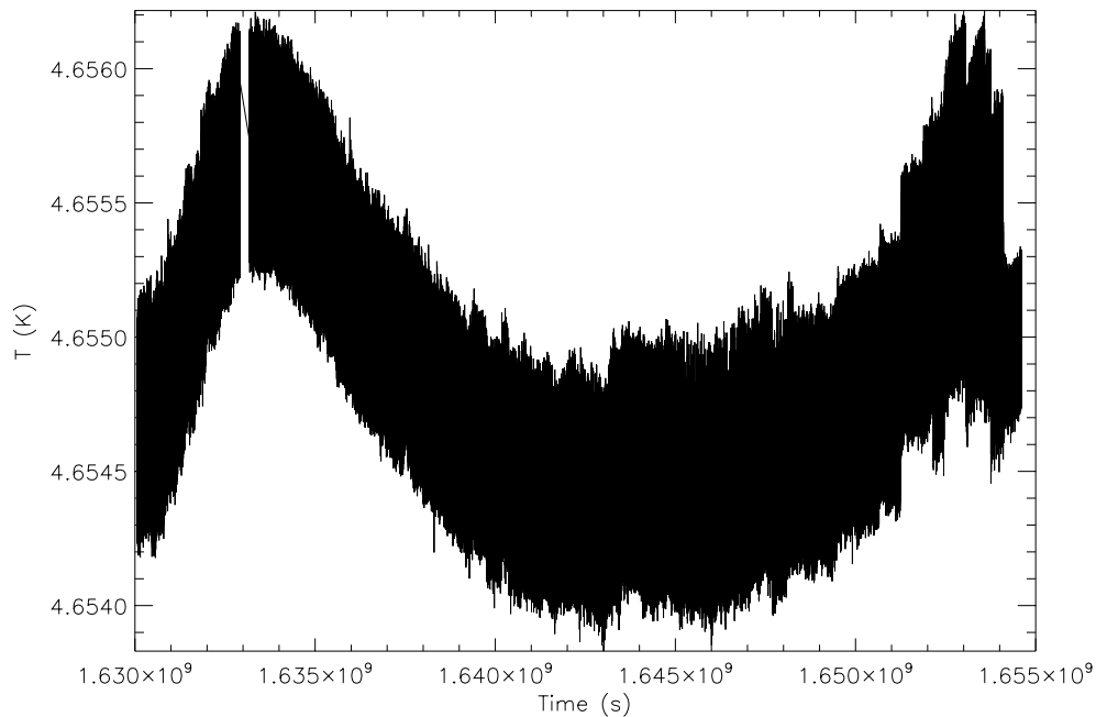
Fig. 36. Temperature curve of the HFI L1 sensor close to 30 GHz reference load, since the beginning of the first sky survey up to OD 389.
