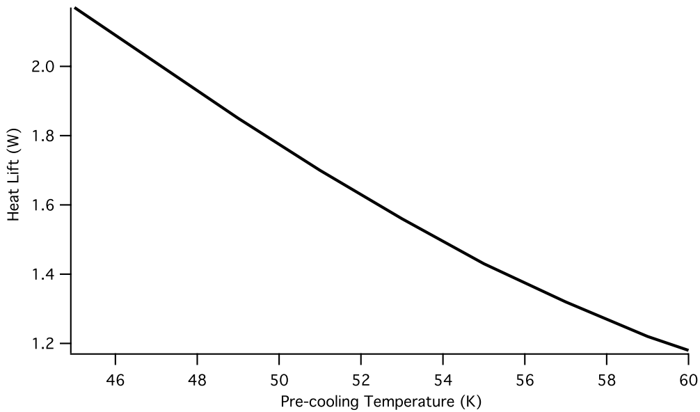
Fig. 11. Heat lift of the sorption cooler as a function of precool (V-groove 3) temperature.
