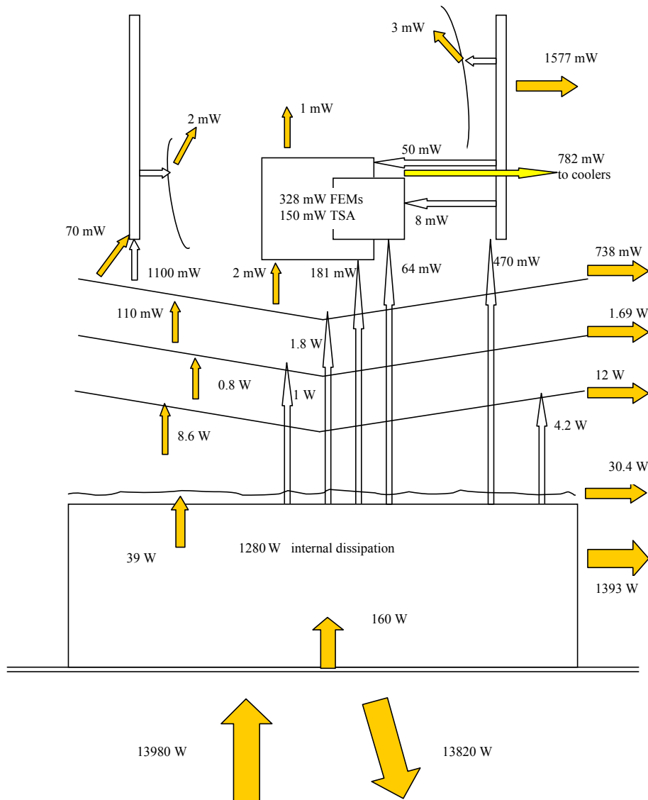
Fig. 13. Principal heatflows for Planck . Nearly 14 kW is incident on the solar panel, but less than 1 W reaches the FPU. Passive radiative cooling and thermal isolation are the keys to the overall thermal performance. Yellow arrows indicate radiation. White arrows indicate conduction.
