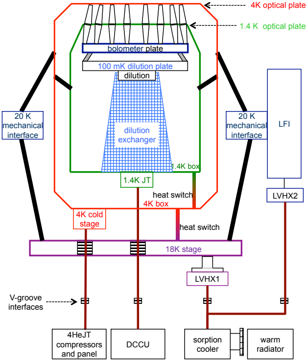
Fig. 5. Schematic of the HFI FPU. The designations “20 K”, “18 K”, “4 K”, “1.4 K”, and “100 mK” are nominal. Actual operating temperatures are given in § 4.
