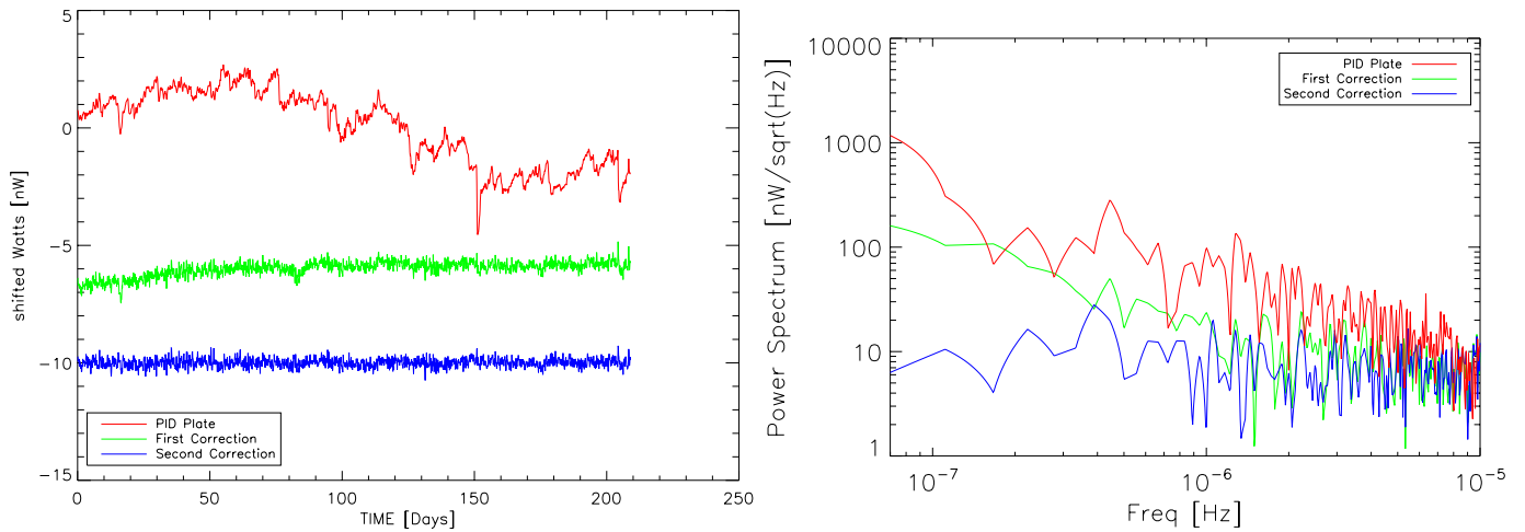
Fig. 30. Correction of the signal of the active regulation of the temperature of the bolometer plate stage with the SREM (first correction in green) signal and the active regulation of the dilution stage (second correction in blue) in time domain (left) and frequency domain (right).
