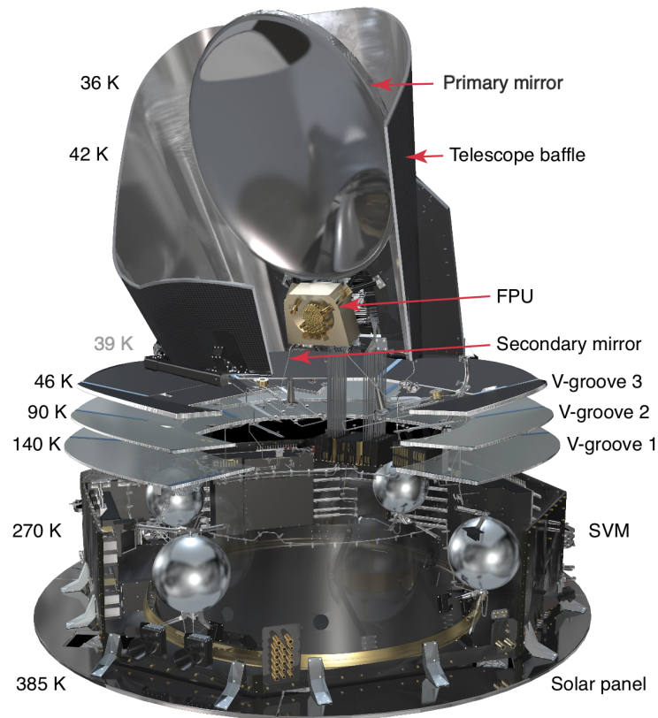
Fig. 1. Cutaway view of Planck showing the temperature of key components. The solar panel at the bottom always faces the Sun and the Earth, and is the only part of the flight system illuminated by the Sun, the Earth, and the Moon. Temperature decreases steadily towards the telescope end, due to low-conductivity mechanical connections and aggressive use of radiative cooling. The focal plane detectors are actively cooled to 20 K and 0.1 K.
