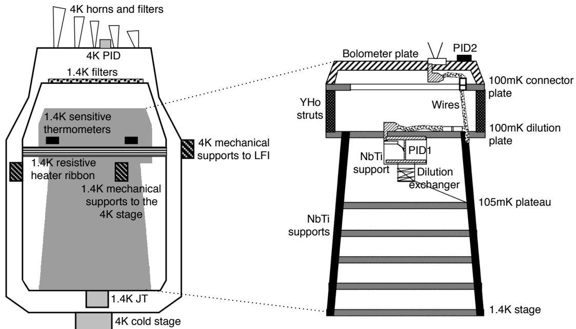
Fig. 10. Thermal control architecture of the 4 K and 1.4 K stages ( left ) and the 0.1 K stage ( right ).
