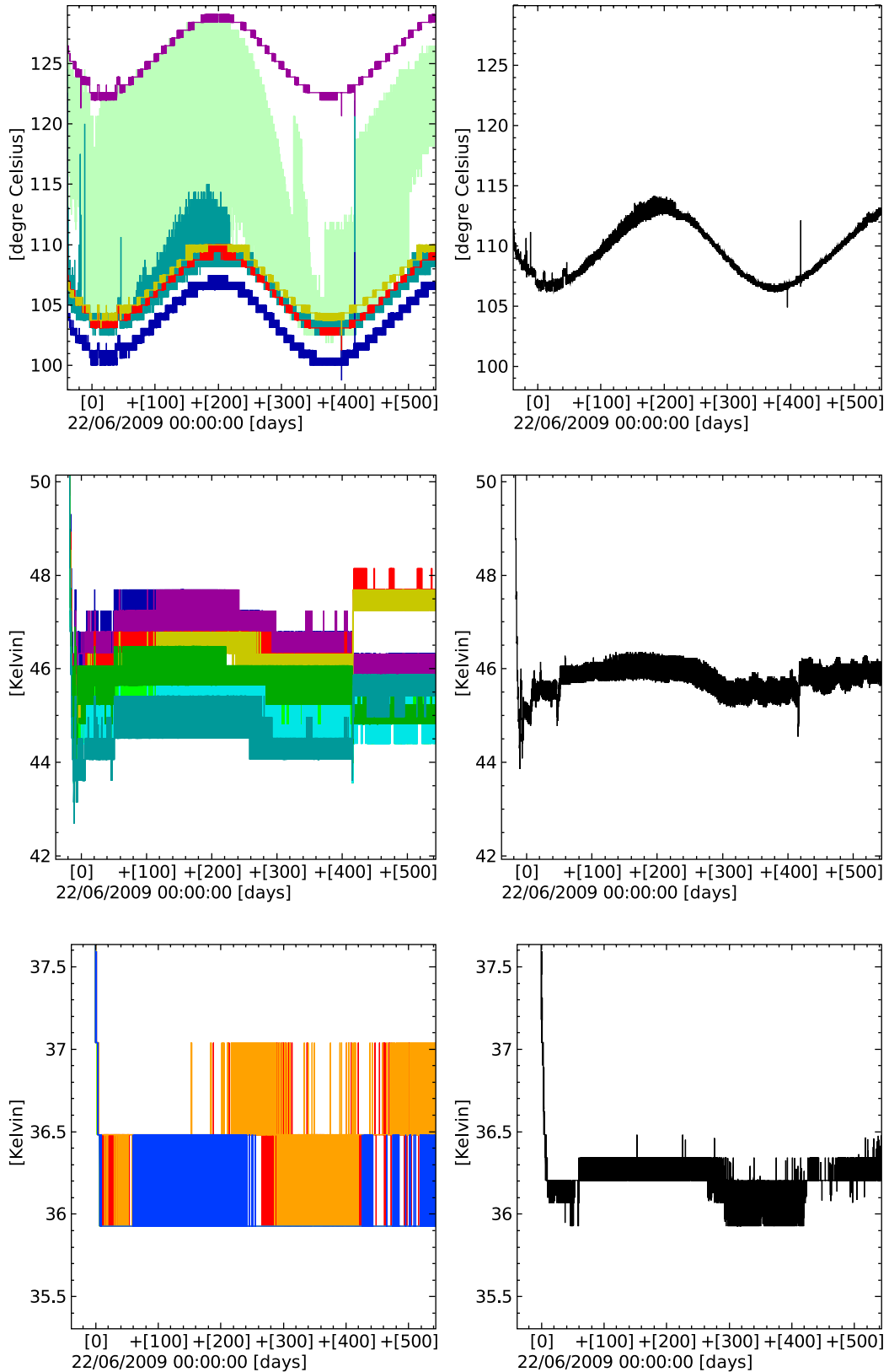
Fig. 37. Seasonal variation in the temperature of the solar panel ( top ), V-groove 3 ( middle ), and the primary mirror ( bottom ). Individual readings are shown for multiple temperature sensors on each part of the structure ( left, all three panels ). Quantization effects are clearly visible for V-groove 3 and the primary mirror. These are reduced but not eliminated by averaging the relevant sensors ( black line in all three panels ).
