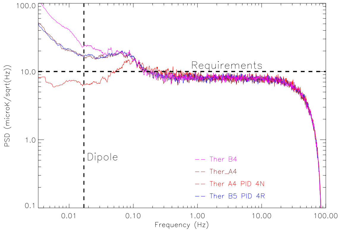
Fig. 27. Power spectrum of thermal fluctuations measured at the feedhorns that couple to the telescope.
