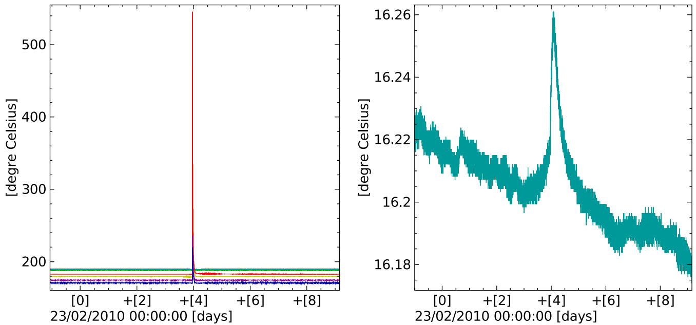
Fig. 8. Temperatures of the 20 N thrusters (left) and the 4 He tank (right).
