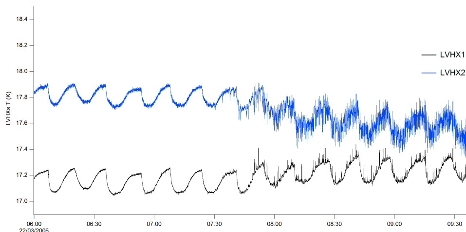
Fig. 38. Temperature fluctuations for two different operating regimes of the sorption cooler cold end. On the left the cold end is in a balanced state and the liquid interface is inside the LVHX2 body. On the right the cold end is in an unbalanced state and the liquid interface moves into the counterflow heat exchanger beyond the LVHX2 body. The flow becomes erratic because of plug-flow events.
