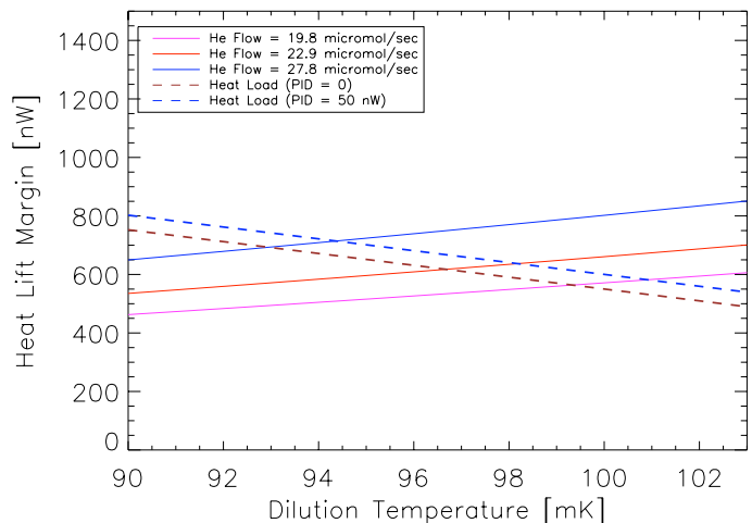
Fig. 7. Heat lift margin of the dilution cooler as a function of dilution temperature and helium flow, with the dilution cooler control unit at 19 °C. For operation in flight at 101 mK, 115 nW is available to accommodate the heating from cosmic rays and for temperature regulation even at the lowest flow (Fmin2 = 19.8 \mu\text{mol s}^{-1} ) which is the flight configuration.
