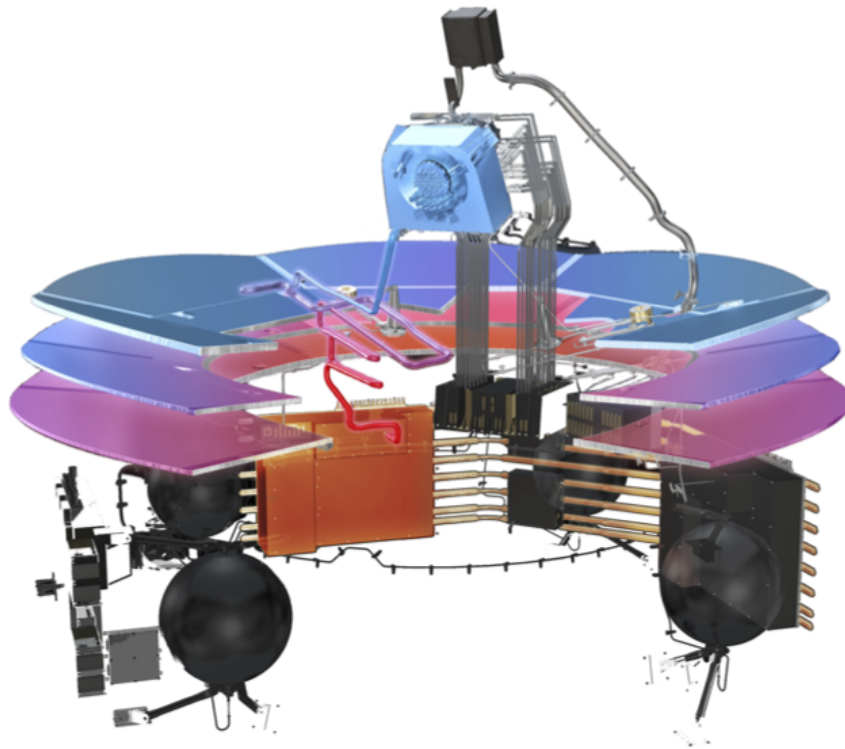
Fig. 2. Sorption cooler system. The system is fully redundant. The orange box houses one of the compressor assemblies, mounted on one of the warm radiator panels, which faces cold space. Heat pipes run horizontally connecting the radiators on three sides of the service vehicle octagon. The second compressor assembly is the black box on the right. A tube-in-tube heat exchanger carries the high and low pressure hydrogen gas from the compressor assembly to the focal plane assembly, with heat-exchanging attachments to each of the three V-grooves. The colors indicate temperature, from warm (red, orange) to cold (blue).
