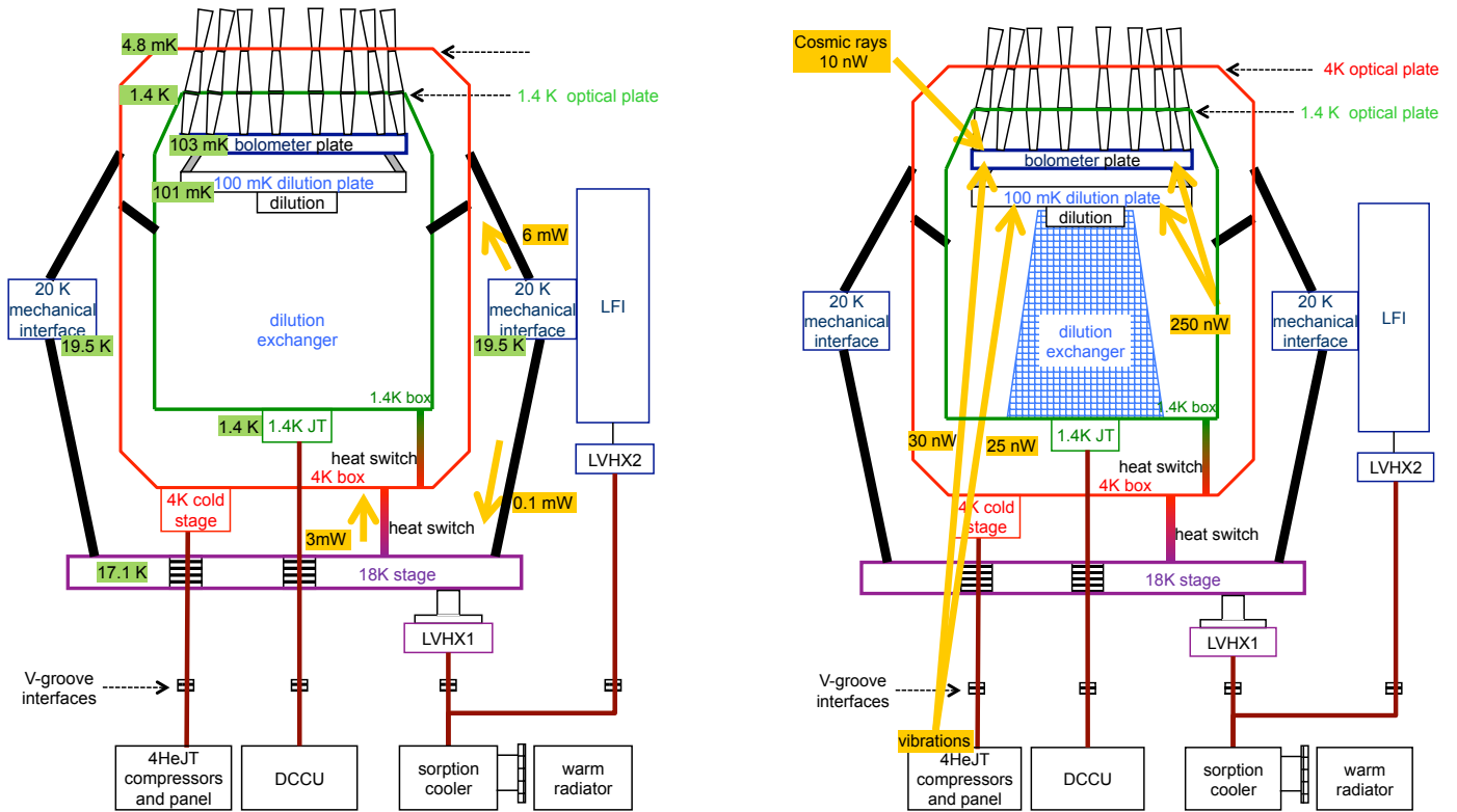
Fig. 15. Principal heatflows for the HFI “4 K” system (left) and dilution system (right).
