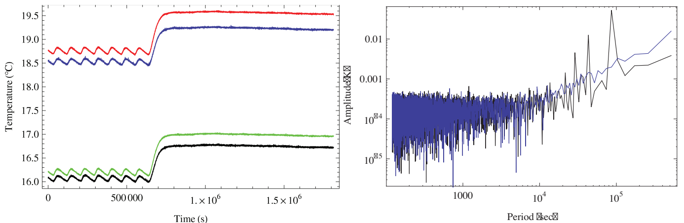
Fig. 26. Left plot: LFI backend temperatures (black: Left BEM1 sensor, blue: Left BEM2 sensor, red: Right BEM1 sensor, green: Right BEM2 sensor) around operational day (OD) 258 of flight operations, when the transition to an always-on condition for the transponder was implemented. Right plot: comparison of the Fourier transform amplitude of the Left BEM1 sensor before (black) and after (blue) transition to stable, showing the daily time scale peaks disappearing.
