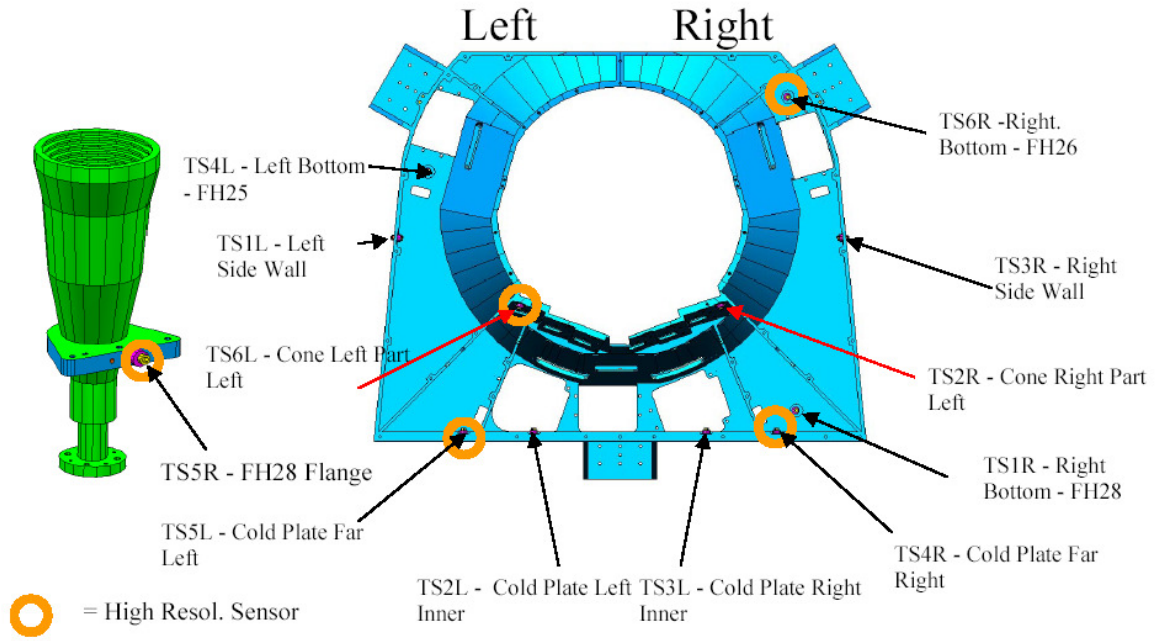
Fig. 32. Location of temperature sensors in the LFI focal plane.
