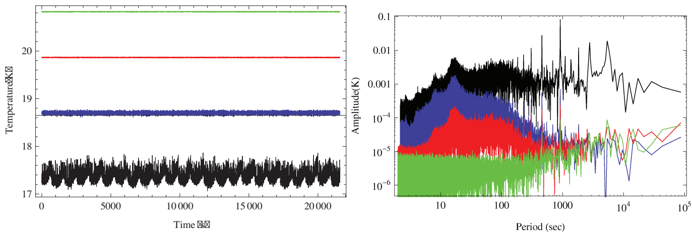
Fig. 21. LFI temperatures, left, and corresponding spectra, right, in October 2009. Black: LVHX2; Blue: TSA, Red: TSR1 (focal plane sensor closest to LVHX2), Green: TSL6 (focal plane sensor farthest from LVHX2).
