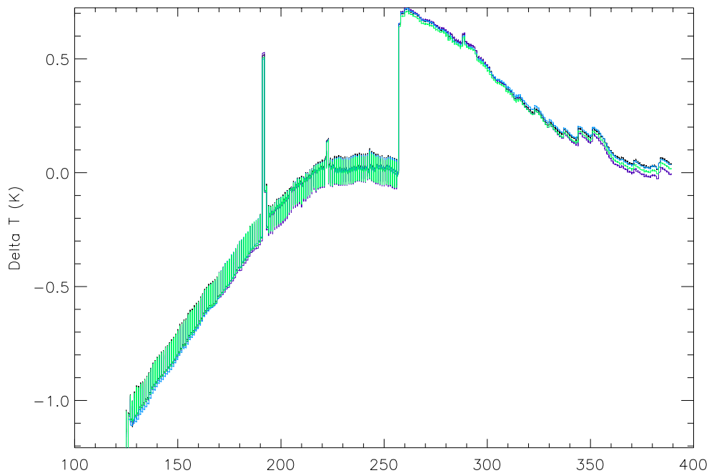
Fig. 35. Temperature of the LFI backend sensors (left back end block sensors) in the period going from 125 to 389 days after launch. Until day 260, the transponder was on only during downlinks. This approximately diurnal variation drove a large periodic variation in temperature. After day 260, the transponder was left on continuously, and the daily temperature variations became much smaller.
