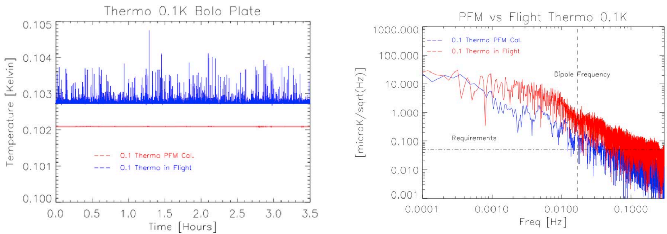
Fig. 31. Comparison of the signal of the thermometer of the bolometer plate stage between ground calibration and flight in time domain (left) and in frequency domain (right). The requirements are calculated for one bolometer.
