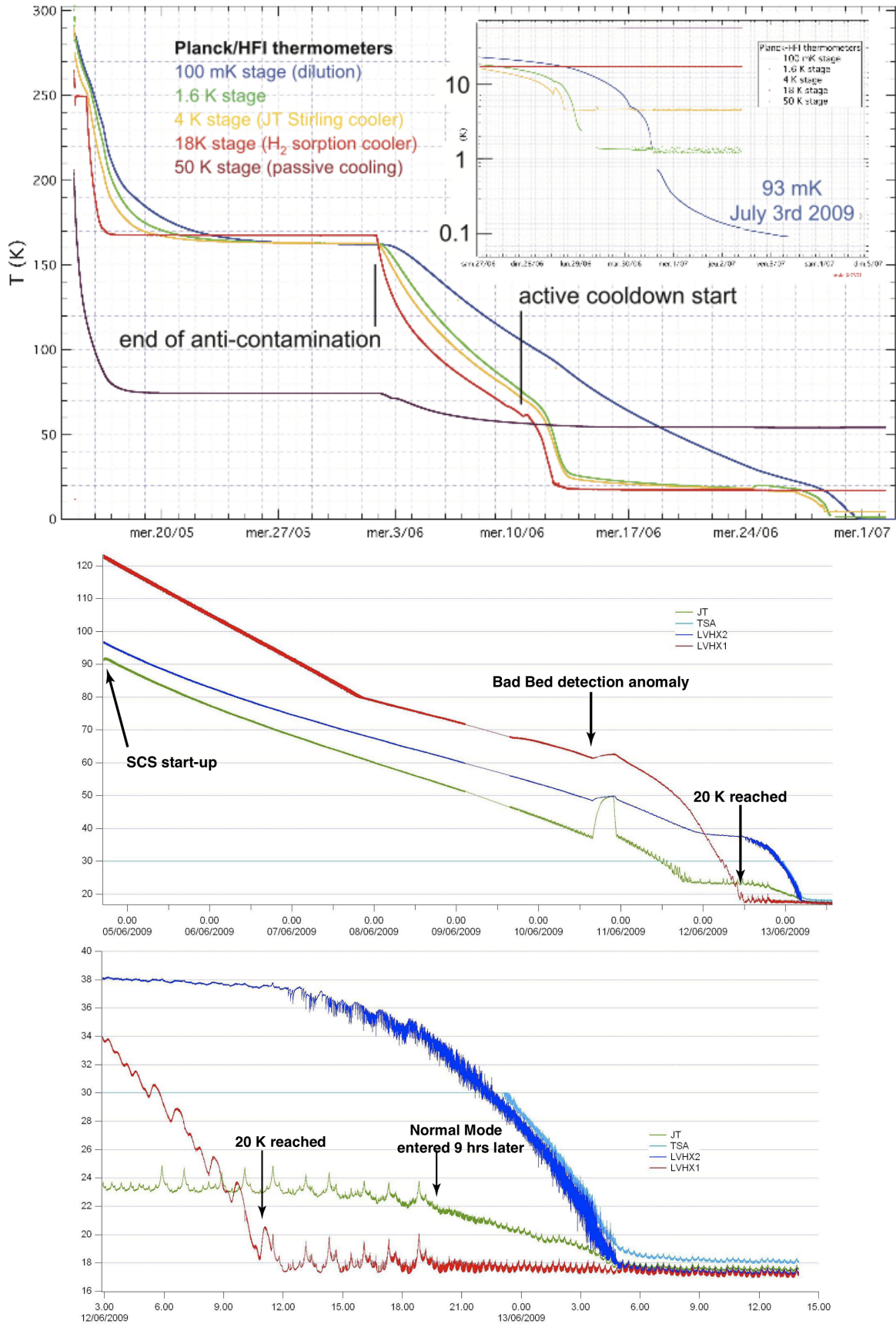
Fig. 16. Top: Initial cooldown of Planck , starting from launch on 14 May 2009 and concluding on 3 July 2009, when the bolometer plate reached 93 mK. The inset above shows the last week of the HFI cooldown. Middle: Expanded view of the LFI cooldown from sorption cooler start-up on 5 June 2009 until 13 June 2009. Bottom: Last day of the sorption cooler cooldown.
