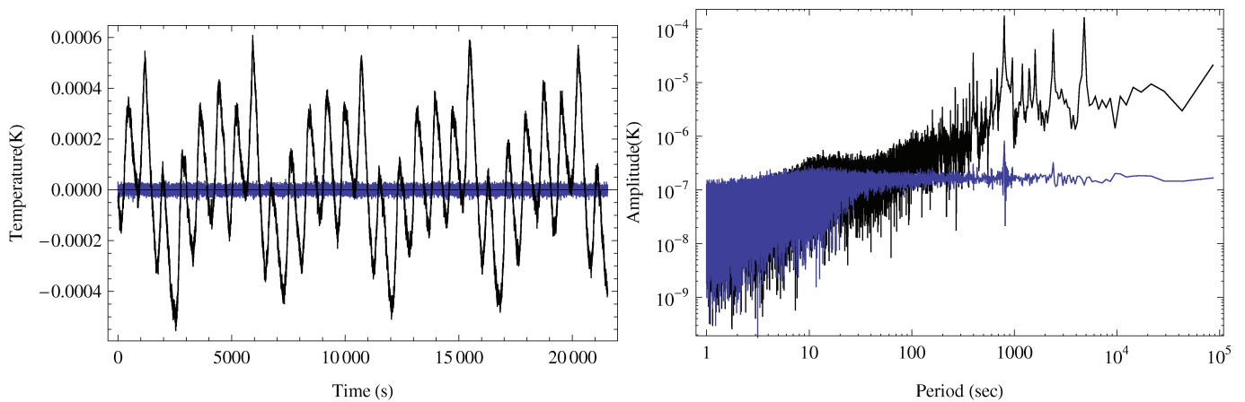
Fig. 25. Daily behaviour of temperatures in the HFI outer shield in May 2010, left, and corresponding Fourier transform amplitude, right. Black: 4KL1 sensor (close to 30 and 44 GHz loads); Blue: PIDN sensor (close to 70 GHz loads).
