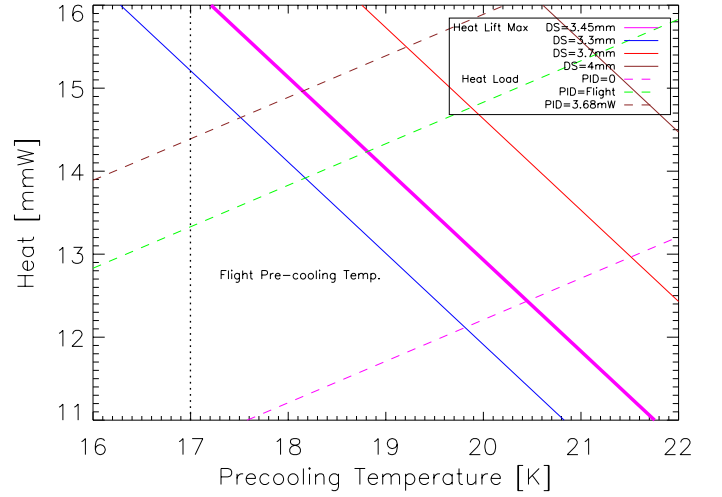
Fig. 6. Heat lift of the ^4\text{He} -JT cooler as a function of precool temperature, stroke amplitude \Delta S , and proportional, integral, differential (PID) control power. For \Delta S = 3.45 mm, a pre-cool temperature of 19.5 K gives the minimum required heat lift (Table 2) of 13.3 mW. The in-flight precool temperature of \sim 17.0 K (vertical dotted line, and Table 10) allows the use of a low stroke amplitude, minimising stresses on the cooler, and provides a large margin in heat lift.
