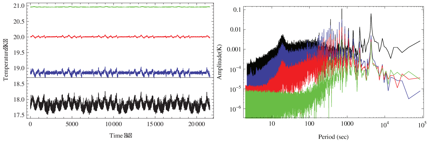
Fig. 22. LFI focal plane temperatures, left, and corresponding Fourier transform amplitude, right, in May 2010. Black: LVHX2; Blue: TSA, Red: TSR1, Green: TSL6.
