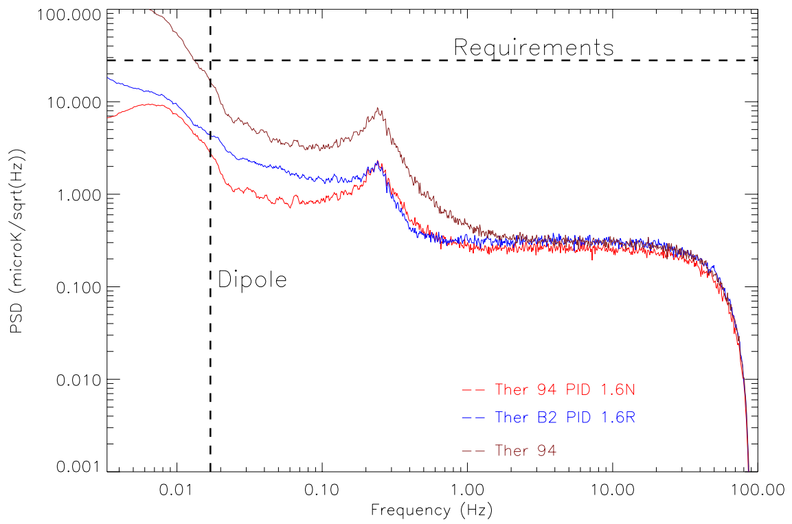
Fig. 28. Power spectrum of thermal fluctuations measured at the 1.4 K filter plate.
