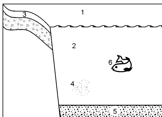
Figure 2a: A Mackay level 1 distribution model (numbers indicate the six different compartments usually included in Mackay level 1 models).
