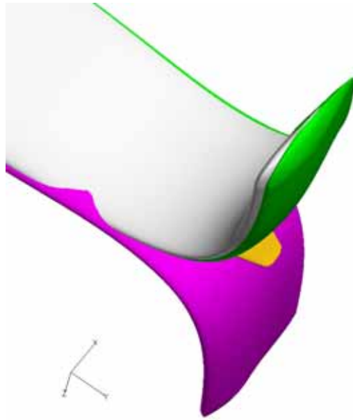
Figure 3: wingle1 (green), wingle4 (white) and wingle5 (purple) compared to the original blade (orange)
