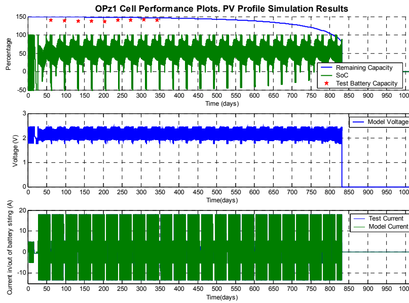
Figure 25 OPzS Battery PV Simulation Results
