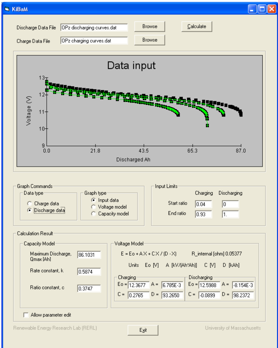
Figure 32 Voltage vs. Charge Removed for OPzS Battery
