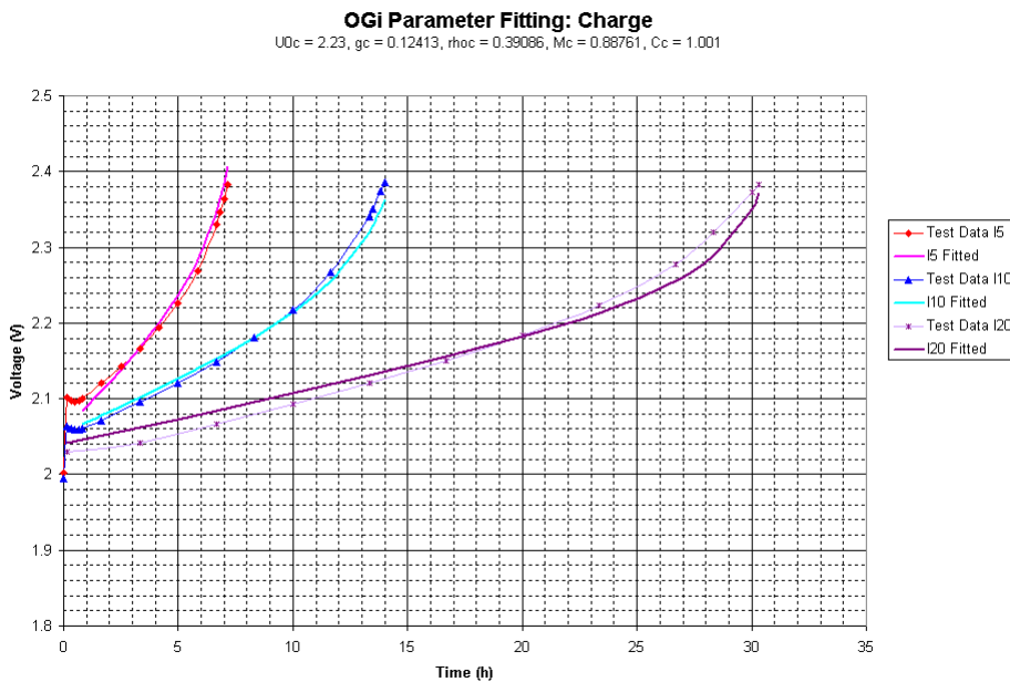
Figure 14 OGi Parameter Fitting: Charge
