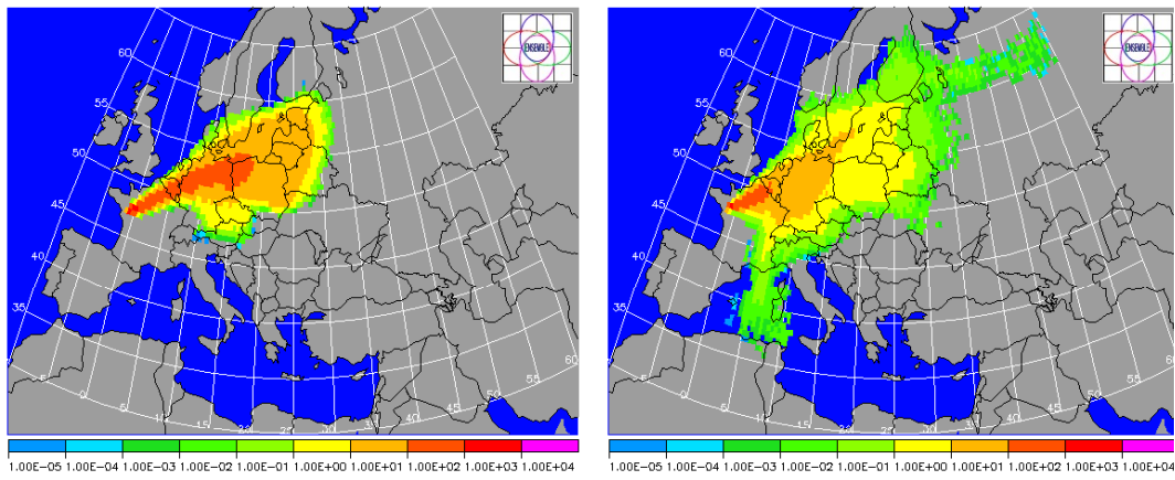
Figure 6-2. Plots of time integrated concentrations at about 60 hours after release for four models in Exercise 4 based upon analysed meteorology: United Kingdom (UKI – left); German (DEI – right).
