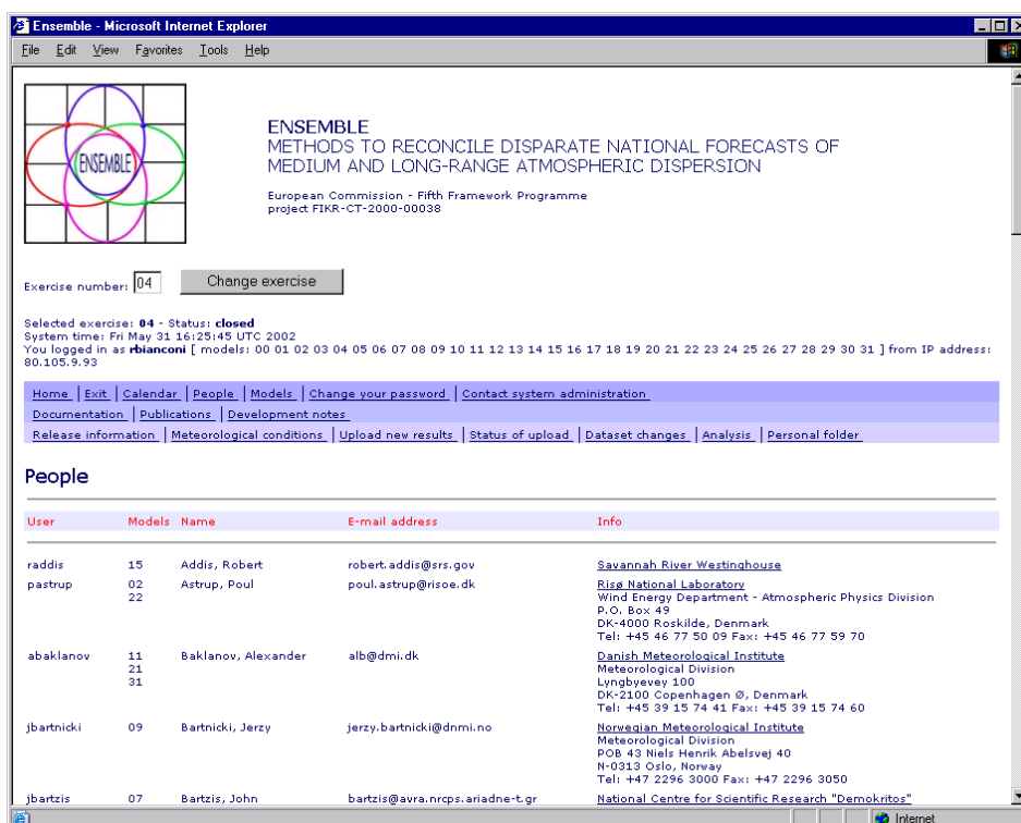
Figure 4-4 – “People” page.
