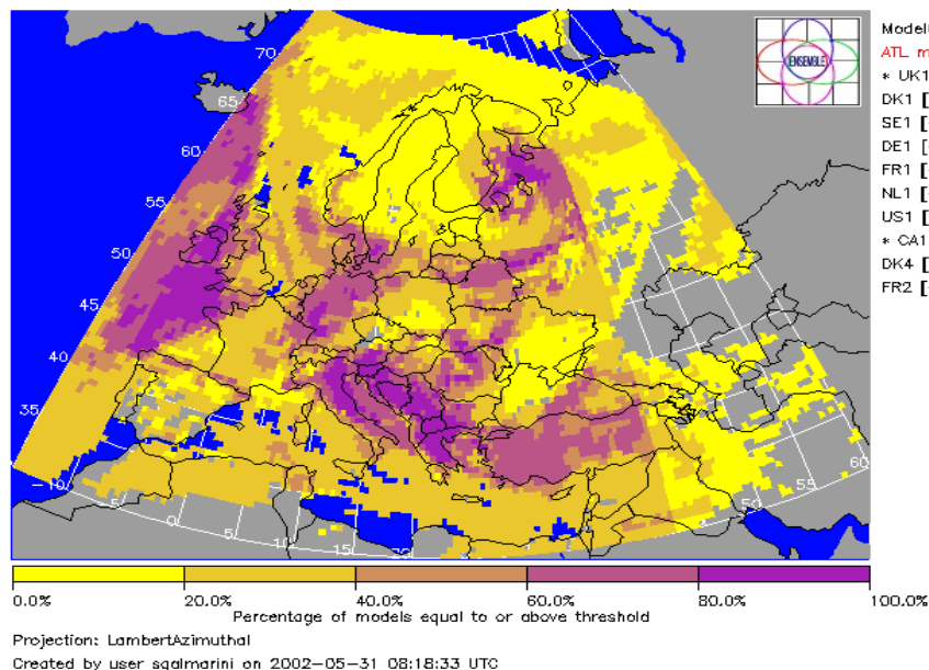
Figure 5-12. ATL for precipitation 51 h after release for exercise 05
