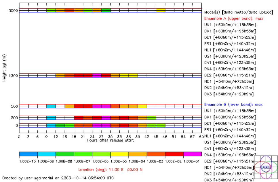
Figure 5-29. Time evolution of vertical profile of maximum 241 Pu at 11E 55N
