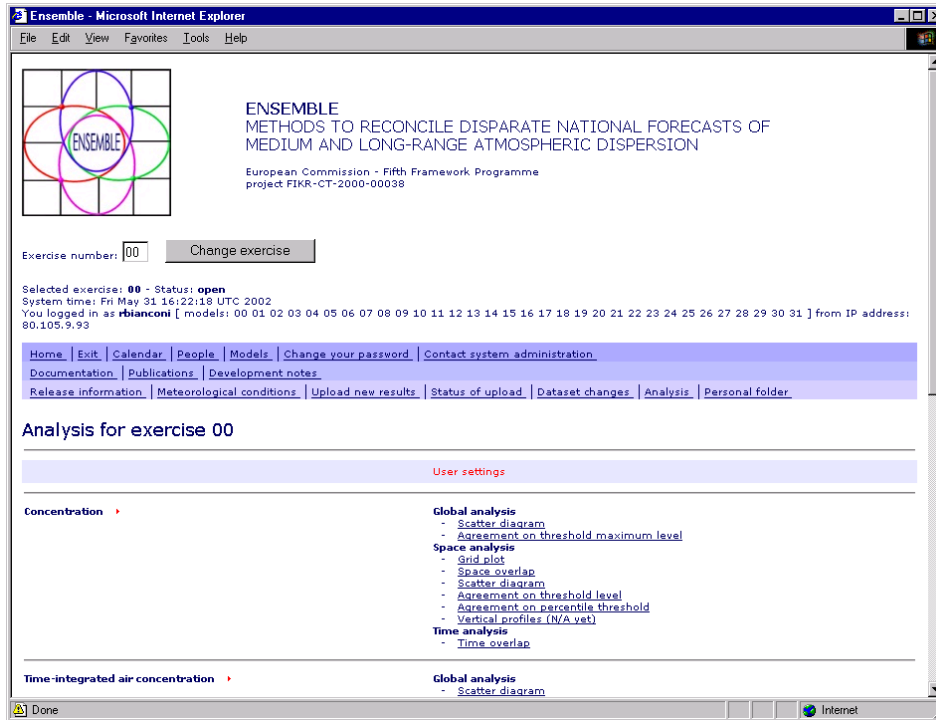
Figure 4-11 – “Analysis” page.
