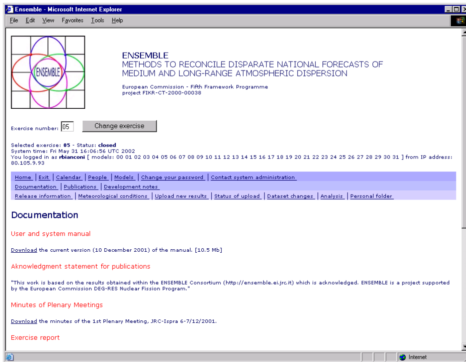
Figure 4-3 – “Documentation” page.
