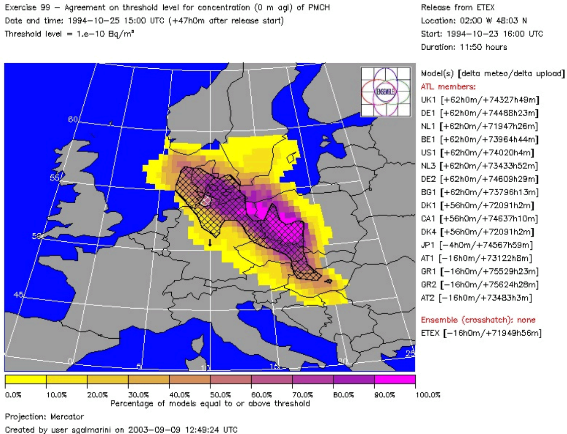
Figure 5-34. ENSEMBLE application to the ETEX case
