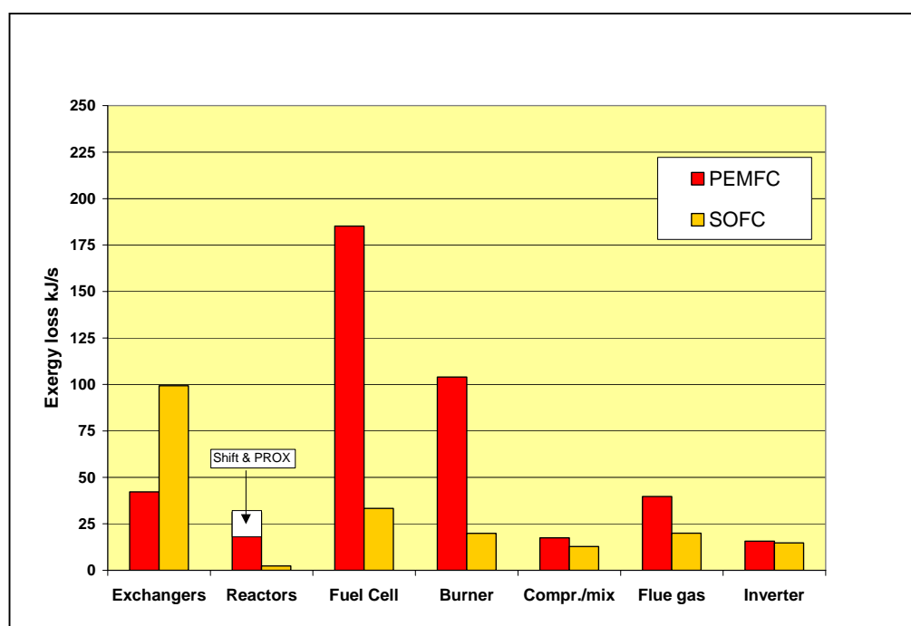
Figure 6. Comparison of exergy losses in PEMFC and SOFC 250 kW CHP systems
