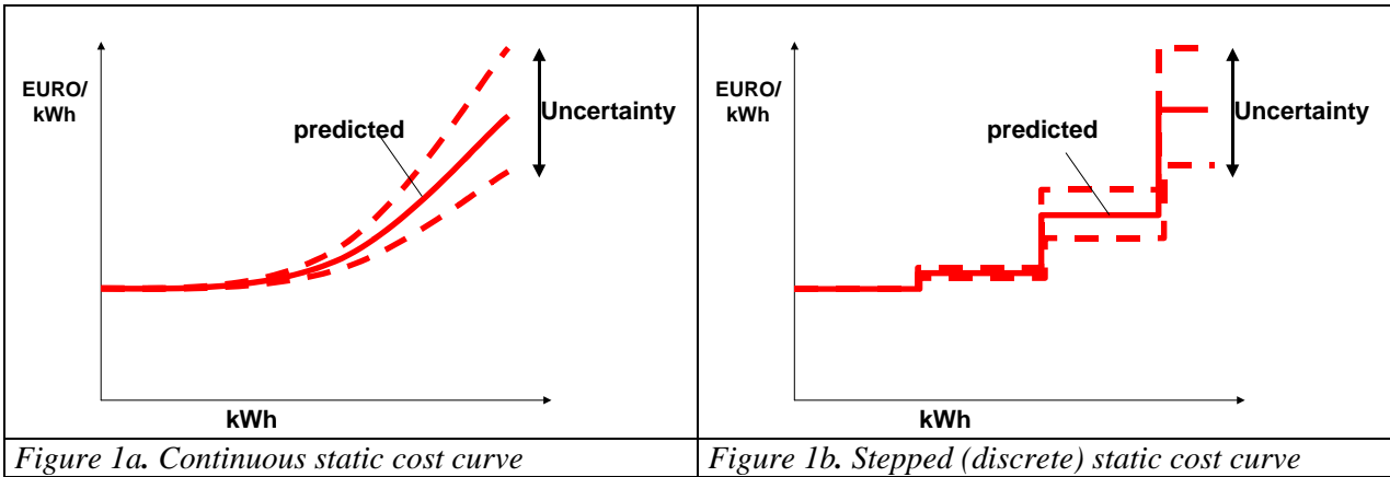
Figure 1a depicts the theoretically ideal continuous static cost curve taking into account that every location is slightly different from each other and, hence, looking at all locations e.g. for wind energy in a certain geographic area a continuous curve emerges after these potentials have been classified and sorted in a least cost way. Fig. 1b takes into account that in real life this accuracy is impossible. Different sites are put into certain categories and then a stepped curve emerges.
