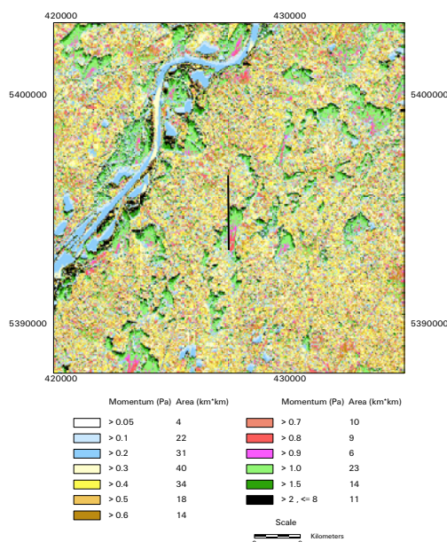
Momentum flux map for a wind speed of 5 m/s from North at 4 m height for summer 1993 based on Landsat TM.
