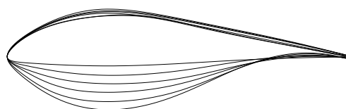
Figure 1 The contours of the Risø-A1 airfoil family.
