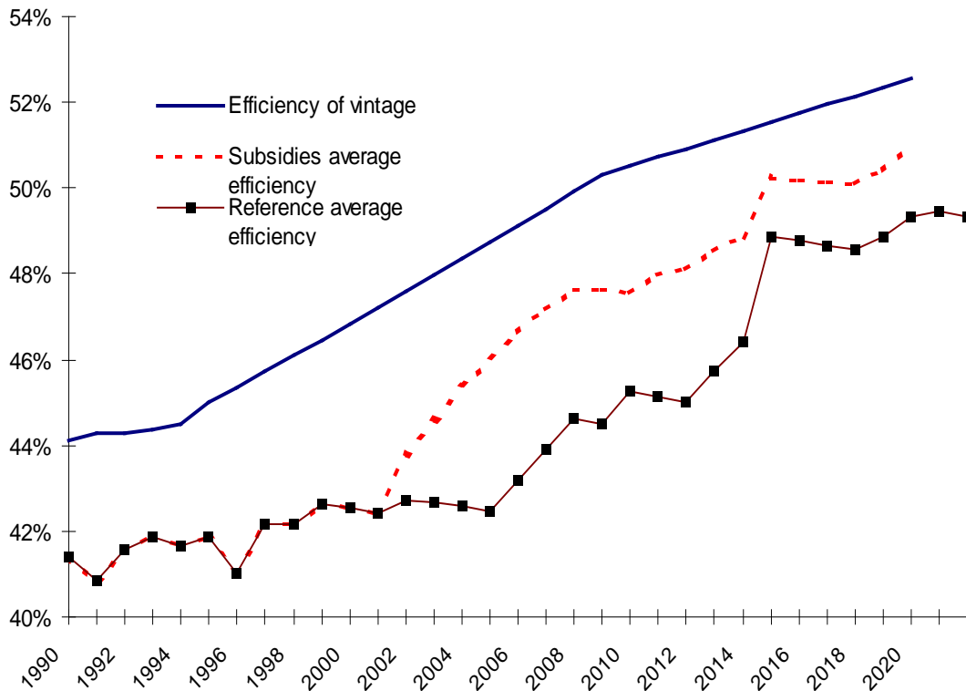
Figure 3 Fuel efficiency for major power plants in Denmark
