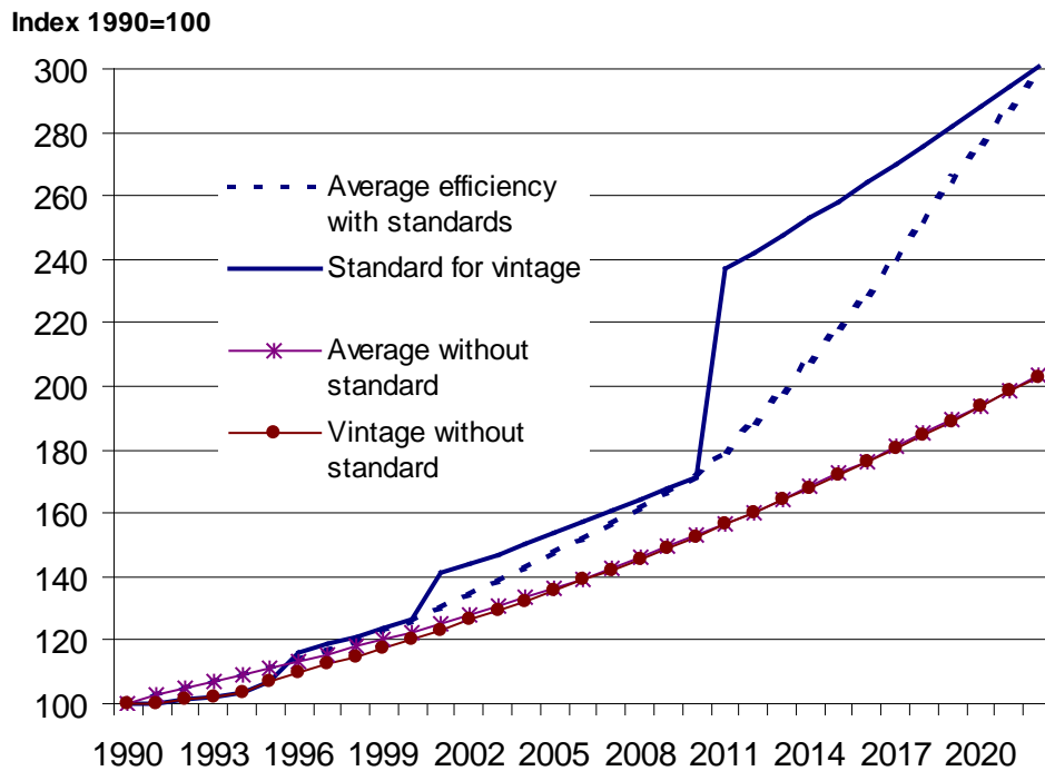
Figure 1 Efficiency developments for washing machine with and without standards.
