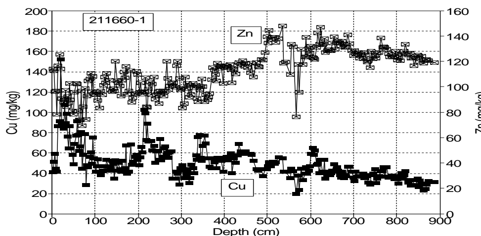
Fig. 19 Distributions of Ca and Mn (upper part of the figure) in the long piston core 211660-1 of the Gotland Basin based on sediment material from cubes that have been used for the paleomagnetic measurements. These data are re-plotted for the upper part of the core section (middle part of the figure) to show the alternating Ca-Mn peaks. Cu and Zn distributions are plotted in the lower part of the figure.
