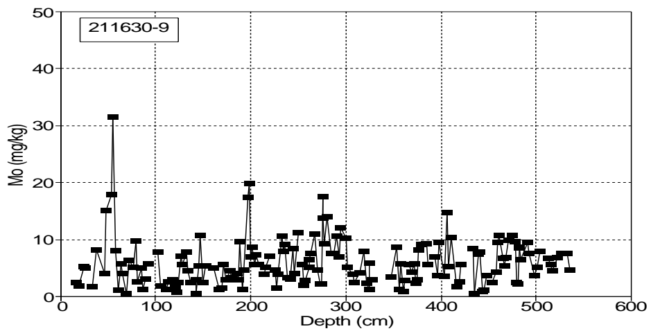
Fig. 15 Distributions of Zr, Br and Mo in the long core of the Bornholm Basin based on sediment material from cubes that have been used for the paleomagnetic measurements.
