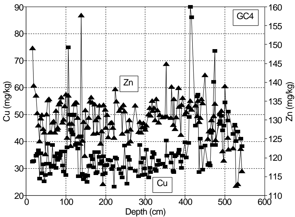
Fig. 24 Distributions of Ca and Mn (upper part of the figure) in the long gravity core GC4 of the North Central Basin based on sediment material from cubes that have been used for the paleomagnetic measurements. Cu and Zn distributions are plotted in the lower part of the figure.
