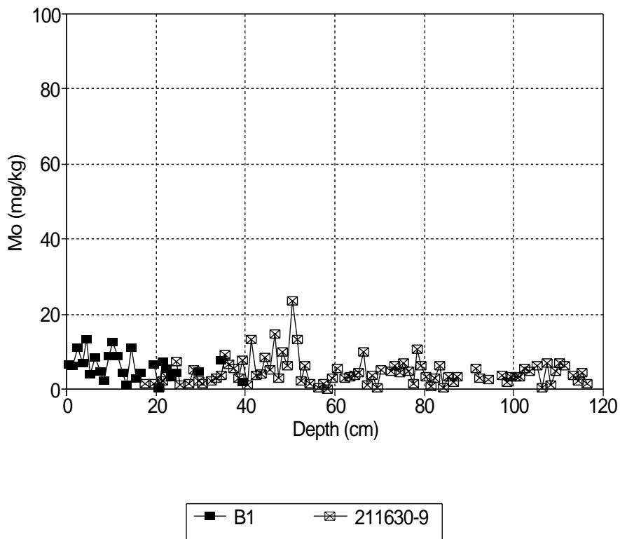
Fig. 13 Distribution of Br (upper part of figure) in the upper 1.2 m of the Bornholm Basin deep coring site constructed by using the short core B1 and the upper 1 m of core 211630-9. The distribution of Mo is shown in the lower part of the figure.
