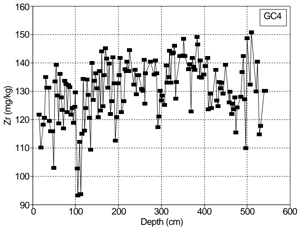
Fig. 25 Distributions of K and Zr along the gravity core GC4 of the North Central Basin based on sediment material from cubes that have been used for the paleomagnetic measurements.
