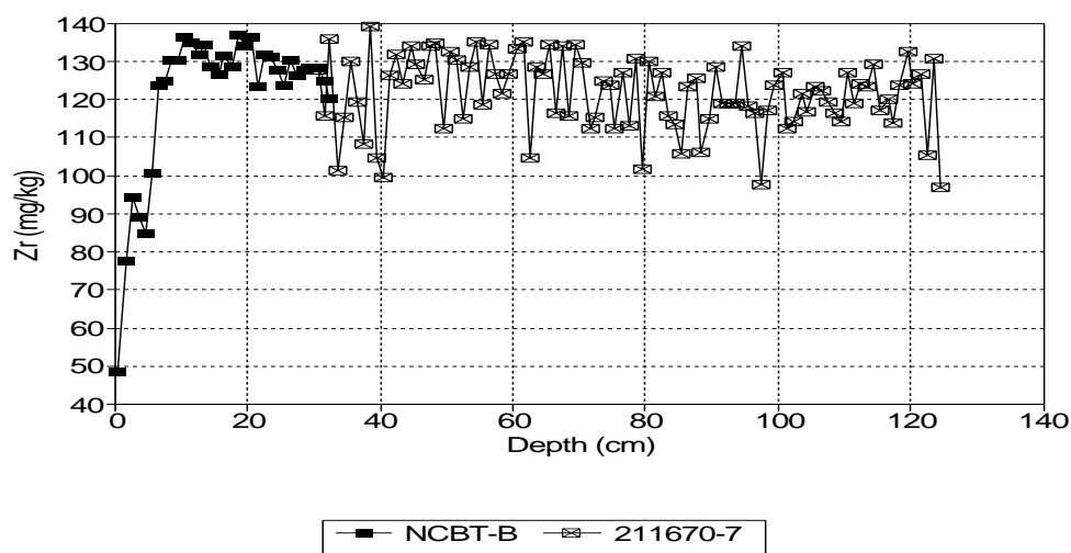
Fig. 23 Distributions of Br, Mo and Zr in the upper 1.2 m of the North Central Basin deep coring site constructed by using the short core NCBT-B and the upper 1 m of core 211670-7.
