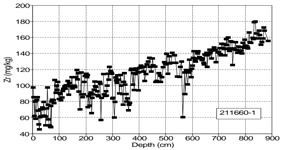
Fig. 20 Distributions of K, Rb and Zr along the long piston core 211660-1 of the Gotland Basin based on sediment material from cubes that have been used for the paleomagnetic measurements.
