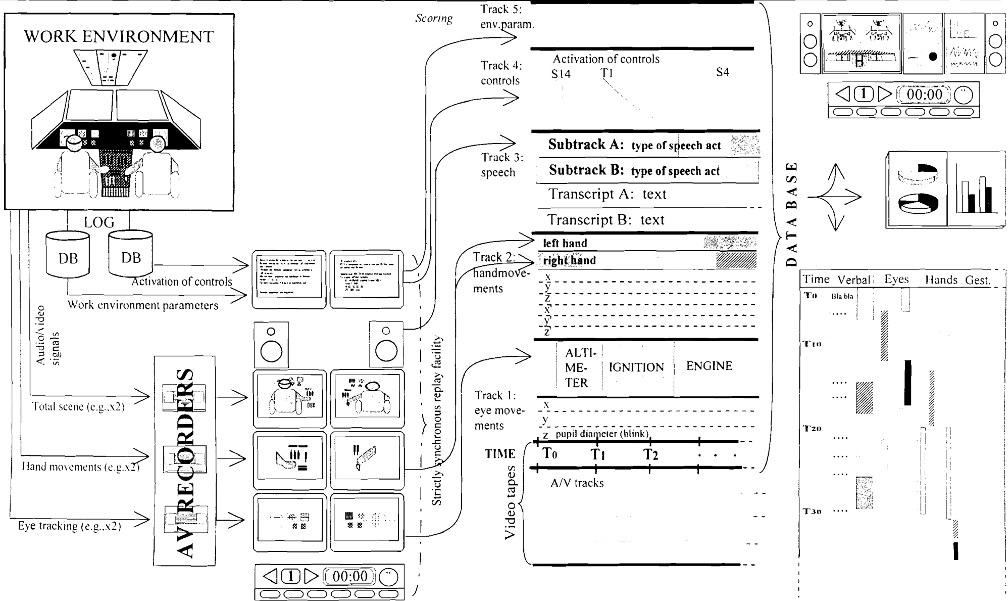
Figure 2: An overview of how the four phases during recording and analysis of operator behaviour are supported by the MULTIMO System
